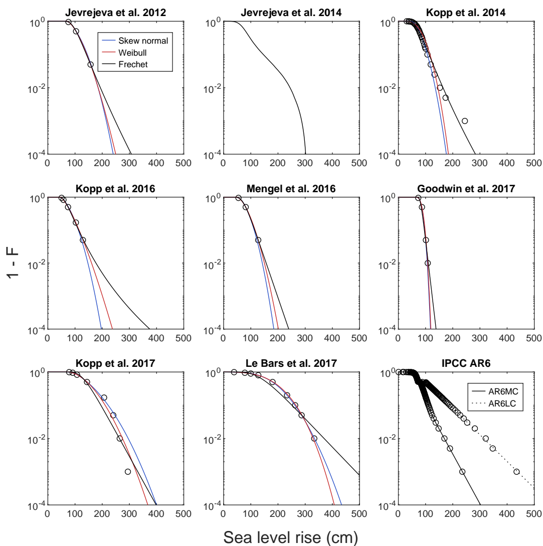
Figure A1. Members of the projection ensemble under the high emission scenario. Fits for all three distribution types (Weibull, Frechet, skew normal) are shown as complementary cumulative distribution functions ( 1 - F ). No fits were applied to Jevrejeva et al. (2014) and IPCC AR6 (Fox-Kemper et al., 2021). AR6MC and AR6LC are the medium and low confidence projections of IPCC AR6, respectively.
