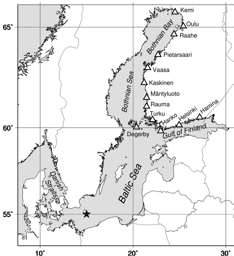
Figure 1. Map of the Baltic Sea region, with Finnish tide gauges marked with triangles. The star denotes the point ( 55^{\circ}\text{N} , 15^{\circ}\text{E} ) with the best correlation between the zonal geostrophic wind speed component and mean sea level on the Finnish coast.
