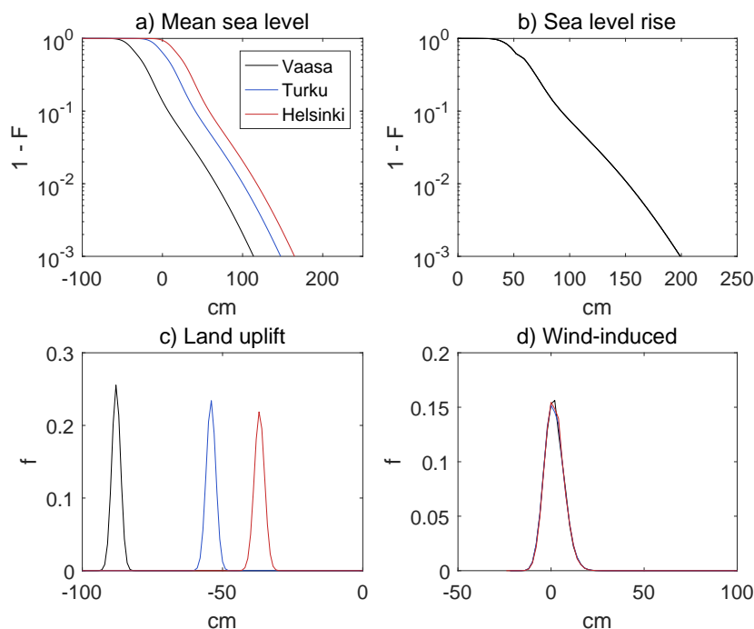
Figure 7. Probability distributions of projected mean sea level (a) and its components (b to d) in Vaasa, Turku, and Helsinki under the medium emission scenario (RCP4.5/SSP2-4.5), 2100 relative to 1995–2014. The distributions a) and b) are complementary cumulative distribution functions ( 1 - F ), while c) and d) are probability density functions ( f ).
