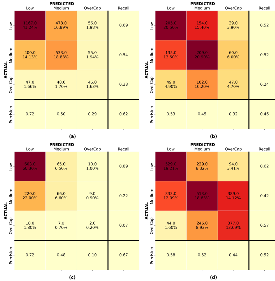
Figure 12. Confusion matrices for the random forest algorithm: (a) 4 September 2010 model tested-validated on 4 September 2010, (b) 4 September 2010 model tested on 22 February 2011, (c) 22 February 2011 model tested on 4 September 2010, (d) 22 February 2011 model tested-validated on 22 February 2011
