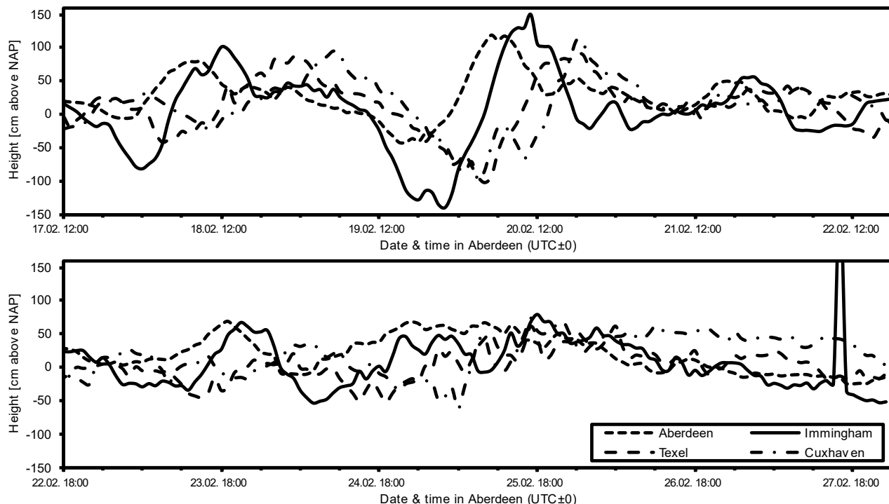
455 Figure 7: Height of the non-tidal residual (at the gauges in Aberdeen & Immingham) and the residual (at Texel & Cuxhaven) during the serial external surges from 17 to 27 February 1997. The fourth surge, starting on 22 February at 06:00 in Aberdeen does not reach the required height limit. However, if the preceding troughs are considered, this surge reaches 39 cm in Aberdeen and 48 cm in Immingham and can therefore be considered as an external surge. The spike in Immingham around 27 February 15:00 is due to uncorrected flawed data.
