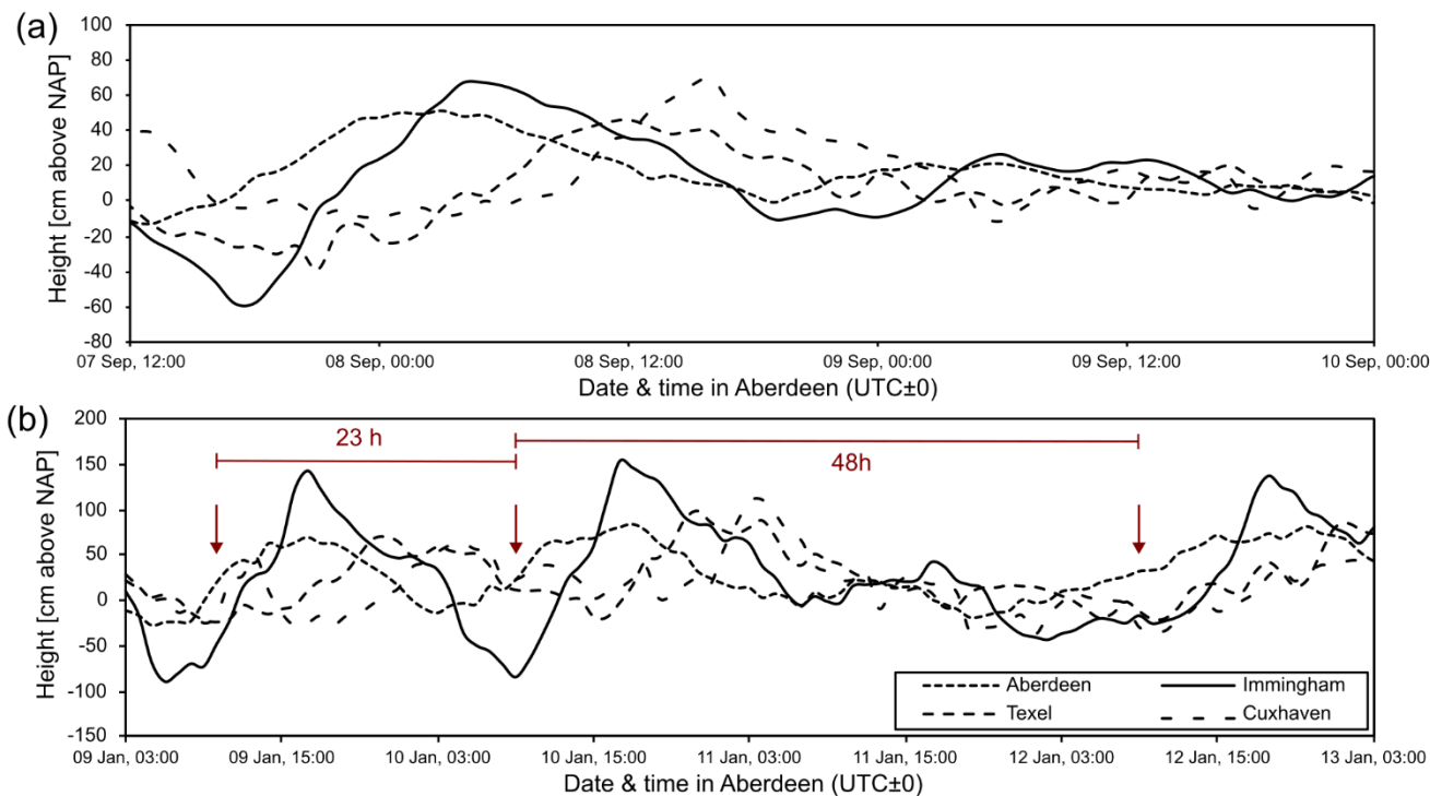
420 Figure 5: Height of the non-tidal residual (at the gauges in Aberdeen & Immingham) and the residual (at Texel & Cuxhaven) for examples of an external surge on 7 and 8 September 2000 (a) and a serial external surge on 9–13 January 2015 (b). The arrows in (b) mark the beginning of the external surges in Aberdeen (residual >20 cm) and the timing between the serial external surges is given.
