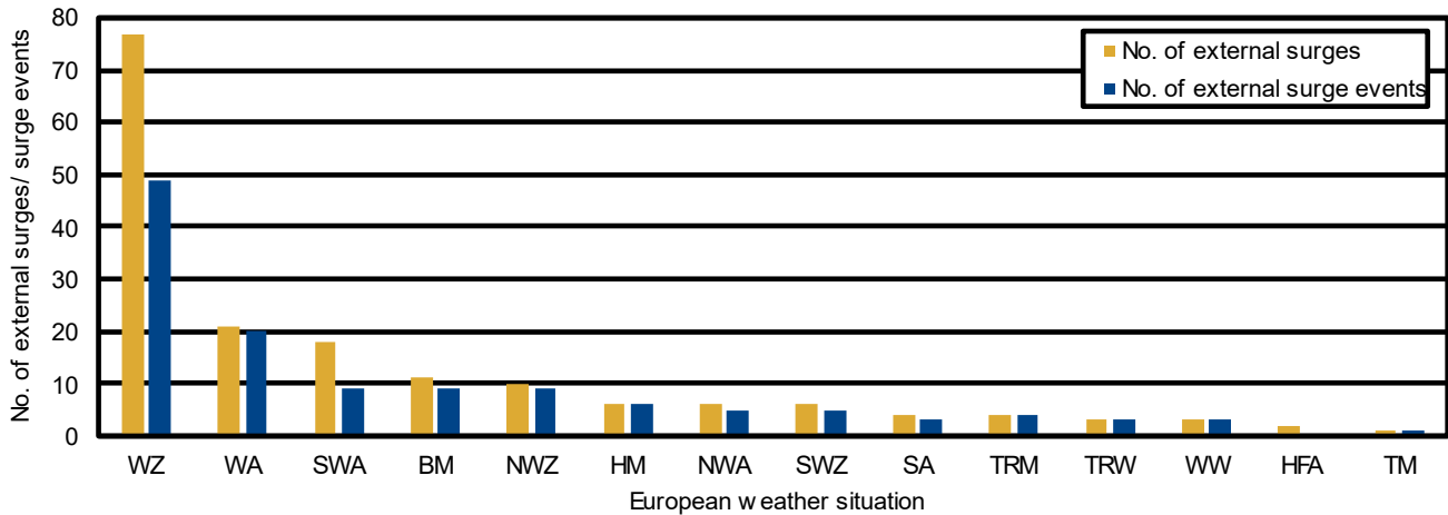
520 Figure 11: Number of external surges per European weather situation of the 1971 to 2020 external surges. Weather situations are defined by Hess and Brezowski (1977). The weather situation of an external surge is the one that is present at the date of arrival at Aberdeen. For an external surge event, the weather situation of the first or only surge in the series is used. For the weather situation HFA, no external surge event is noted, as both external surges occurred as part of a series that started during a different weather situation.
