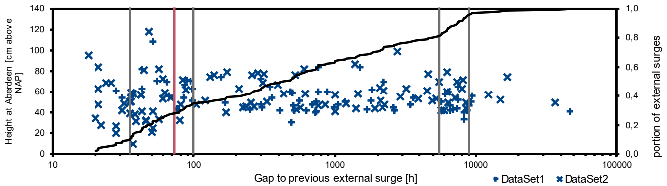
Figure 6: Height of the external surges (combined datasets) over the time gap to the previous surge and the sum line of external surges depending on the gap to the previous surge. Two areas of stronger increases can be seen (highlighted by the grey lines): between 35 and 100 h and between 5500 and 9000 h. The first shows the occurrence of serial external surges, the second is due to the lack of external surges in spring and summer, resulting in similar gaps between the last surge in winter and the first surge in autumn. The red line shows the threshold of 72 h for serial external surges.
