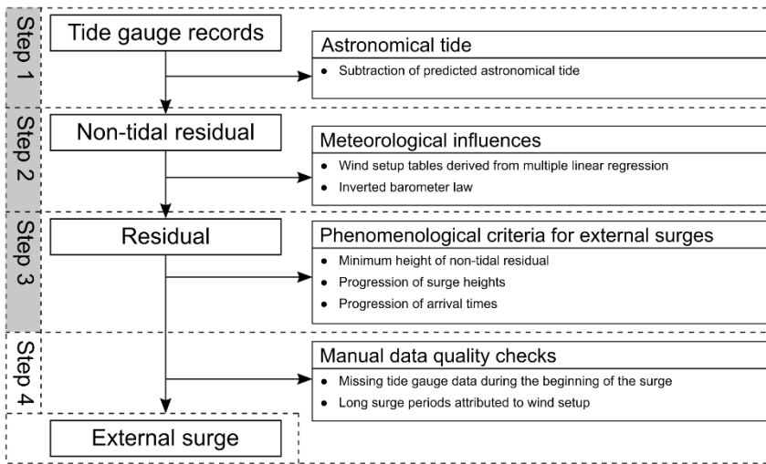
195 Figure 2: Schematic representation of the process to identify external surges. Grey backgrounds mark automated steps in the analysis.
