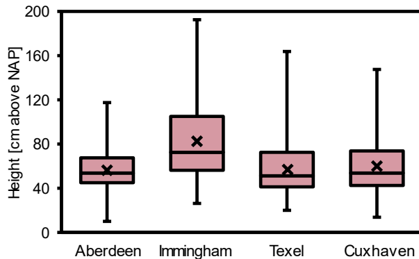
500 Figure 10: Boxplot of the heights of external surges in Aberdeen, Immingham, Texel, and Cuxhaven from 1995 to 2020. Crosses mark the mean, the boxes represent the upper and lower quartile with the horizontal line for the median. The whiskers show the minimum and maximum height.
