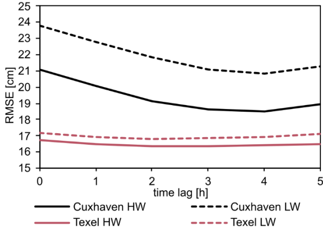
290 Figure 3: RMSE depending on the time lag between measured winds and wind setups at the tide gauges in Cuxhaven (black lines) and Texel (red lines). Solid lines mark the RMSE for high water phases, dashed lines for low water phases. The groups, based on off- and onshore wind directions are combined before determining the RMSE.
