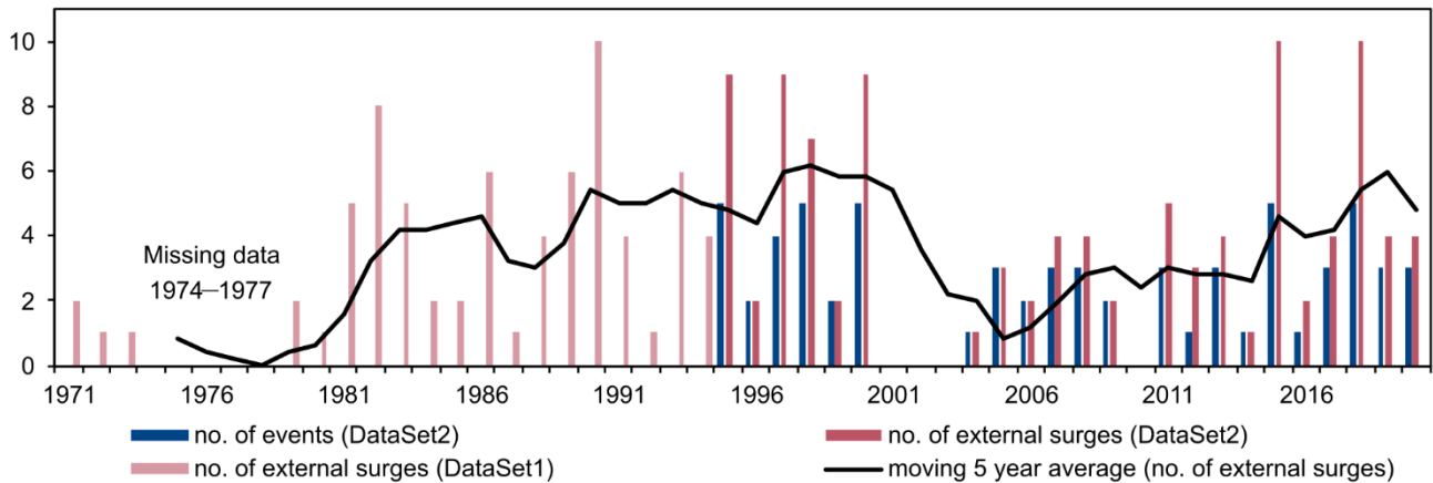
Figure 8: Number of external surges per year and rolling moving 5 year average, combination of this study and data from Gönner (2003). The 5 year average is accurate from 1983 onwards, as previous values include years with missing data. From 1995 onwards, the number of events is also shown, which counts serial external surges as a single event.
