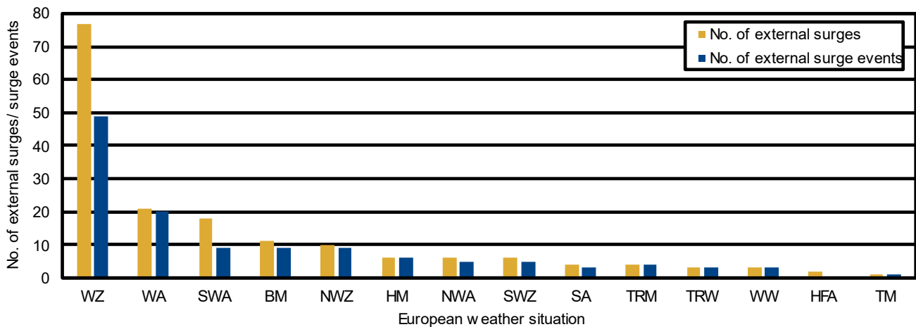
525 Figure 11: Number of external surges per European weather situation of the 1971 to 2020 external surges. Weather situations are defined by Hess and Brezowski (1977). The weather situation of an external surge is the one that is present at the date of arrival at Aberdeen. For an external surge event, the weather situation of the first or only surge in the series is used. For the weather situation
