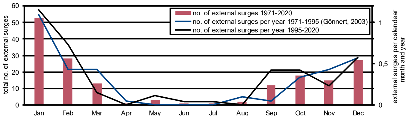
Figure 9: number of external surges per calendar month, the data from Gönner (2003) contains a data gap from 1974 to 1977, which does not influence the monthly distribution, as whole years are missing.
