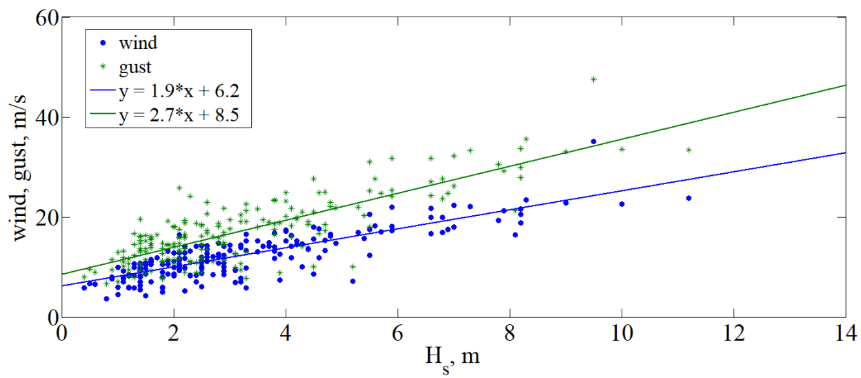
430 Figure 14: Dependence of wind speed and gusts versus significant wave heights for deep and shallow freak wave events.
