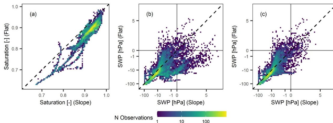
295 Figure 5: Hourly sloped vs. flat profile mean saturation (a) and profile mean SWP for the entire monitoring period (b) and 300 disregarding the period 2020-10-01 – 2021-07-20 (c). The colour indicates the number of measurement points (scaled logarithmically).
