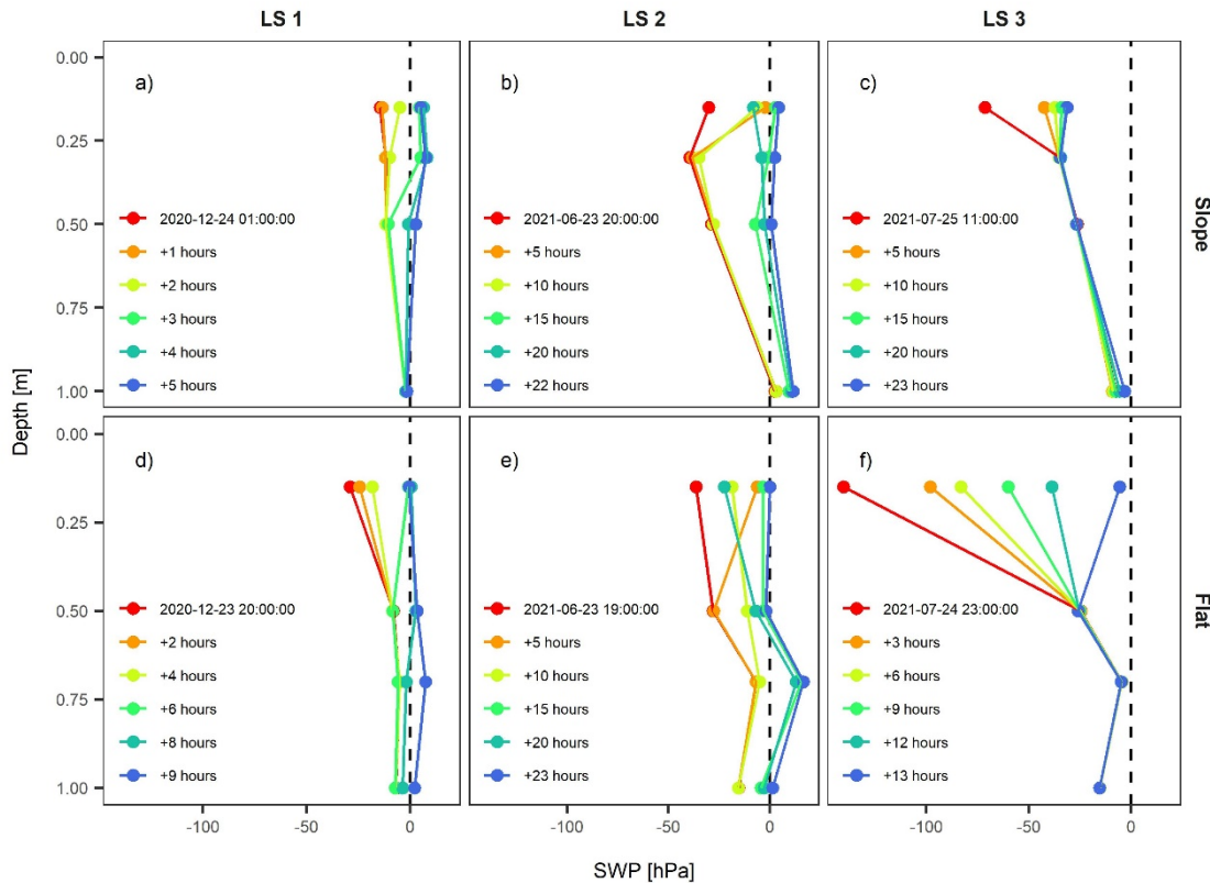
Figure 10: Depth profiles of soil water potential at the sloped (a-c) and flat site (d-f) during three landslide triggering infiltration events (LS1, LS2, LS3). The first timestep corresponds to the onset of the respective infiltration event. LS1 and LS2 show relatively high antecedent SWP values throughout the profiles and infiltration to large depths, whereas the surface layers at LS3 were relatively dry and infiltration concentrated to the surface layer.
