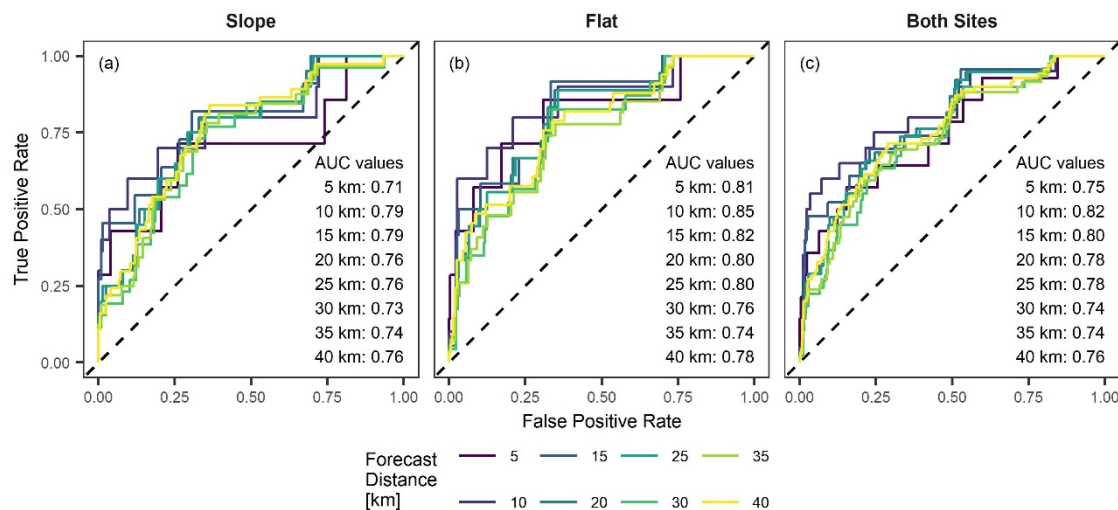
390 Figure 9: ROC curves and AUC values at the sloped (a) and flat site (b), as well as at both sites combined (c). Landslide predictions are based on a logistic regression model that predicts landslide probability based on antecedent saturation and saturation change and which was fitted to 35 sites in Switzerland over the time period 2008–2018. The colours correspond to different forecast distances.
