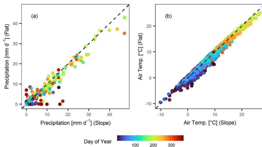
Figure 2: Sloped vs. flat daily precipitation sums (a) and daily mean air temperature (b). The point colour indicates the day of the year. In (a), only days with liquid precipitation are shown (not snowfall) because the rain gauge was heated at the sloped site only.
