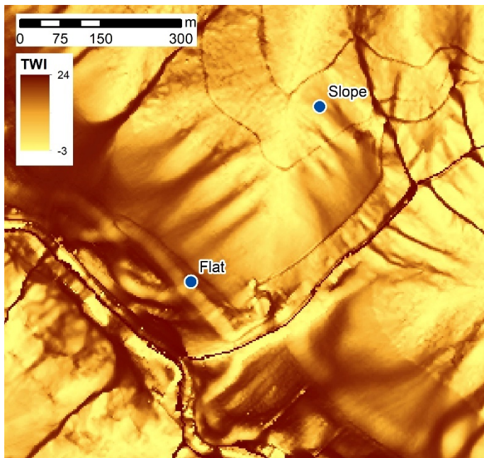
460 Figure 11: Topographic wetness index (TWI) at the study sites according to Beven and Kirkby (1979). The extract corresponds to the extent in Figure 1b.
