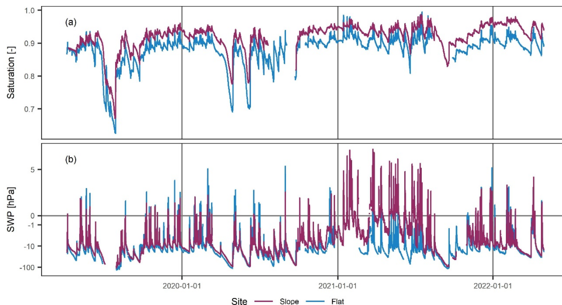
Figure 4: Hourly profile mean saturation (a) and SWP (b) over the entire study period for the flat and the sloped site.
