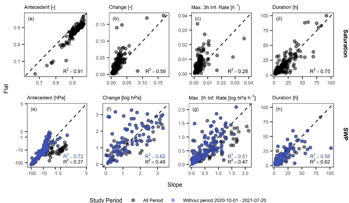
330 Figure 6: The infiltration event properties antecedent wetness, wetness increase, maximum 3 hours infiltration rate and event duration for saturation (a-d) and SWP (e-h) showing the slope vs. flat site. The blue points and R^2 values in (e-h) disregard the period 2020-10-01 – 2021-07-20.
