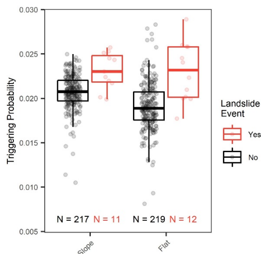
Figure 8: Boxplots showing the triggering probability distribution of infiltration events without (black) and with landslides (red) applied to the sloped and flat site separately, for a landslide forecast model based on the antecedent saturation and saturation change event properties and the 15 km forecast distance. The number of infiltration events is indicated at the bottom.
