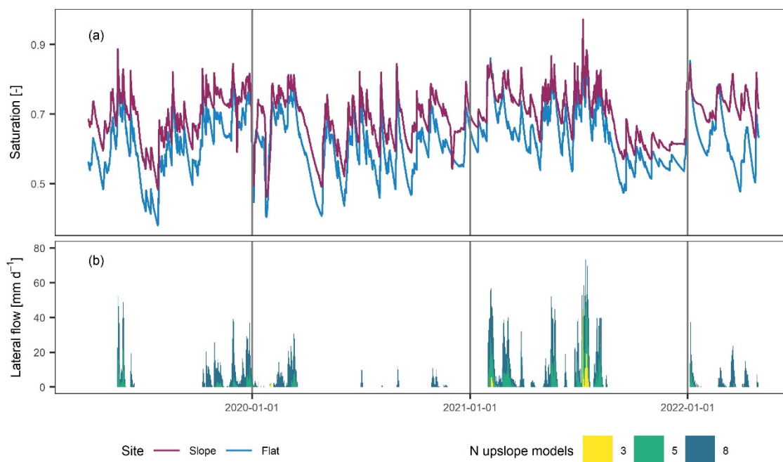
480 Figure 12: Simulated soil moisture variation at the sloped and the flat location (number of upslope models defining lateral flow at sloped site was 5) (a) and simulated lateral water flow at the sloped site in the uppermost 2 m as a function of the number of upslope models (b).
