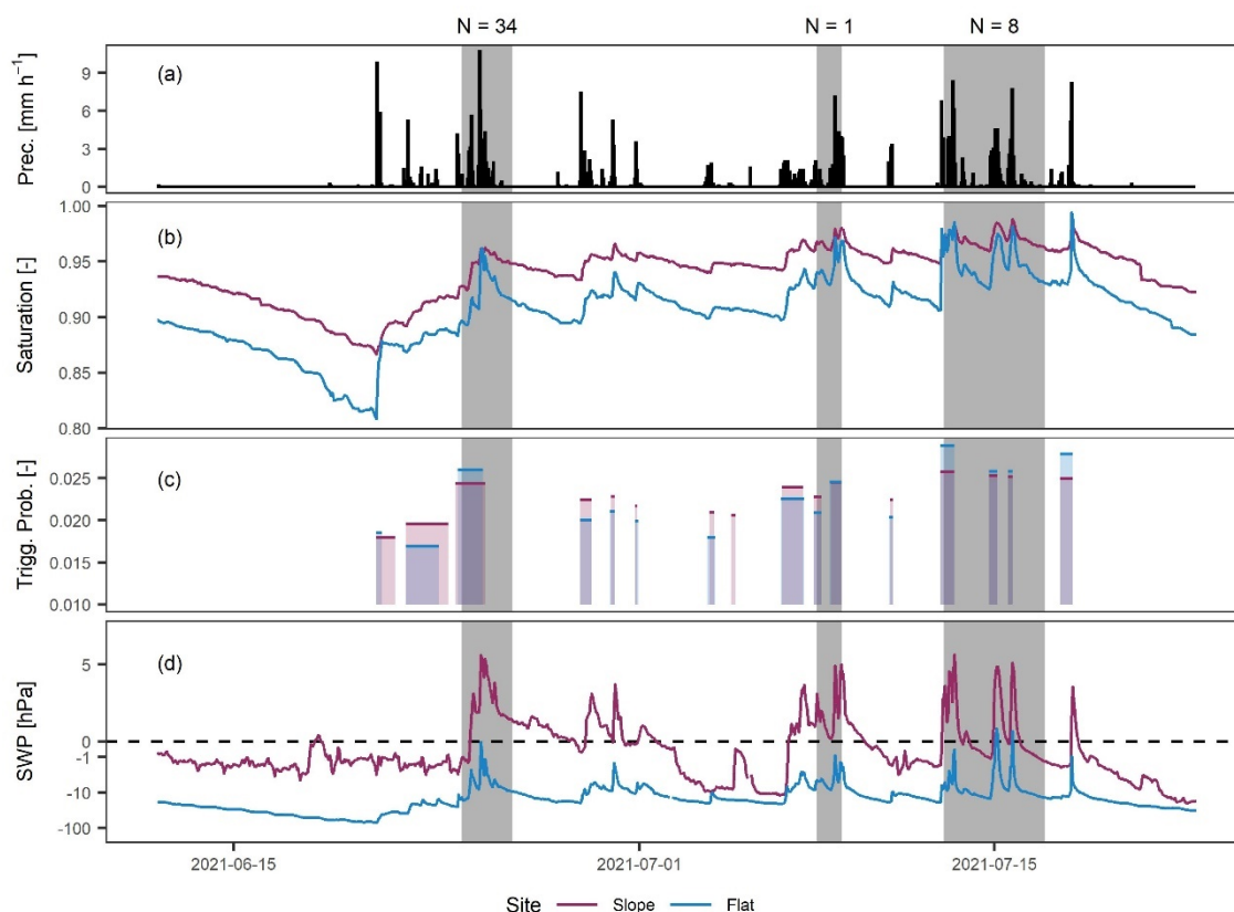
355 Figure 7: Time series extract for a period of 40 days in summer 2021 showing hourly precipitation sums at the sloped site (a), as well as the profile mean saturation (b), the triggering probabilities of the statistical landslide prediction model (c), and the profile mean SWP (d) at the two sites. The grey bars indicate consecutive days with observed landslides and the numbers (N) indicate the number of landslide events recorded within a distance of 15 km.
