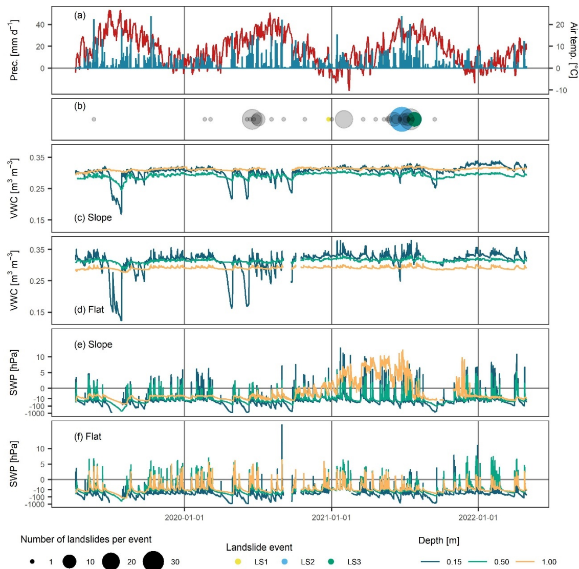
225 Figure 3: Time series of daily precipitation (blue) and air temperature variation (red) at the sloped site (a) and number of landslides per event recorded within a distance of 40 km from the monitoring sites shown as filled circles of different sizes (b). The three landslide events LS1, LS2 and LS3 (Figure 1a) are highlighted in yellow, blue, and green colours and all other events are shown in gray. Further, hourly variation of VWC at the sloped (c) and flat site (d) and hourly variation of SWP at the sloped (e) and the flat site (f) at 0.15, 0.50 and 1.00 m depth
