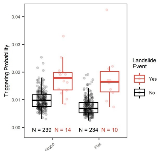
490 Figure 13: Boxplots showing the triggering probability distribution of infiltration events without (black) and with landslides (red) applied to the sloped and flat site separately, based on simulated soil moisture (number of upslope models defining lateral flow at sloped site was 5). The number of infiltration events is indicated at the bottom.
