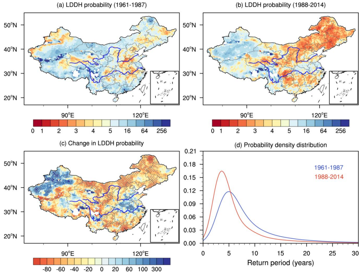
255 Figure 4: Return periods (years) of compound long-duration dry and hot events for (a) 1961-1987 and (b) 1988-2014. (c) Percentage changes (%) across China for 1988-2014 relative to 1961-1987. Stippling indicates locations with significant changes at the 90% confidence interval. (d) Probability density functions based on all grid points for the two periods.
