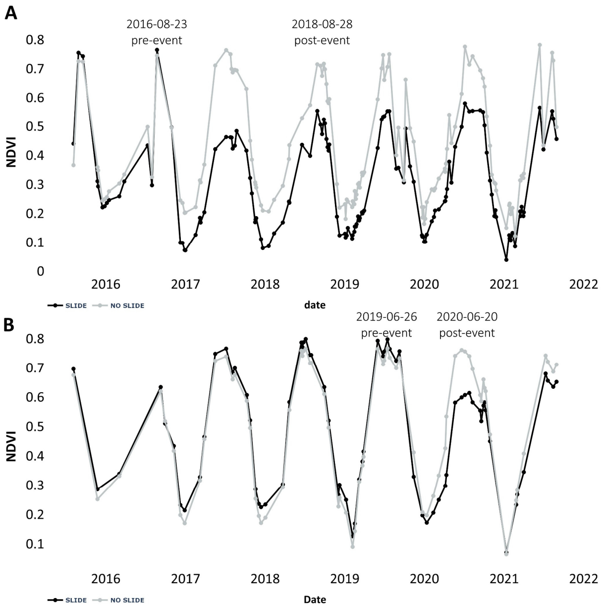
620 Figure 16. NDVI Time series based on Sentinel-2 data and processed with GEE: the 'Slides' black lines are the averaged time series of the selected ML; the 'no slides' grey lines are the time series of the surrounding unaffected areas. A) 2016 Arrocia-Tanarello case study; B) 2019 Gavi case study.
