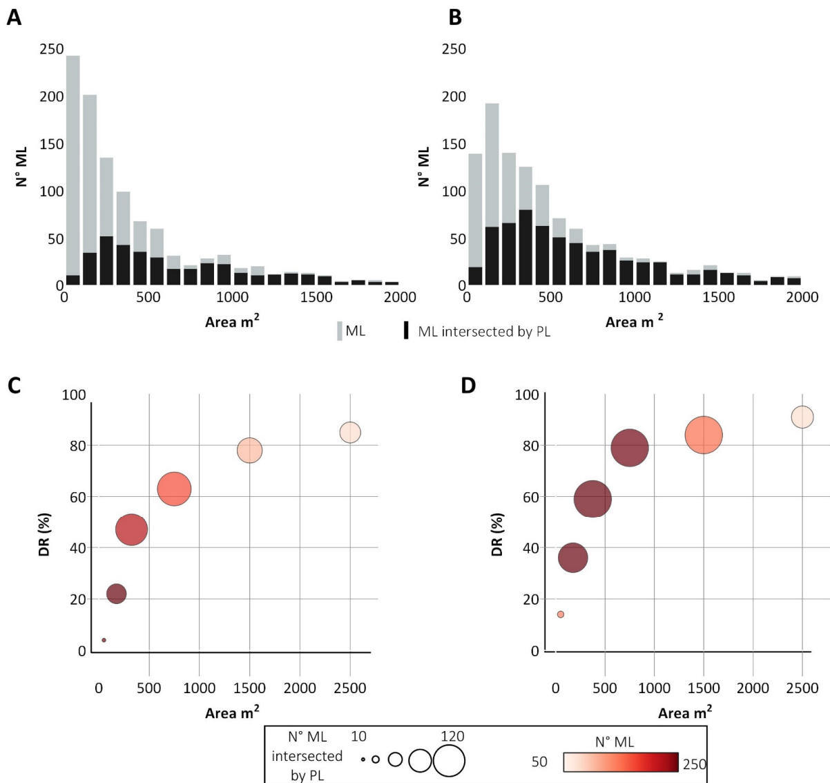
535 Figure 13 Histogram of ML area distribution for Tanarello and Arroscia valleys (A) and Gavi (B) study areas, the grey bars represent the entire ML inventory while the black one represents the ML intersected by a PL. Detection rate (DR) for each area class for Tanarello and Arroscia valleys (C) and Gavi area (D) case study. The size of the circle is correlated with the number of detected ML; the colour scale represents the total number of ML for each class.
