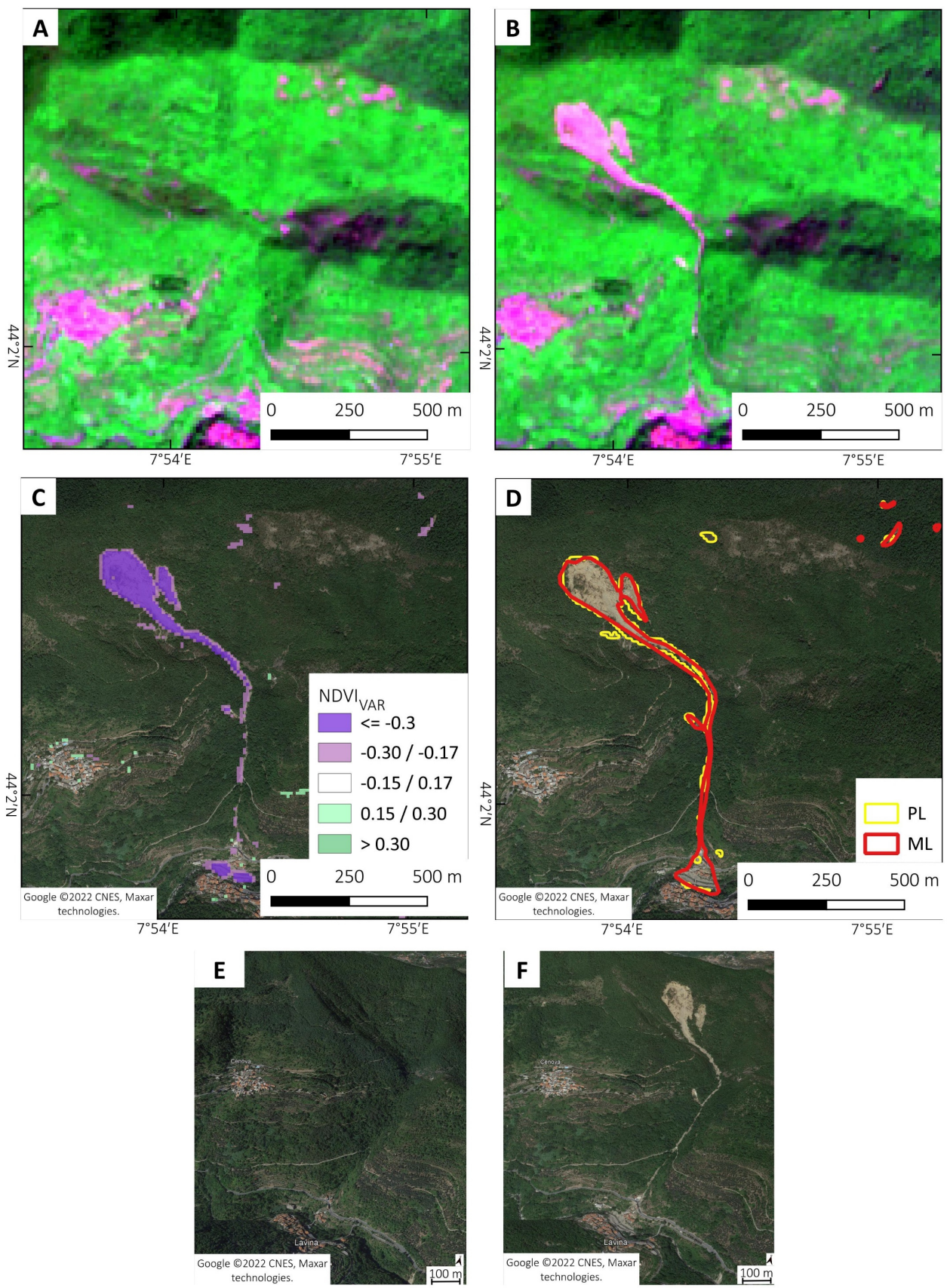
355 Figure 5. Example of shallow landslides detection methodology for Tanarello and Arroscia valleys case study: A) Sentinel-2 pre-event images (RED-NIR-BLUE) acquired on 2016-08-23; B) A) Sentinel-2 post-event images (RED-NIR-BLUE) acquired on 2018-08-28; C) NDVI var map PL inventory; D) ML and PL inventory overlapped to post-event high-resolution image (Google Earth – 2017). Google Earth 3D view of pre- (E) and post- (F) events of the area affected by landslides. Maps data: Google ©2022 CNES, Maxar technologies.
