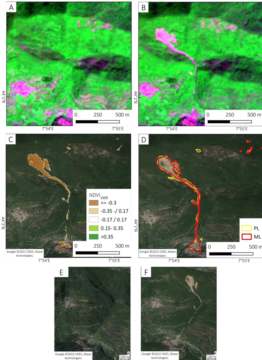
Figure 5. Example of shallow landslides detection methodology for Tanarello and Arroschia valleys case study: A) Sentinel-2 pre-event images (RED-NIR-BLUE) acquired on 2016-08-23; B) Sentinel-2 post-event images (RED-NIR-BLUE) acquired on 2018-08-28; C) NDVI var map PL inventory; D) ML and PL inventory overlapped to post-event high-resolution image (Google Earth – 2017). Google Earth 3D view of pre- (E) and post- (F) events of the area affected by landslides. Maps data: Google ©2022 CNES, Maxar technologies.
