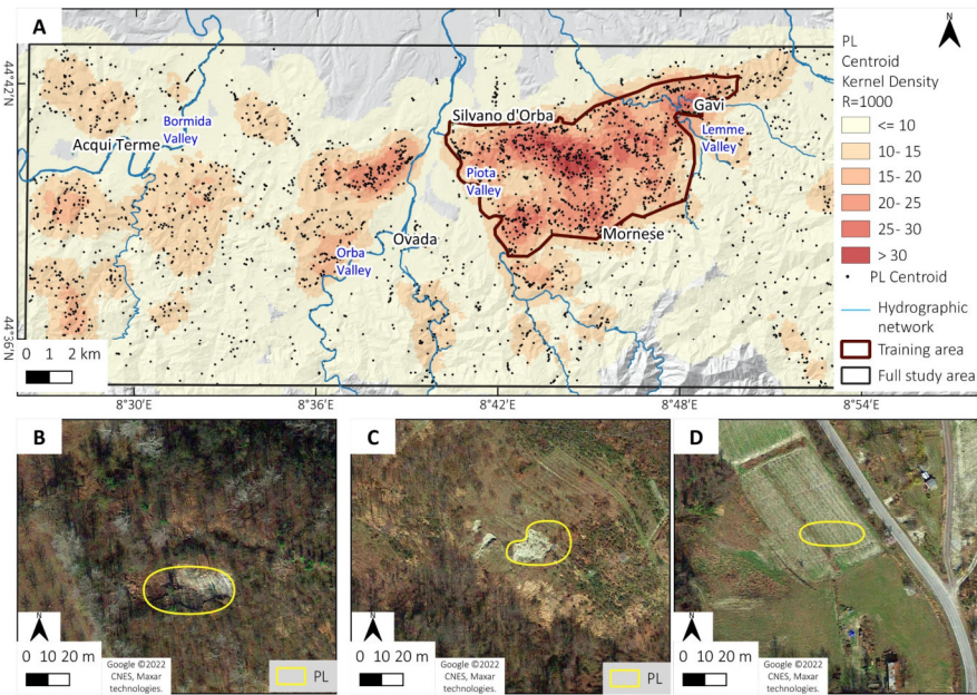
455 Figure 10. October 2019 event. A) PL centroids relative Kernel Density (R=1000) over the whole AOI. Some examples of PL: B) PL that completely overlaps a shallow landslide; C) PL that partly overlaps a shallow landslide; D) PL that corresponds to a false-positive case. Maps data: Google ©2022 CNES, Maxar technologies. The shaded relief of map A is based on the 5-m DTM of ARPA Piemonte.
