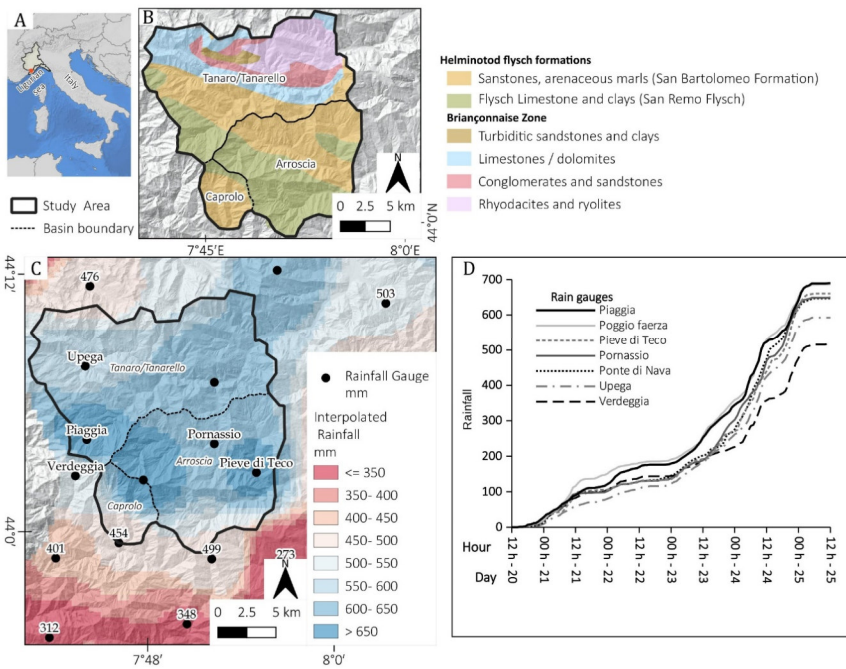
Figure 1. Arroscia/Tanarello November 2016 event. A) Location of the study area; B) Simplified geological map based on (Lanteaume et al., 1990); C) Accumulated rainfall from 20 to 25 November 2016 in the study area. D) Hourly cumulated rainfall for some rain gauge stations of study areas. (Rainfall source: ARPA Piemonte and ARPAL Liguria). Shaded reliefs of maps B and C are based on the DTM of ARPA Piemonte and Regione Liguria.
