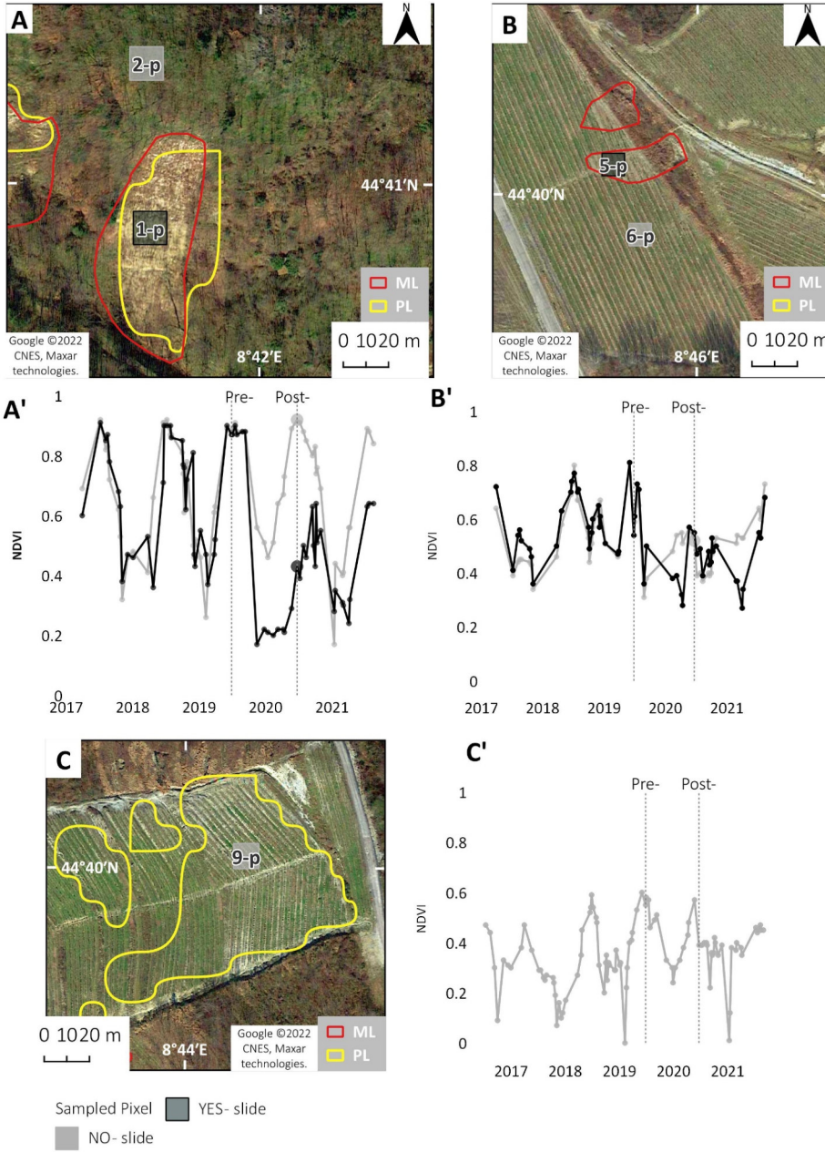
Figure 17. NDVI Time series (2017-2021) of five sample points (Landslide / No Landslide) in the area affected by the 2019 event. A and A' comparison located in a broadleaf forest (true positive); B and B' vineyard (false negative); C and C' vineyard (false positive). The Google Earth satellite image was acquired on 2021-03-16. Maps data: Google ©2022 CNES, Maxar technologies.
