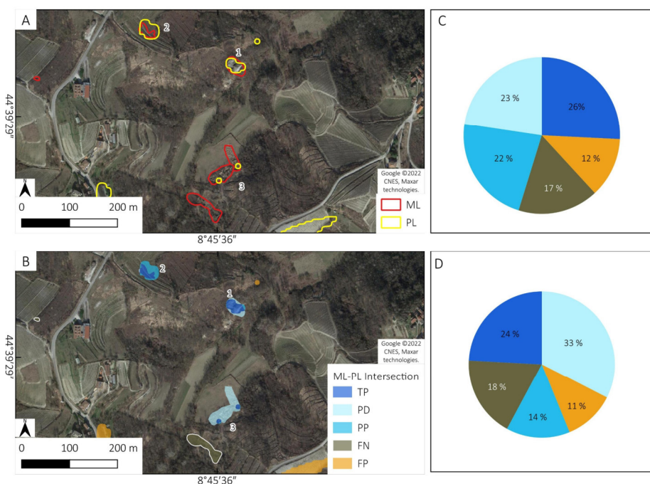
Figure 11. 2019 Gavi case study. A) PL-ML inventories intersections over a sample area. B) PL-ML intersection classified by type. Pie charts of the intersection type distribution by number (C) and area (D). Maps data: Google ©2022 CNES, Maxar technologies.
