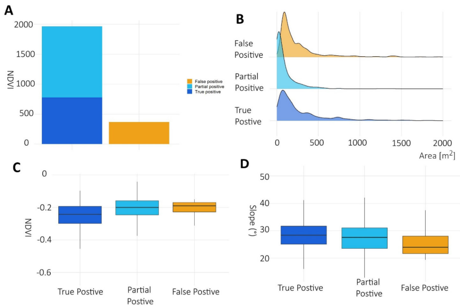
495 Figure 12. PL validation statistics for the 2019 Gavi study area: A) Bar plot showing the number of polygons of PL classified as TP, PP and FP area; B) Area frequency distribution for the polygons classified as TP, PP, and FP area C) Box plot chart of NDVI var distribution for TP, PP and FP classes ; D) Box plot chart of median slope distribution for each class of ML-PL intersection.
