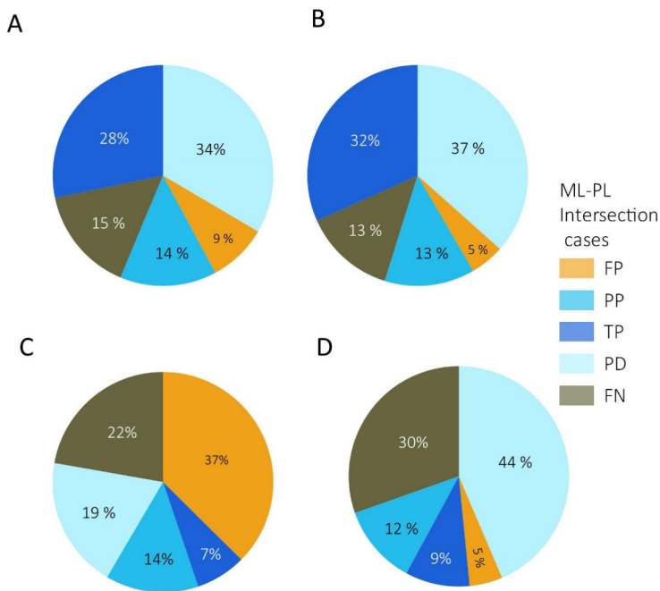
575 Figure 15. Gavi 2019 case study, PL-ML intersection distribution for the main land-use classes: A) Broad-Leaf forest; B) New-forest or shrubland; C) Vineyard; D) Cultivated land
