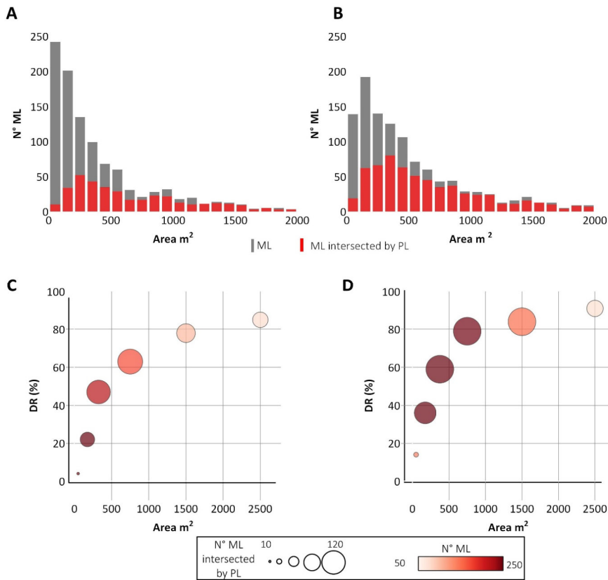
535 Figure 13 Histogram of ML area distribution for Tanarello and Arroscia valleys (A) and Gavi (B) study areas, the grey bars represent the entire ML inventory while the red one represents the ML intersected by a PL. Detection rate (DR) for each area class for Tanarello and Arroscia valleys (C) and Gavi area (D) case study. The size of the circle is correlated with the number of detected ML; the colour scale represents the total number of ML for each class.
