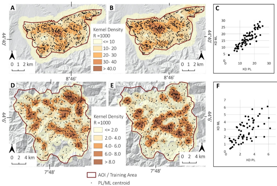
555 Figure 14. Heatmap Kernel Density for: A) Gavi PL inventory; B) Gavi ML inventory; D) Tanarello and Arroscia valleys PL inventory; E) Tanarello and Arroscia valleys ML inventory. Scatter plot of ML/PL Kernel density comparison for: C) Gavi training area; F) Tanarello and Arroscia valleys study area. Shaded relief of maps A, B, D and E are based on 5-m DTMs of ARPA Piemonte and regione Liguria.
