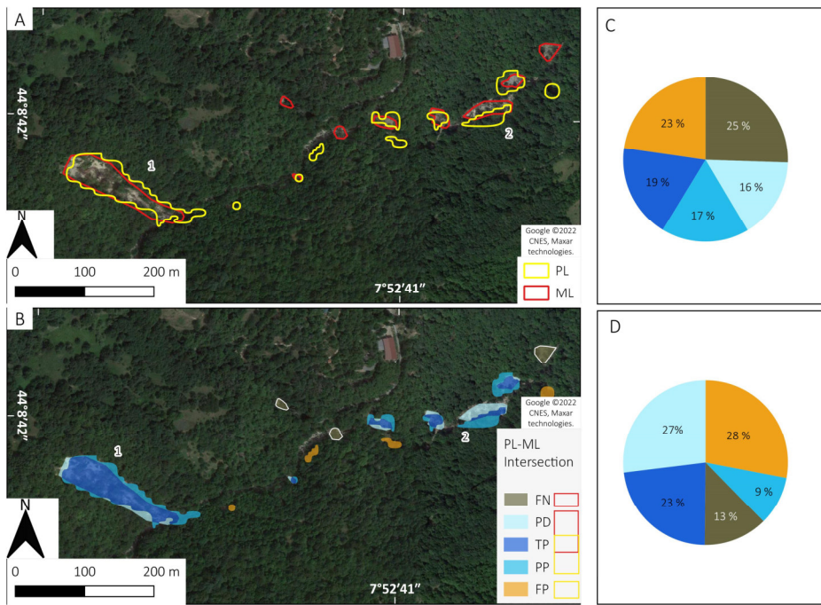
395 Figure 7. Tanarello and Arroscia valleys case study. A) PL-ML inventories intersections over a sample area. B) PL-ML intersection classified by type. Pie charts of the intersection type distribution by number (C) and area (D). Maps data: Google ©2022 CNES, Maxar technologies.
