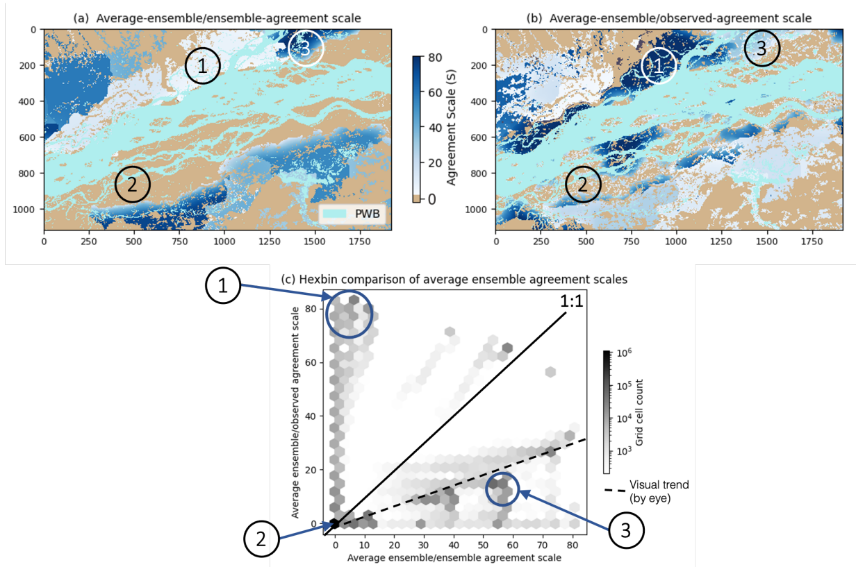
Figure 9. Brahma Putra River, Assam region, August 2017. (a) The average agreement scale map of each unique pair of forecast ensemble flood maps and (b) between each ensemble member compared against the observed SAR-derived flood map. (c) A binned histogram scatter plot compares (a) and (b) to indicate the spatial spread-skill of the forecast ensemble. Areas labelled (1, 2 and 3) are discussed in Section 4.3. For georeferencing of (a) and (b) see Figure 6. Note PWB means permanent water bodies.
