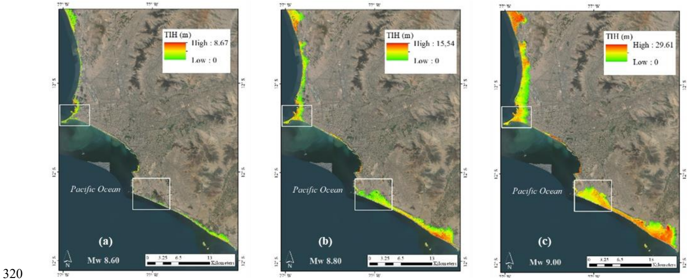
Figure 4. Expected tsunami inundation heights (TIH) in meters (m) for three out of the six considered scenarios per moment magnitude ( M_w ), namely: (a) M_w 8.6; (b) M_w 8.8; and (c) M_w 9.0. These raster products are available from Harig and Rakowsky, (2021). Two densely populated areas are depicted by white rectangles: in the north the “La Punta” (Callao) and Chorrillos in the south. Updated figure from Gómez Zapata et al., (2021f). Map data: ©Google Earth 2021.
