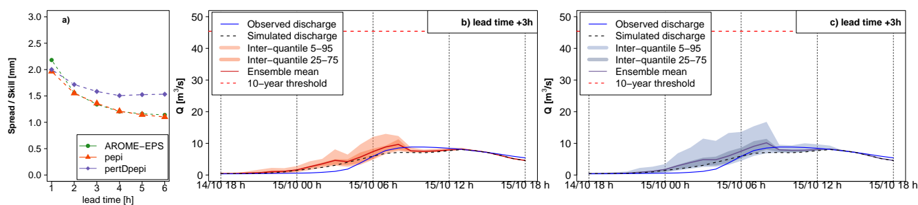
Figure 11. Detailed hydrological forecasts evaluation at outlet 1: a) spread/skill relationship, b) hydrographs of 3 hours lead time forecasts with pepi, c) hydrographs of 3 hours lead time forecasts with pertDpepi. In blue, the observed hydrograph at the gauging station.
