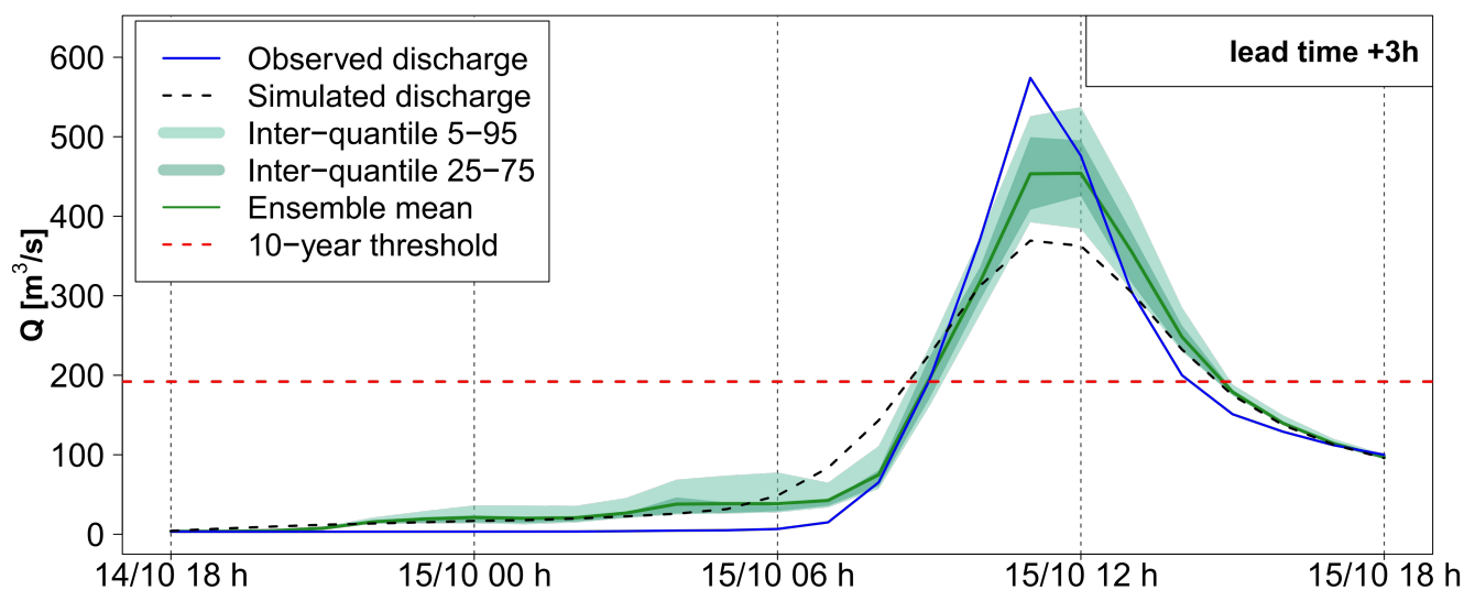
Figure B6. Detailed hydrograph for 3 hours lead time forecasts evaluation at outlet 4 for AROME-EPS. In blue, the observed discharge at the gauging station
