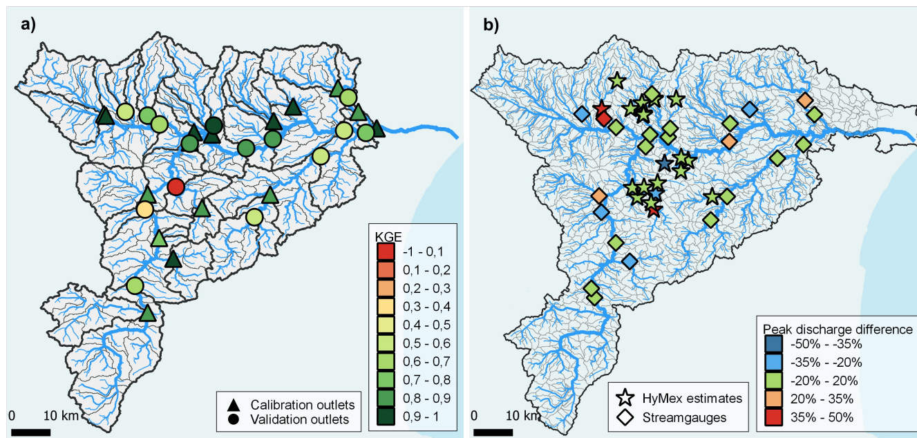
Figure 4. Calibration-validation results for the two rainfall-runoff models: a) KGE values at calibration and validation outlets (stream gauges) for the GRSDi model and the period 01/10/2008 at 0h to 15/10/2018 at 23h, b) Peak discharge difference (in %) between CINECAR simulated discharges and HyMex estimates (stars) or stream gauges (diamonds) when the model is calibrated over the Aude 2018 flood event.
