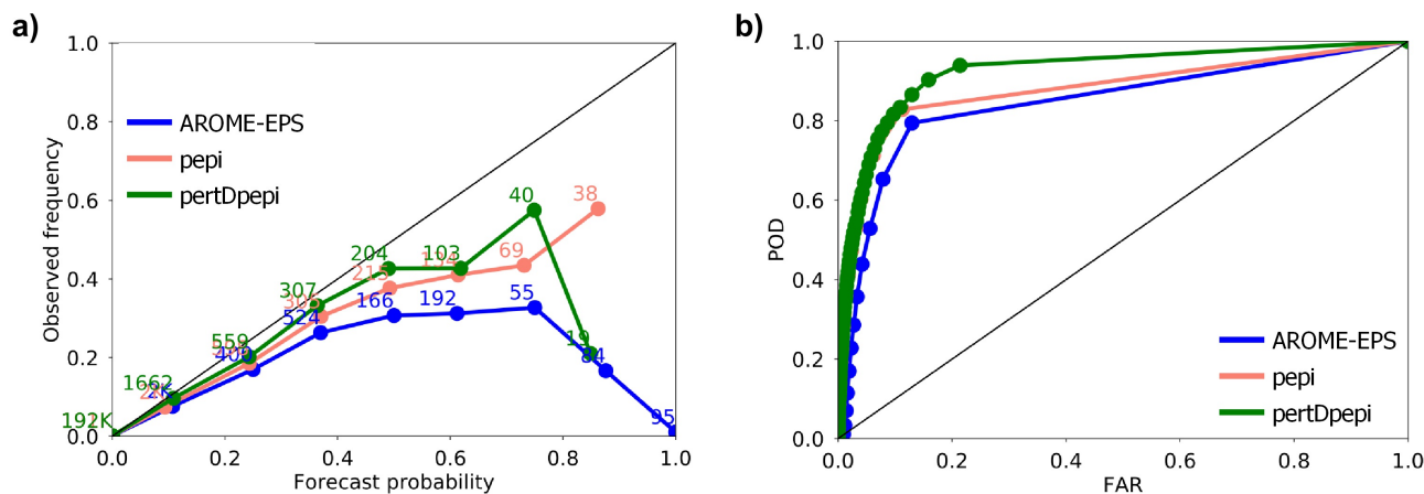
Figure 3. Evaluation of rainfall ensembles for rainfall exceeding 5 mm/h and lead times from 2h to 6h: a) Reliability diagram, b) ROC curves (POD, Probability of detection and FAR, false alarm rate).
