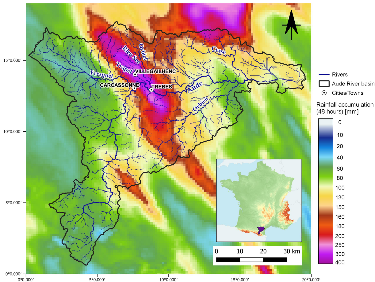
Figure 2. The Aude River basin, its river network, and the observed rainfall accumulation during the October 2018 flood (14 October 2018 00:00 to 15 October 2018 23:00).
