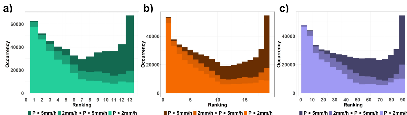
Figure 7. Rank diagrams of the three ensemble products for lead time one-hour : a) AROME-EPS, b) pepi, c) pertDpepi.
