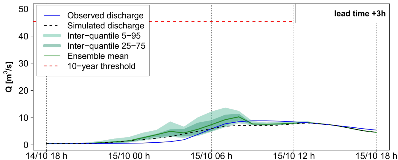
Figure B1. Detailed hydrological 3 hours lead time forecasts evaluation at outlet 4 for AROME-EPS. In blue, the observed discharge at the gauging station
