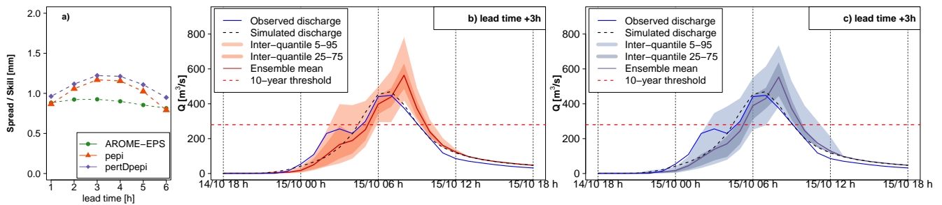
Figure 15. Detailed hydrological forecasts evaluation at outlet 5: a) spread/skill relationship, b) hydrographs of 3 hours lead time forecasts with pepi, c) hydrographs of 3 hours lead time forecasts with pertDpepi. In blue, the observed hydrograph at the gauging station.
