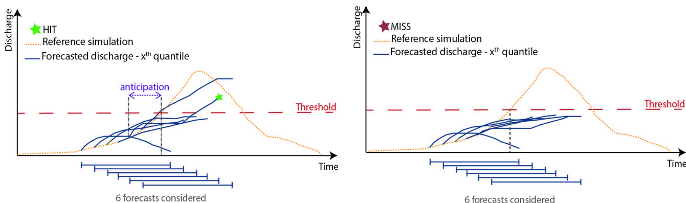
Figure A1. Illustration of the discharge threshold exceedance detection method - cases of a hit (left) and a miss (right)
