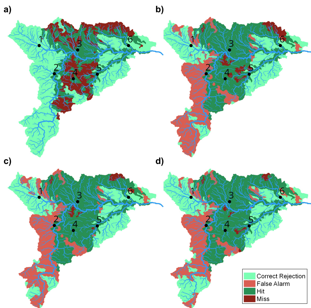
Figure 9. Maps of anticipation (0-6h) of the 10-year return period discharge threshold : a) RF0 scenario, b) AROME-EPS ensemble (75% percentile), c) pepi ensemble (75% percentile), d) pertDpepi ensemble (75% percentile). Hits are displayed for anticipation times exceeding 15 min. Black dots represent the outlets where a detailed analysis of the forecasts is proposed in Section 4.3.
