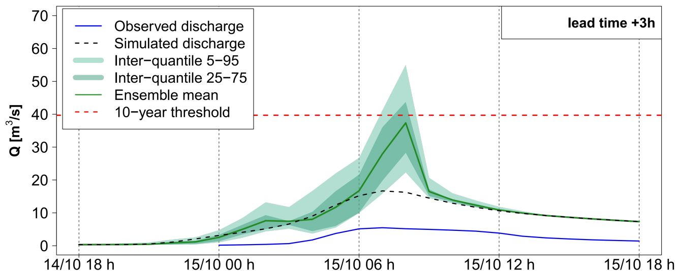
Figure B2. Detailed hydrograph for 3 hours lead time forecasts evaluation at outlet 4 for AROME-EPS. In blue, the observed discharge at the gauging station
