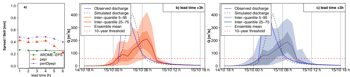
Figure 14. Detailed hydrological forecasts evaluation at outlet 4: a) spread/skill relationship, b) hydrographs of 3 hours lead time forecasts with pepi, c) hydrographs of 3 hours lead time forecasts with pertDpepi. In blue, the observed hydrograph at the gauging station.
