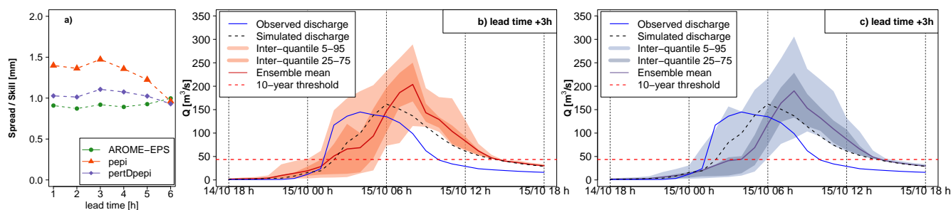
Figure 13. Detailed hydrological forecasts evaluation at outlet 3: a) spread/skill relationship, b) hydrographs of 3 hours lead time forecasts with pepi, c) hydrographs of 3 hours lead time forecasts with pertDpepi. In blue, the observed hydrograph at the gauging station.
