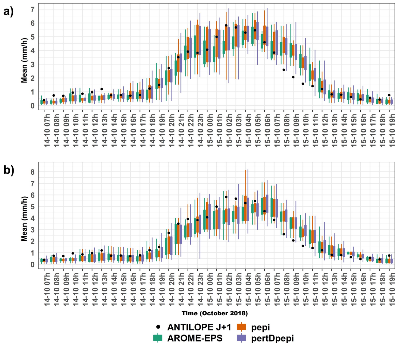
Figure 5. Temporal evolution of observed hourly rainfall rates (black dots), and a) 1 hour and b) 6 hours lead time ensemble forecasts (boxplots), during the October 2018 flood event. Rainfall rates are averaged over the Aude River basin. The boxplots correspond to AROME-EPS (green), pepi (orange) and pertDpepi (purple). Whiskers reflect the min-max range and boxes the inter-percentile (25%-75%) for the forecasts.
