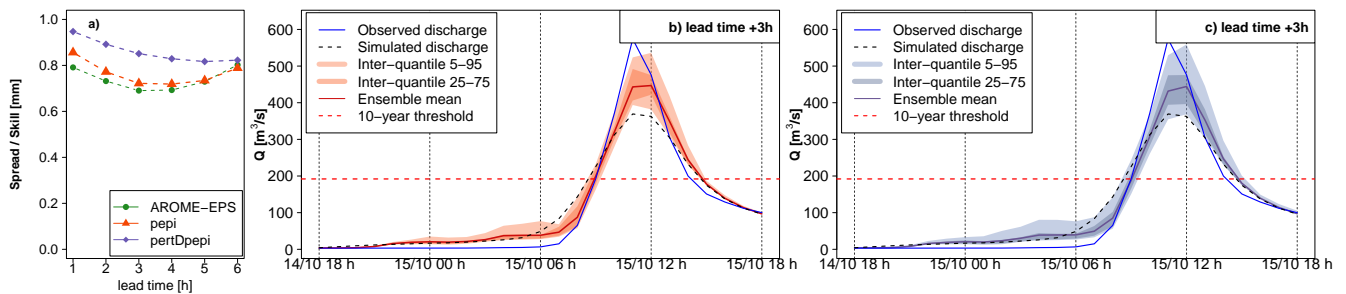
Figure 16. Detailed hydrological forecasts evaluation at outlet 6: a) spread/skill relationship, b) hydrographs of 3 hours lead time forecasts with pepi, c) hydrographs of 3 hours lead time forecasts with pertDpepi. In blue, the observed hydrograph at the gauging station.
