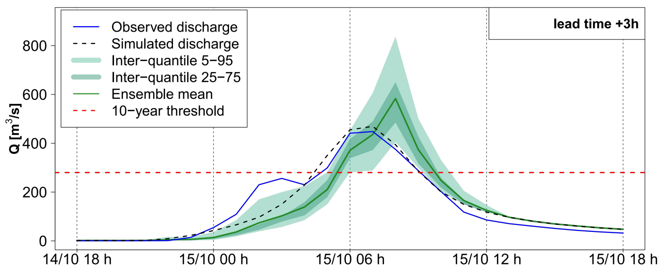
Figure B5. Detailed hydrograph for 3 hours lead time forecasts evaluation at outlet 4 for AROME-EPS. In blue, the observed discharge at the gauging station
