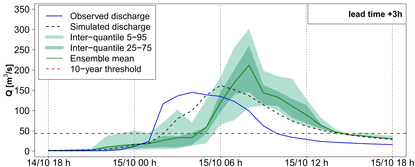
Figure B3. Detailed hydrograph for 3 hours lead time forecasts evaluation at outlet 4 for AROME-EPS. In blue, the observed discharge at the gauging station
