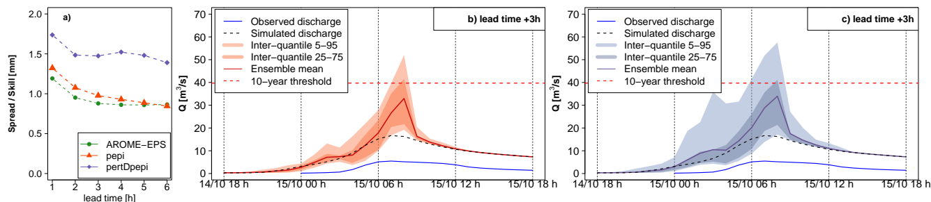
Figure 12. Detailed hydrological forecasts evaluation at outlet 2: a) spread/skill relationship, b) hydrographs of 3 hours lead time forecasts with pepi, c) hydrographs of 3 hours lead time forecasts with pertDpepi. In blue, the observed hydrograph at the gauging stations.
