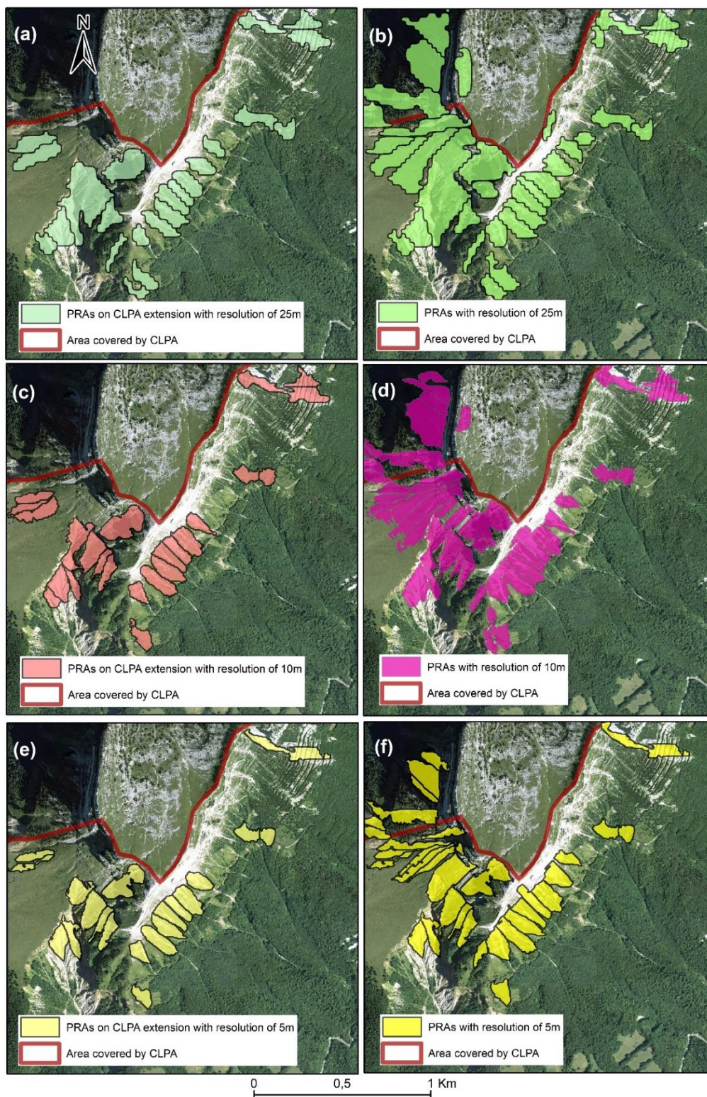
525 Figure 12 : Combined effect of DEM resolution on the selection of the validation sample (left) and PRA detection (right), Chartreuse/Dent de Crolles study area. For the PRA detection and the determination of the validation sample, DEM resolution varies, all other factors are set to their default values (Figures 3-4), and forest cover data is from DB forest IGN. Aerial photograph ©IGN 2012. Left, the absence of CLPA in the upper left corner is clearly visible, and CLPA extensions” refer to avalanche extents from the French avalanche cadastre.
