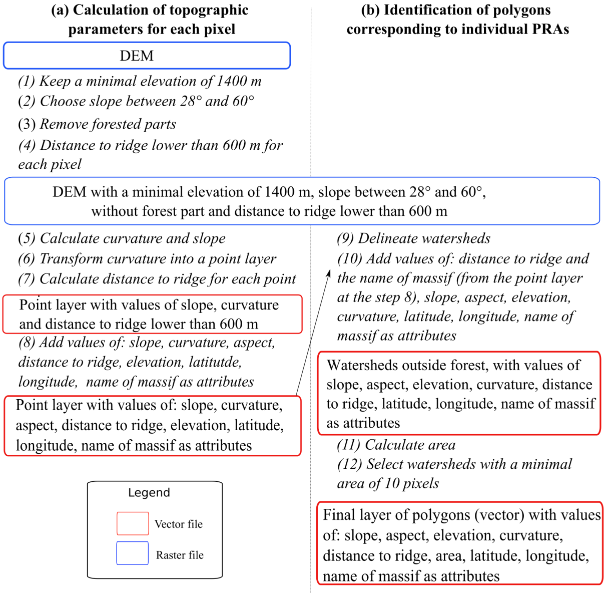
Figure 3: The 12 steps of the proposed PRA detection method. Calculations at (a) the pixel scale, (b) at the scale of identified polygons.
