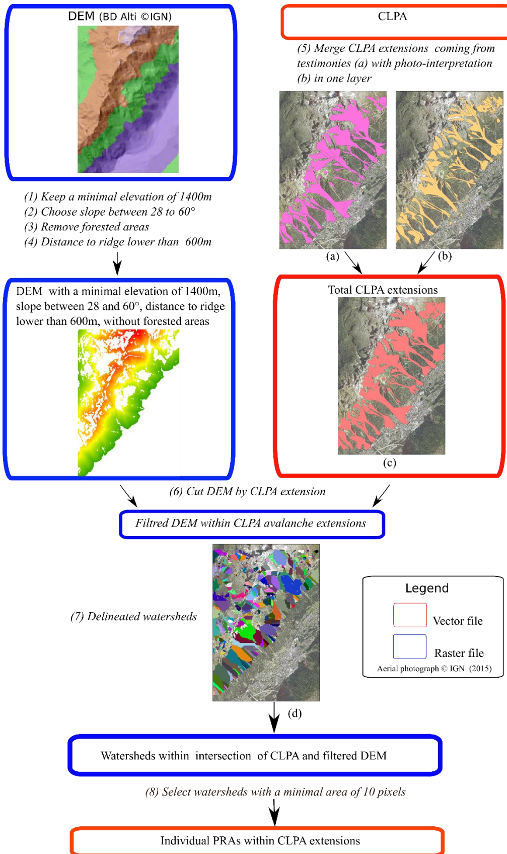
Figure 4: The French avalanche cadaster (CLPA) and the processing steps used to identify individual PRAs within CLPA avalanche extents (“avalanche extensions”) as a validation sample for the proposed PRAs detection method. (a) CLPA avalanche extents coming from testimonies, (b) CLPA avalanche extents coming from photo-interpretation, (c) Union of CLPA avalanche extents, (d) Delineation of individual PRAs within CLPA avalanche extents. Aerial photograph ©IGN 2015.
