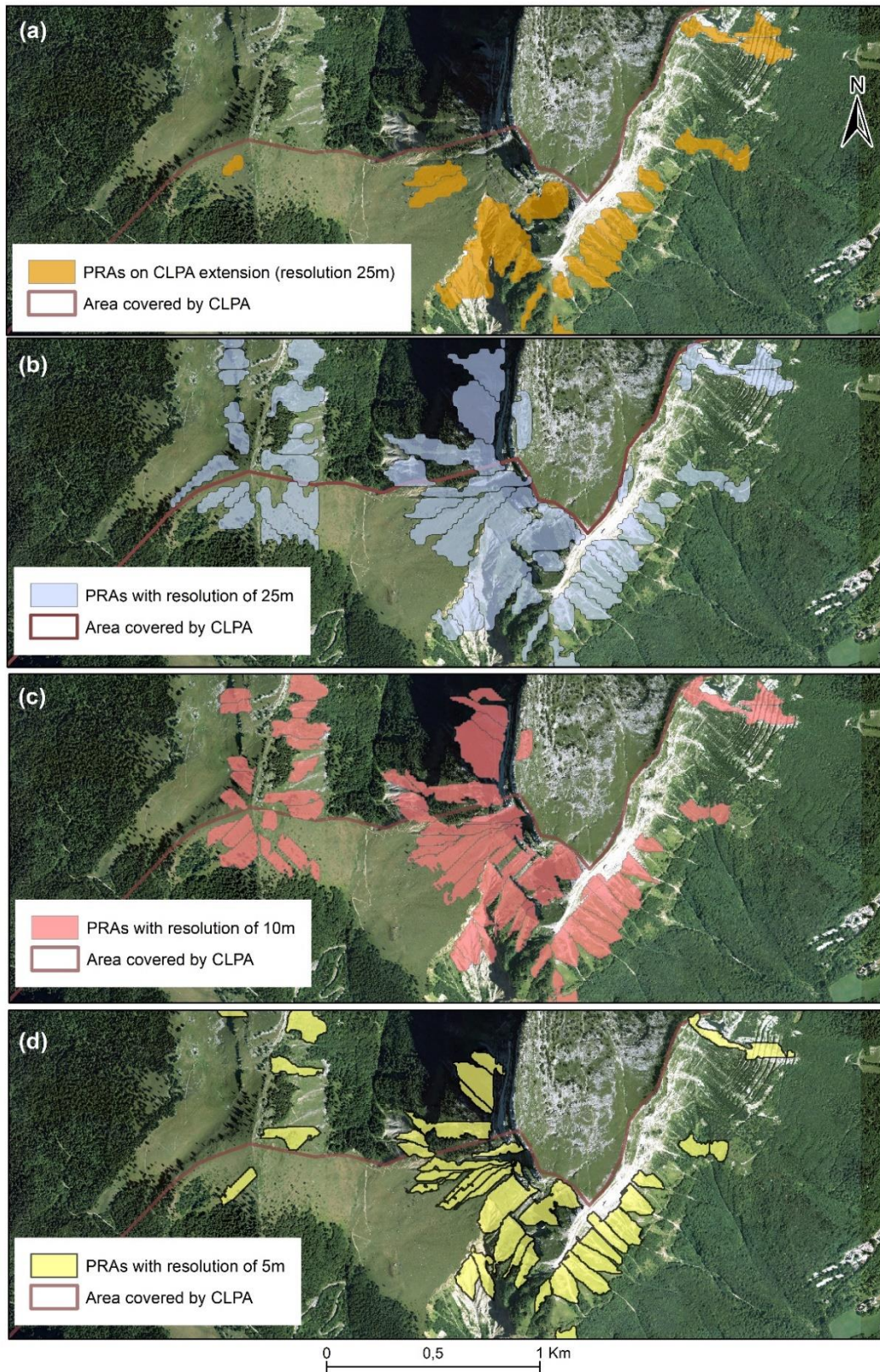
Figure 11: Effect of DEM resolution on PRA detection, Chartreuse/Dent de Crolles study area. Aerial photograph ©IGN 2012. a) For the determination of the validation sample, all factors and the DEM resolution are set to their default values (Figure 4) and forest cover data is from DB forest IGN; the absence of CLPA in the upper left corner is clearly visible. b-d) For the PRA detection, DEM resolution varies, other factors are set to their default values (Figure 3) and forest cover data is from DB forest IGN. In a), CLPA extensions” refer to avalanche extents from the French avalanche cadastre.
