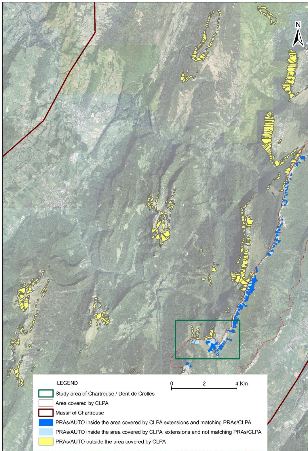
Figure 6 : Result of the proposed PRA detection method for the entire Chartreuse massif. For the PRA detection and the determination of the validation sample, all factors and the DEM resolution are set to their default values (Figures 3-4), and forest cover data is from DB forest IGN. “CLPA extensions” refer to avalanche extents from the French avalanche cadastre. Aerial photograph ©IGN 2012.
