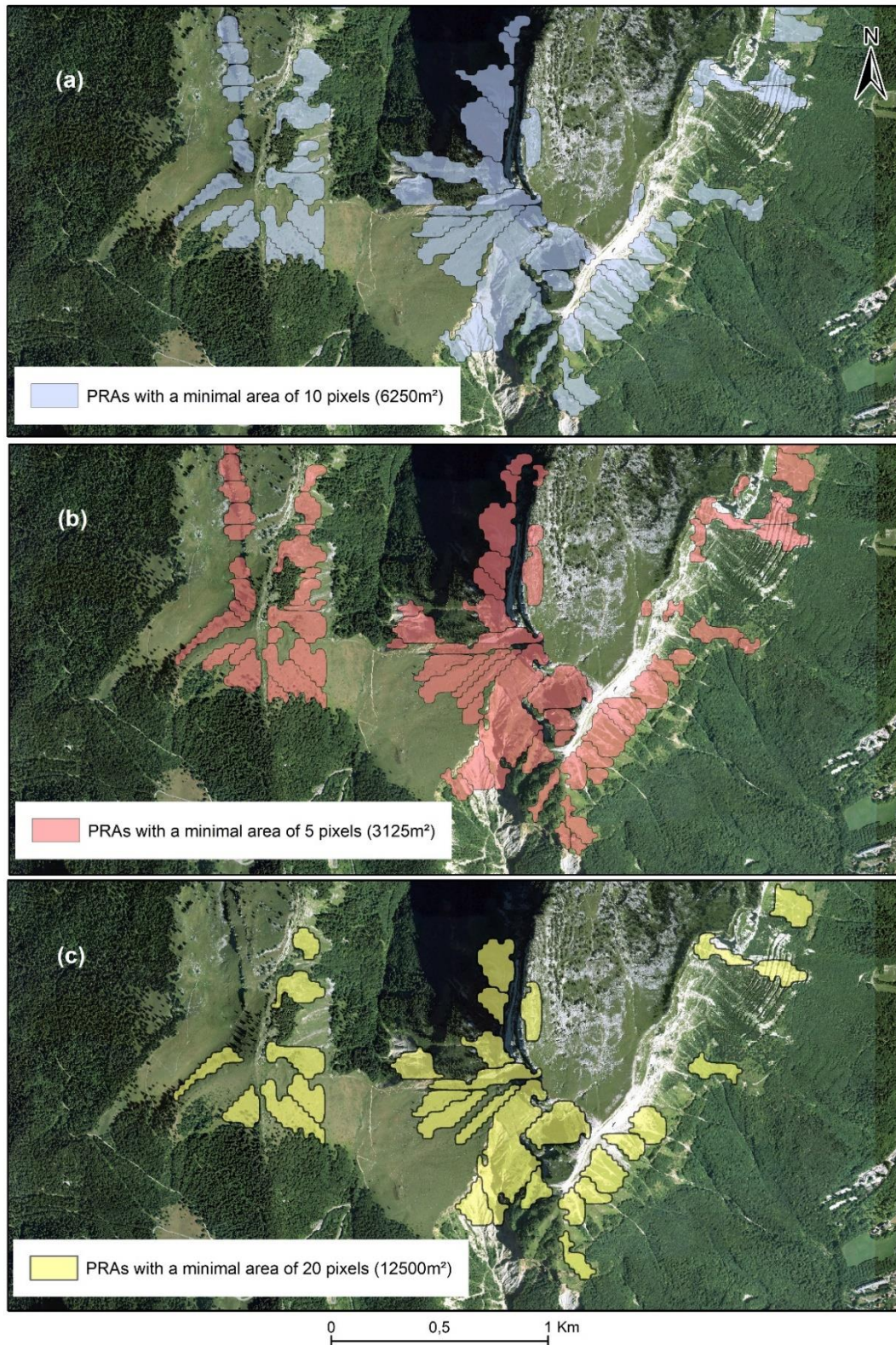
495 Figure 10 : Effect on PRA detection of the minimal area size, Chartreuse/Dent de Crolles study area: a) with a 6250 m 2 minimal area size, b) with a 3125 m 2 minimal area size, c) with a 12500 m 2 minimal area size. For the PRA detection, minimal area size varies, all other factors and the DEM resolution are set to their default values (Figure 3) and forest cover data is from DB forest IGN. Aerial photograph ©IGN 2012. For the determination of the validation sample, all factors and the DEM resolution are set to their default values (Figure 4) and forest cover data is from DB forest IGN.
