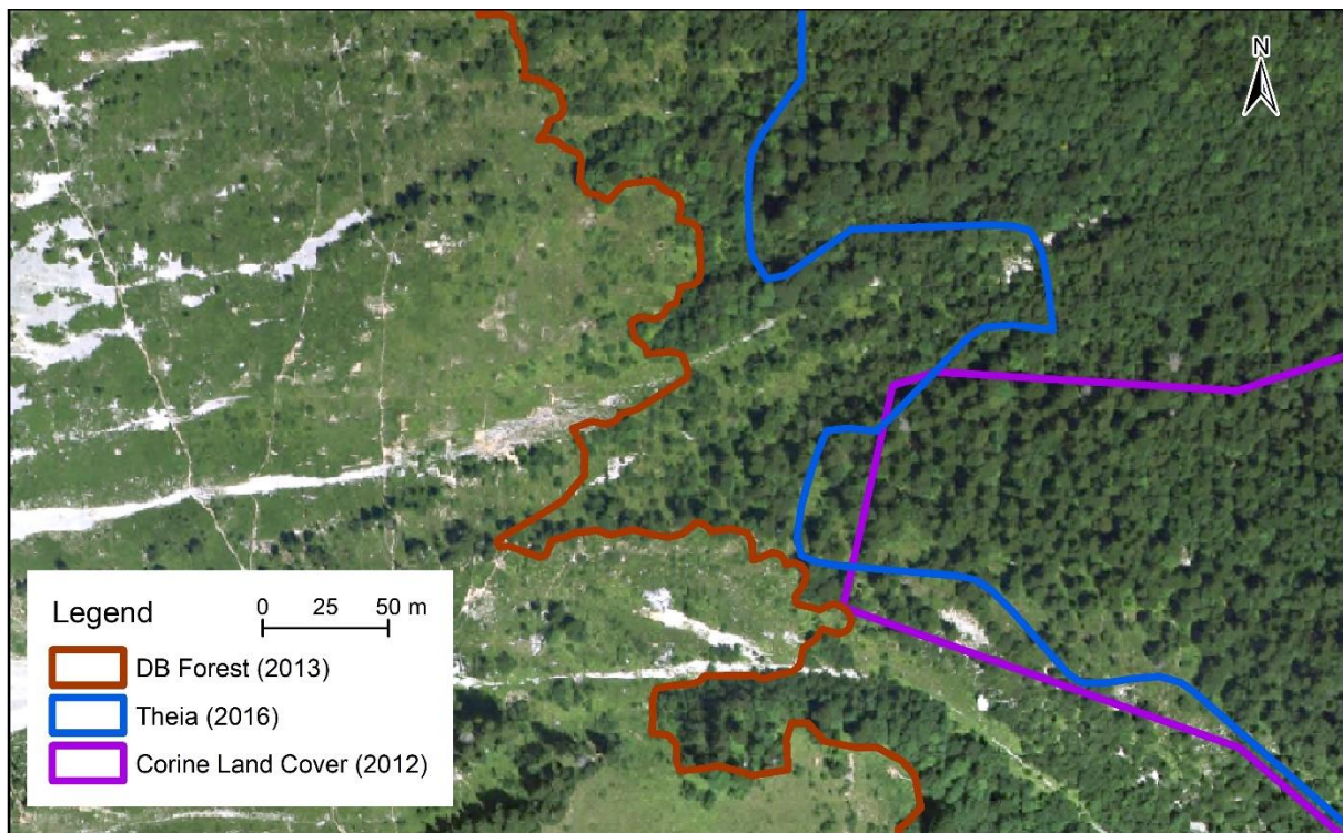
180 Figure 2: Comparison of forest extents from Theia, Corine land cover, and DB Forest from IGN with aerial photographs (©IGN) taken in 2012 within the municipality of Le Sappey-en-Chartreuse, Chartreuse / Dent de Crolles study area.
