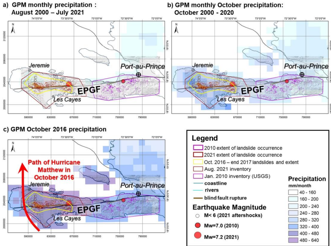
682 Figure 7: Monthly © Global Precipitation Measurement Mission (NASA) maps (0.1° resolution, values in 683 mm/month) for southwestern Haiti, (a) for all months between August 2000 and July 2021, (b) for the month 684 of October between 2000 and 2020, and (c) for October 2016 (marked by the Hurricane Matthew event).
