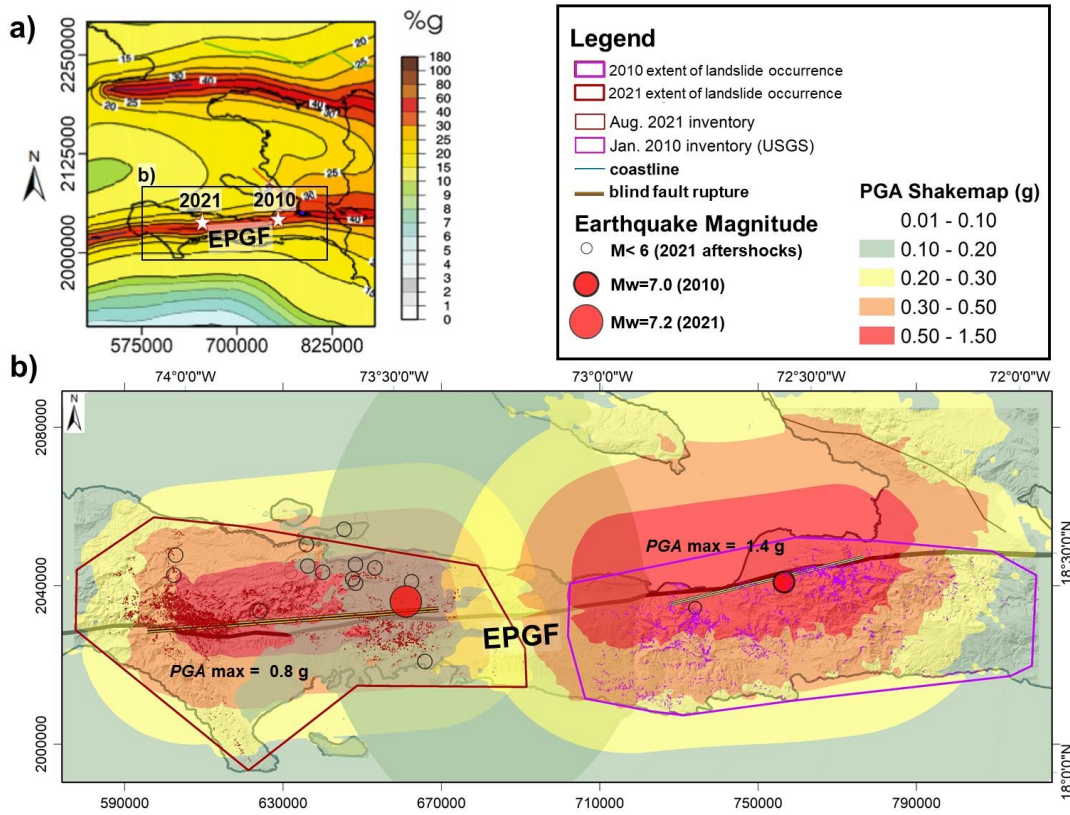
1093 Figure A1: a) Seismic hazard map of Haiti (modified from Frankel et al., 2011) with location of the January 1094 12, 2010, and August 14, 2021, main epicenters. b) Combined overlays of shakemaps of the 2010 (right part 1095 of map) and 2021 (left part) earthquakes.
