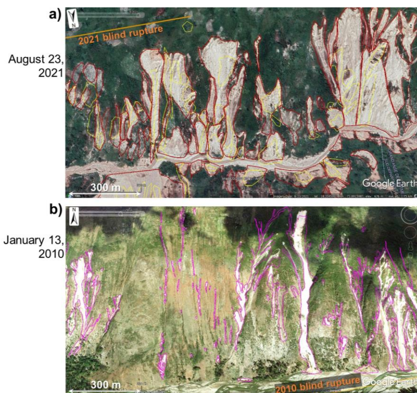
447 448 449 Figure 5: a) GEPPro view (© Google Earth Pro) of landslides triggered by the August 2021 earthquake. b) 450 GEPPro view (© Google Earth Pro) of landslides induced by the January 2010 main shock (with landslide 451 outlines by Harp et al., 2016).
