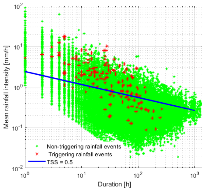
Figure 6: Traditional power-law threshold on the log-log plane between observed mean rainfall intensity ( I ) and duration ( D ).
