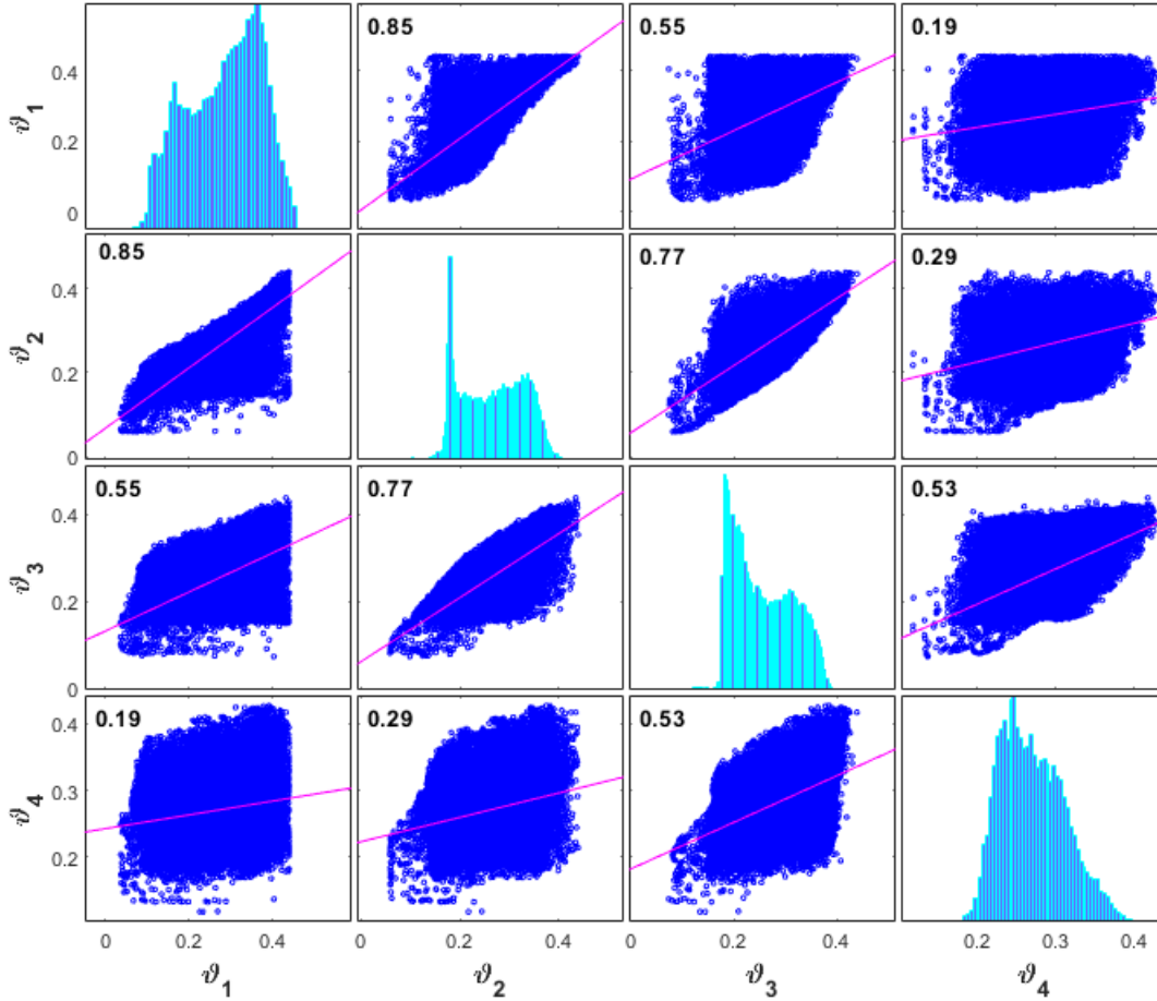
335 Figure 4: Correlation matrix between the four soil moisture level depths ( \vartheta_1, \vartheta_2, \vartheta_3, \vartheta_4 ). Each off-diagonal subplot contains a scatterplot of a pair of variables with a least-squares reference line, the slope of which is equal to the displayed Pearson correlation coefficient. Each diagonal subplot contains the distribution of a variable as a histogram.
