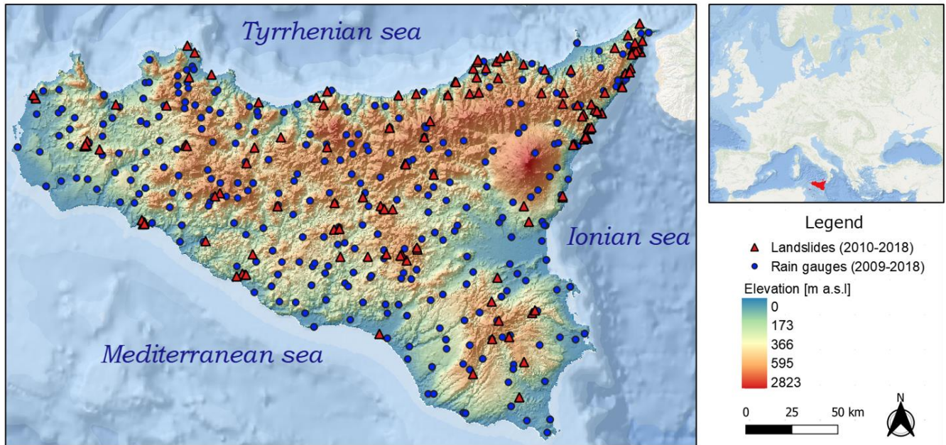
270 Figure 3: Elevation map of the study area (Sicily region), showing the location of the rain gauges and landslide occurrences. (Credit to: http://www.sinanet.isprambiente.it/it/sia-ispra/download-mais and ESRI 2020).
