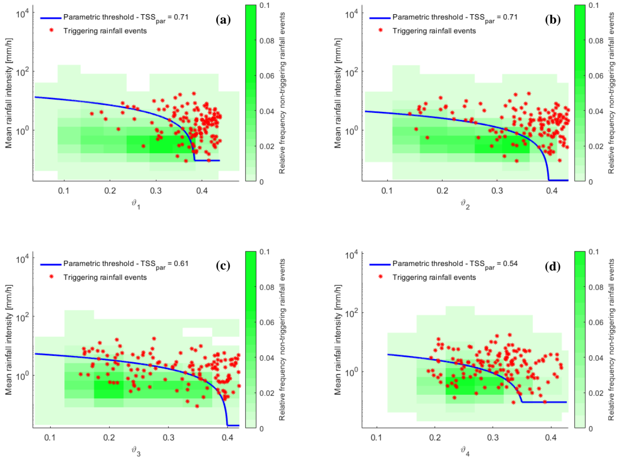
360 Figure 8: Parametric thresholds on the semi-log plane between mean rainfall intensity and soil moisture at the four distinct depths: (a) \vartheta_1 0-7 cm; (b) \vartheta_2 7-28 cm; (c) \vartheta_3 28-100 cm; (d) \vartheta_4 100-289 cm.
