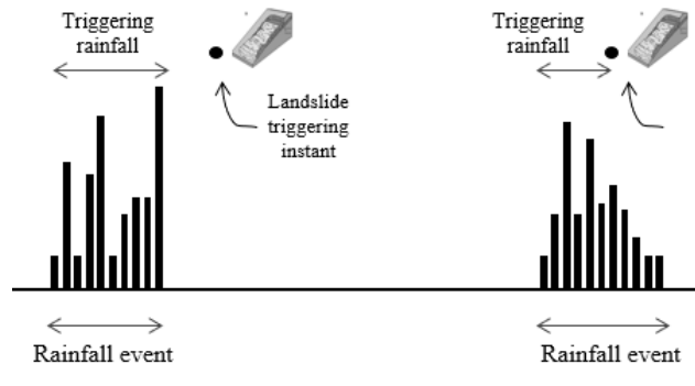
Figure 2: Sketch illustrating how the duration of a triggering rainfall event is defined (adapted from Peres et al., 2018)
