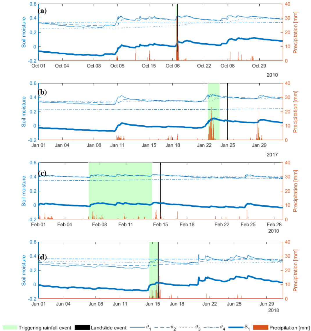
335 Figure 6: Panel showing four different triggering rainfall events. For each of them the precipitation time series together with the soil moisture time series ( \vartheta_1, \vartheta_2, \vartheta_3, \vartheta_4 ) are reported, as well as the first principal component of soil moisture S_1 and the timing of each landslide.
