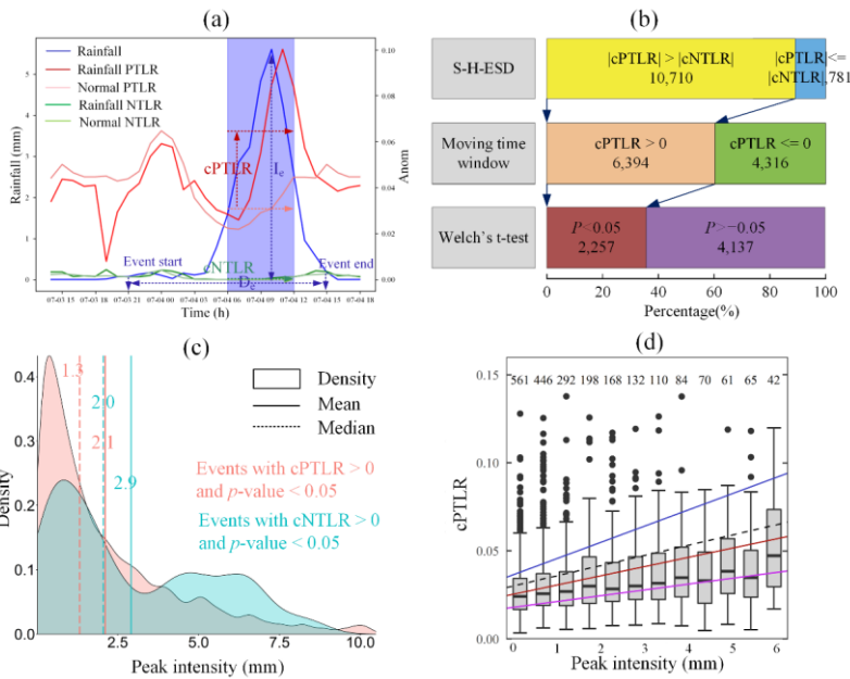
Fig. 3 (a) The schematic definitions of the human activity anomaly associated with a specific rainfall event used in this study. (b) The relative proportions and numbers of the rainfall events with various cPTLR and cNTLR values. (c) The probability density distribution curves of the events with significantly increased cPTLR/cNTLR. (d) Box plots by peak rainfall intensity groups per 0.5mm. Trend lines are shown for the OLS regression (black dotted), 0.25 (purple), median (red), 0.75 quantile (blue) range. The numbers in Fig. 3(d) show the numbers of rainfall events with specific peak intensity as shown along the x axis.
