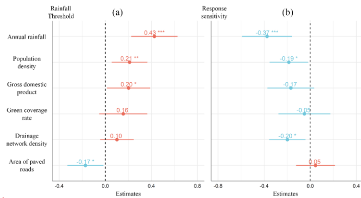
Fig. 7-8 Regression coefficients between the six explanatory variables and the 6-hour rainfall threshold (a), response sensitivity (b). The horizontal lines mean 95% confidence interval.
