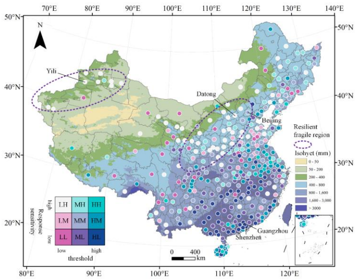
Fig. 6-7 Spatial distribution of urban resilience. The basemap colors indicate the 2017 annual rainfall.
