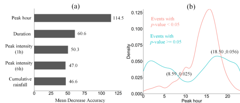
Fig. 4. (a) The importance of the five rainfall indicators obtained by the random forest model. The peak hour is the most important covariate that triggers human activity anomalies and has the highest decrease accuracy value of 114.5. (b) The peak hour thresholds identified from the differences of the peak hour PDF values between the rainfall events with and without significant collective human activity anomalies. When the peak hours are between 8:59 am and 6:50 pm, the PDF values of the events with human activity anomalies are higher than those without. In other words, daytime rains are more likely to trigger human activity anomalies. There are 11,491 daytime rains (i.e., from 8.59 am to 6.50 pm) out of the total 20,860 rainfall events (ratio: 55.11%).
