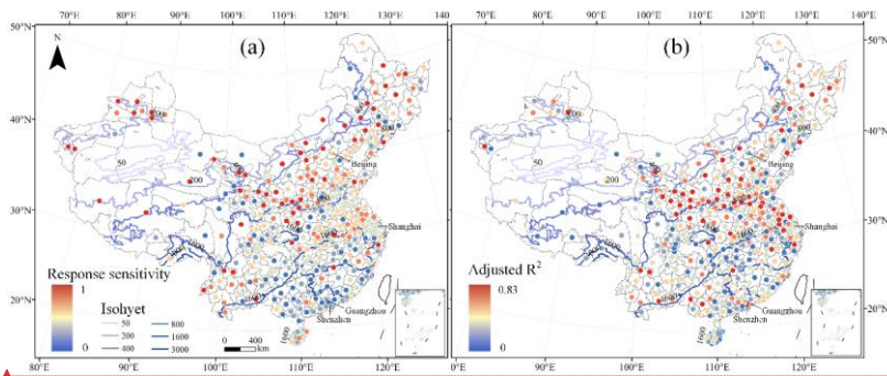
Fig. 5-6 Spatial distribution of the response sensitivity (a) and adjusted R^2 (b) in multiple linear regression. The isohyets show the 2017 annual rainfall.
