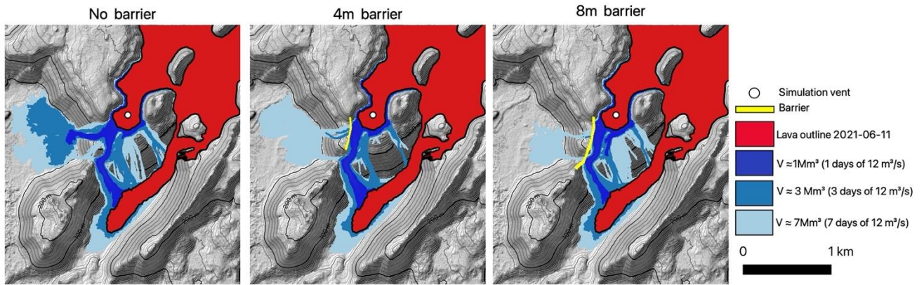
805 Figure 8: An example of lava simulations predicting how Geldingadalir would overflow with and without lava barriers. The simulation vent is located in southern Geldingadalir based on observation of lava inflation in that area. Data based on survey from June 11, 2021 and the calculated volumes and time scales are based on the estimated TADR from the same survey. Background topography is based on the IslandsDEM (Porter et al., 2018).
