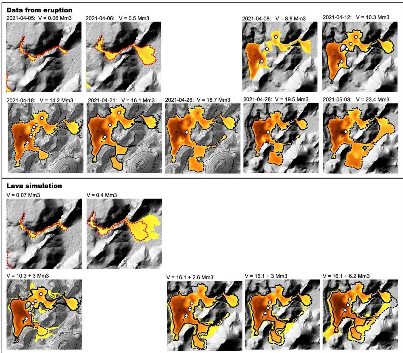
785 Figure 6: Comparison between thickness maps obtained from the lava field (Pedersen et al., 2022b) from April 5 to May 3 (Upper box) and lava simulation thickness maps performed during the vent migration phase (Lower box). The lava simulations in the bottom panel show the cumulative thickness of the syn-eruptive thickness map and the results from the simulation. The volume of each thickness map is noted above each map, which for the cumulative thickness maps is split into the volume contribution from the syn-eruptive thickness map and the simulation (e.g., V=16.1 + 6.2 \text{ Mm}^3 ). The thickness scale is the same for DDEMs and lava simulation thickness maps going from 0 m (yellow) to 50 m (brown). The extent of the thickness maps used as input to the simulation has a solid black outline, while the extent of the lava thickness maps from the lava field with comparable volume is marked with hatched outlines. The active vents are in white, except for fissure 2 (top left), where the initial two fissure segments are shown as black lines. Background topography is based on the IslandsDEM (Porter et al., 2018). 790
