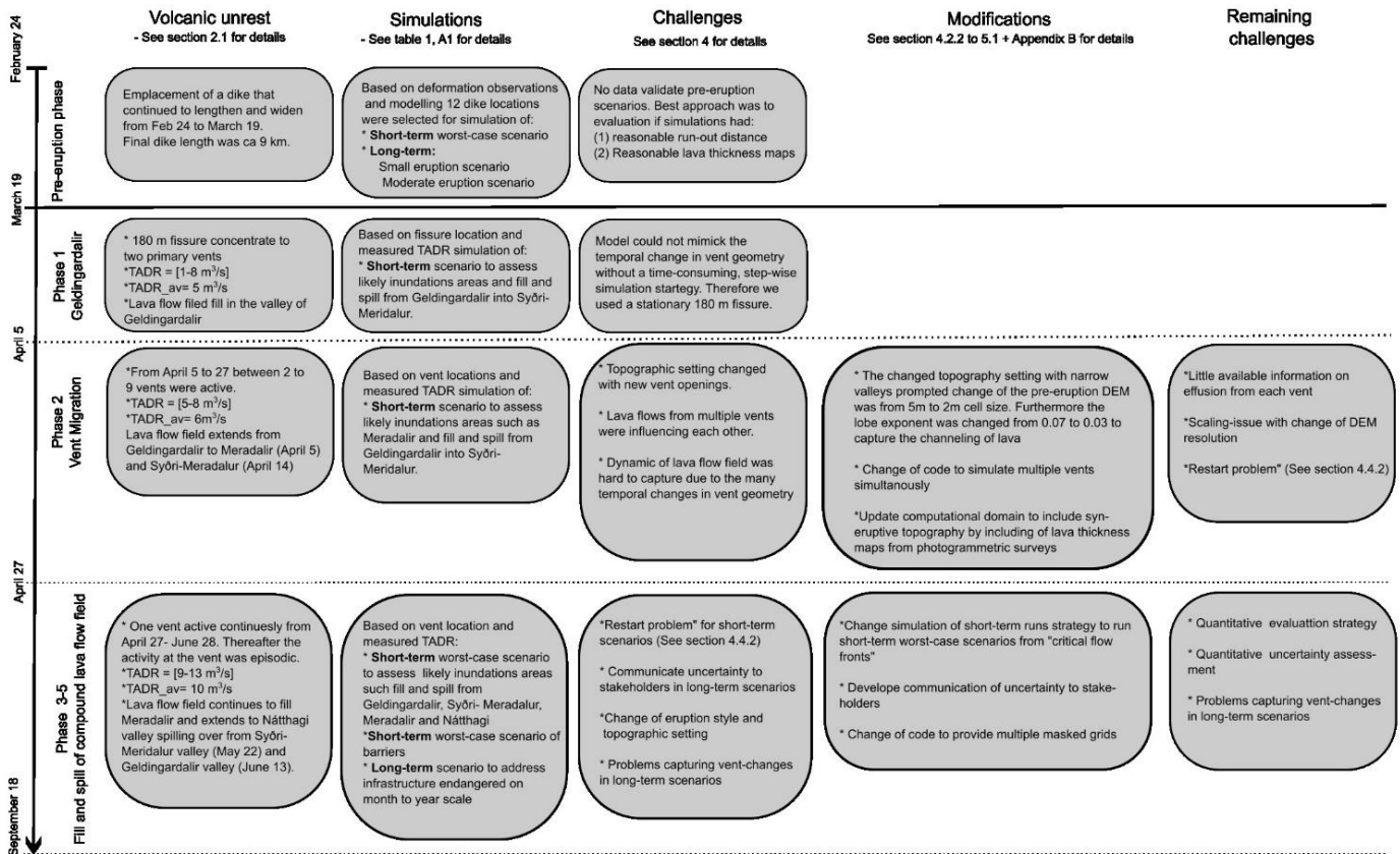
760 Figure 2: Illustration of the temporal development of the volcanic unrest (first column), the simulations performed addressing these developments (column 2), the identified simulation challenges (column 3), the modifications implemented to address these challenges (column 4) and the remaining challenges.
