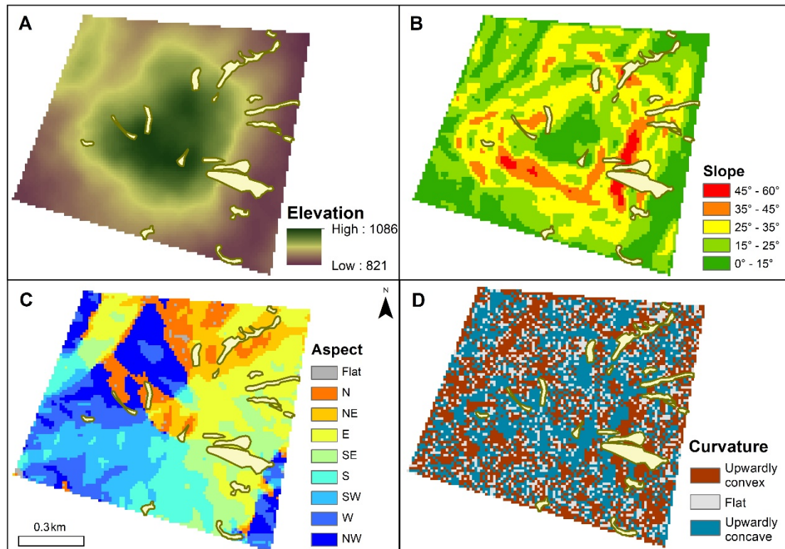
320 Figure 6. Distribution map of terrain attributes in the study area of Petrópolis. (A) Elevation (B) Slope (C) Aspect and (D) Curvature of Petrópolis. Light yellow polygons represent the extent of the February 2022 landslide patches.
