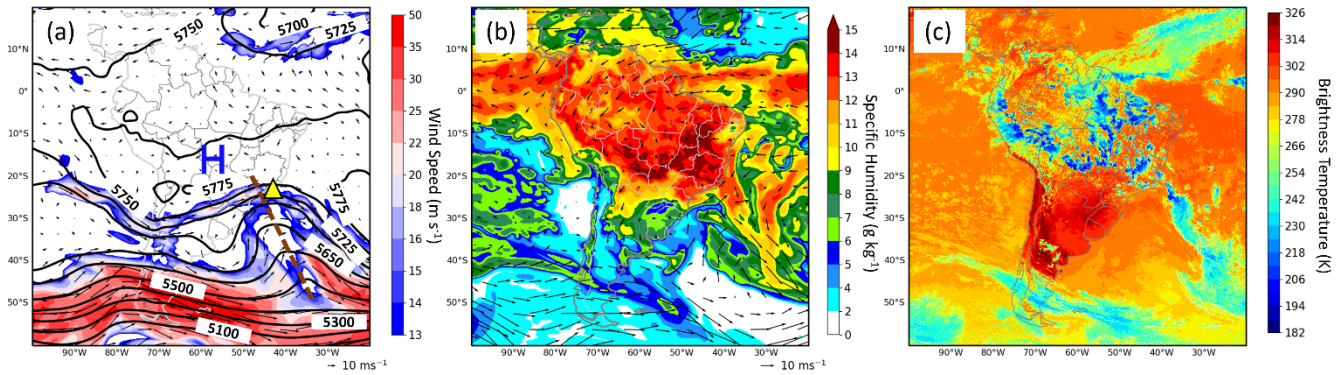
260 Figure 2: Large-scale environmental variables and satellite observation at 16:00 (local time). (a) wind speed (shading), geopotential height (contour), and winds (arrow) at 500 hPa, where the trough line is indicated using a brown dash line and the location of Petrópolis is highlighted by a yellow triangle. (b) Specific humidity (shading) and winds (arrow) at 850 hPa. (c) Merged IR brightness temperature, where cold color represents the presence of deep clouds.
