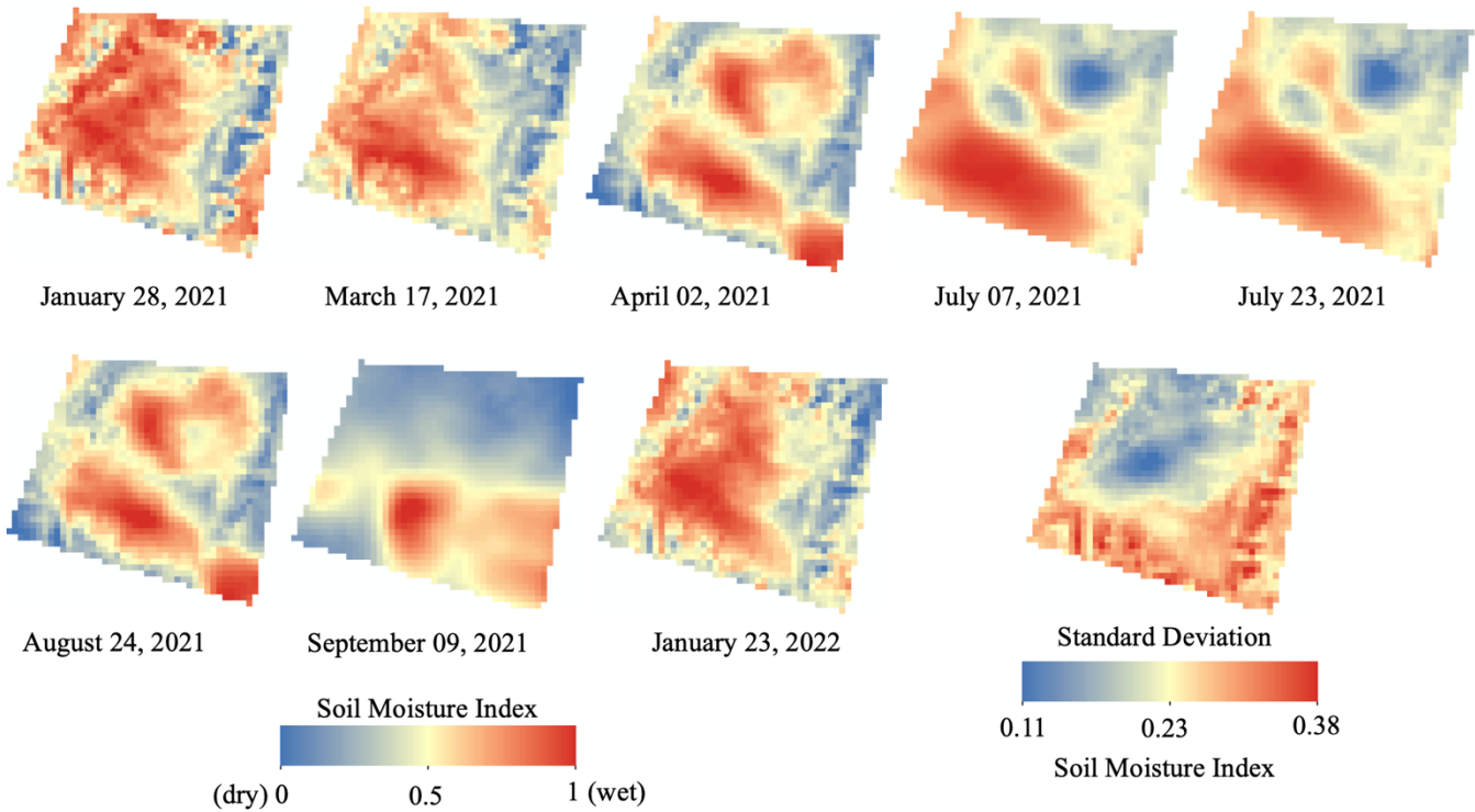
365 Figure 8: Soil moisture index from January 28, 2021 to January 23, 2022.
