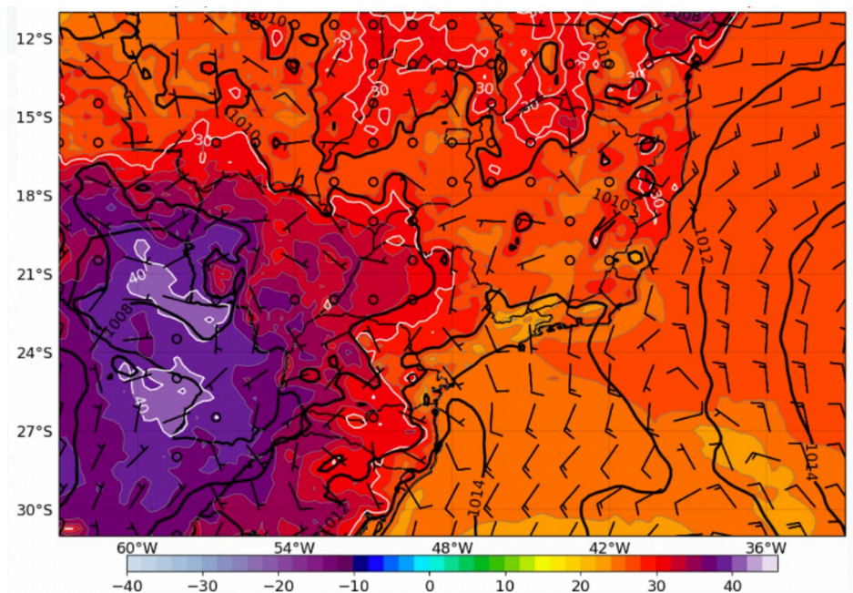
Figure 13. GFS analysis at 18:00 UTC for February 15 2022, for the Petrópolis region. Shades represent surface temperature, isolines represent sea level pressure and the barbs shows wind speed (in knots).
