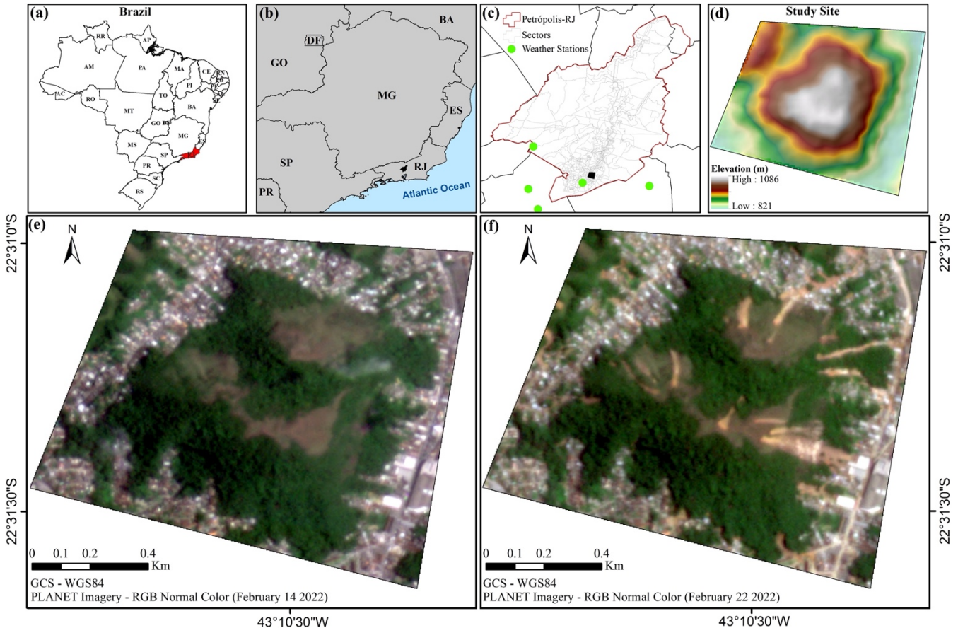
Figure 1: Petrópolis and the study site. (a) location of Rio de Janeiro State in Brazil, (b) location of the study site in the Rio de Janeiro State. (a) – (b) were based on the Brazilian Institute of Geography and Statistics (IBGE). (c) location of the study site into Petrópolis city and the position of weather stations and (d) elevation map of the study site (ALOS/PALSAR, https://asf.alaska.edu/data-sets/sar-data-sets/alos-palsar/ ). (e) Planet image natural color from February 14, 2022, (f) Planet image natural color from February 22, 2022
