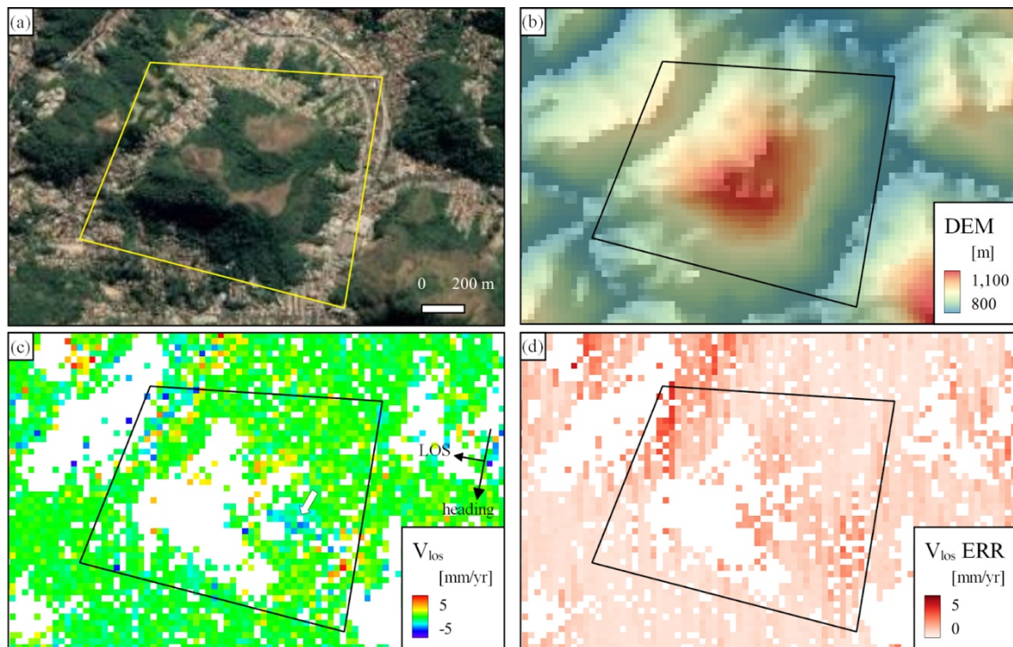
380 Figure 9: (A) Optical image before February 2022 landslides (Image from Google Earth Pro). (B) Digital Elevation Map (ALOS/PALSAR). (C) InSAR line-of-sight (LOS) velocity between May 8, 2015 and December 20, 2021. Note that most areas have nearly zero deformation except for the eastern slope (pointed by a white arrow). (D) Standard deviation of LOS velocity.
