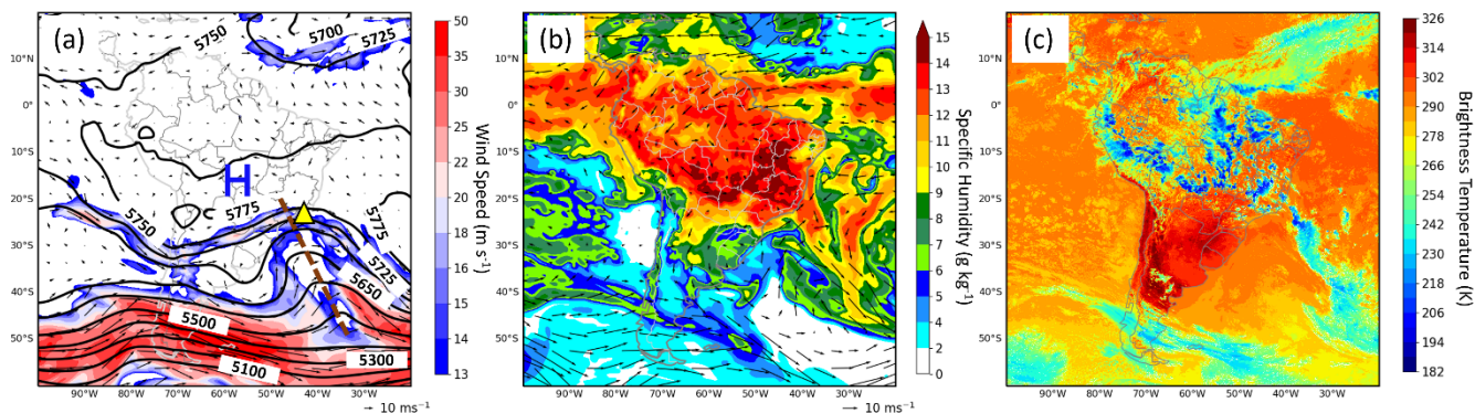
260 Figure 2: Large-scale environmental variables and satellite observation at 16:00 (local time). (a) wind speed (shading), geopotential height (contour), and winds (arrow) at 500 hPa, where the trough line is indicated using a brown dash line and the location of Petrópolis is highlighted by a yellow triangle. (b) Specific humidity (shading) and winds (arrow) at 850 hPa. (c) Merged IR brightness temperature, where cold color represents the presence of deep clouds.
