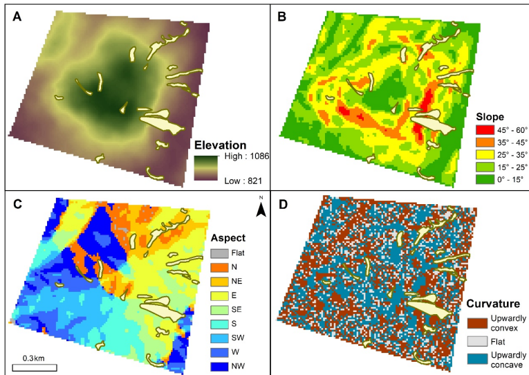
Figure 5. Distribution map of terrain attributes in the study area of Petrópolis. (A) Elevation (B) Slope (C) Aspect and (D) Curvature of Petrópolis. Light yellow polygons represent the extent of the February 2022 landslide patches.
