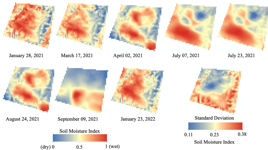
Figure 7: Soil moisture index from January 28, 2021 to January 23, 2022.
