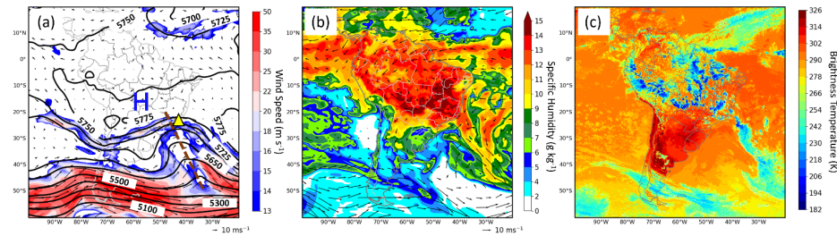
Figure 2: Large-scale environmental variables and satellite observation at 16:00 (local time). (a) wind speed (shading), geopotential height (contour), and winds (arrow) at 500 hPa, where the trough line is indicated using a brown dash line
