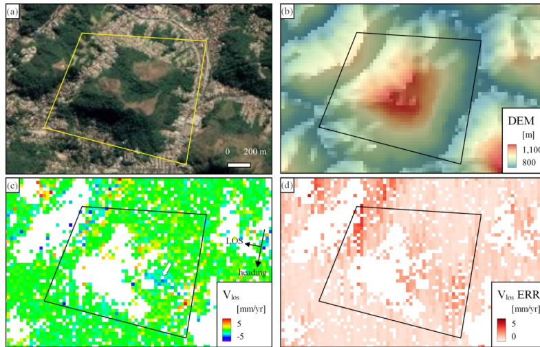
630 Figure 8: (A) Optical image before February 2022 landslides (Image from Google Earth Pro). (B) Digital Elevation Map (ALOS/PALSAR). (C) InSAR line-of-sight (LOS) velocity between May 8, 2015 and December 20, 2021. Note that most areas have nearly zero deformation except for the eastern slope (pointed by a white arrow). (D) Standard deviation of LOS velocity.
