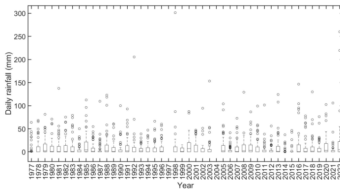
Figure 3: The Long-Term precipitation time-series was created from 2 weather stations from INMET (A603-Duque de Caxias and A610-Pico do Couto), 2 weather stations from INEA (2243238-Xerem and 2243235-Andorinhas), and one from Cemaden (Sao Sebastiao).
