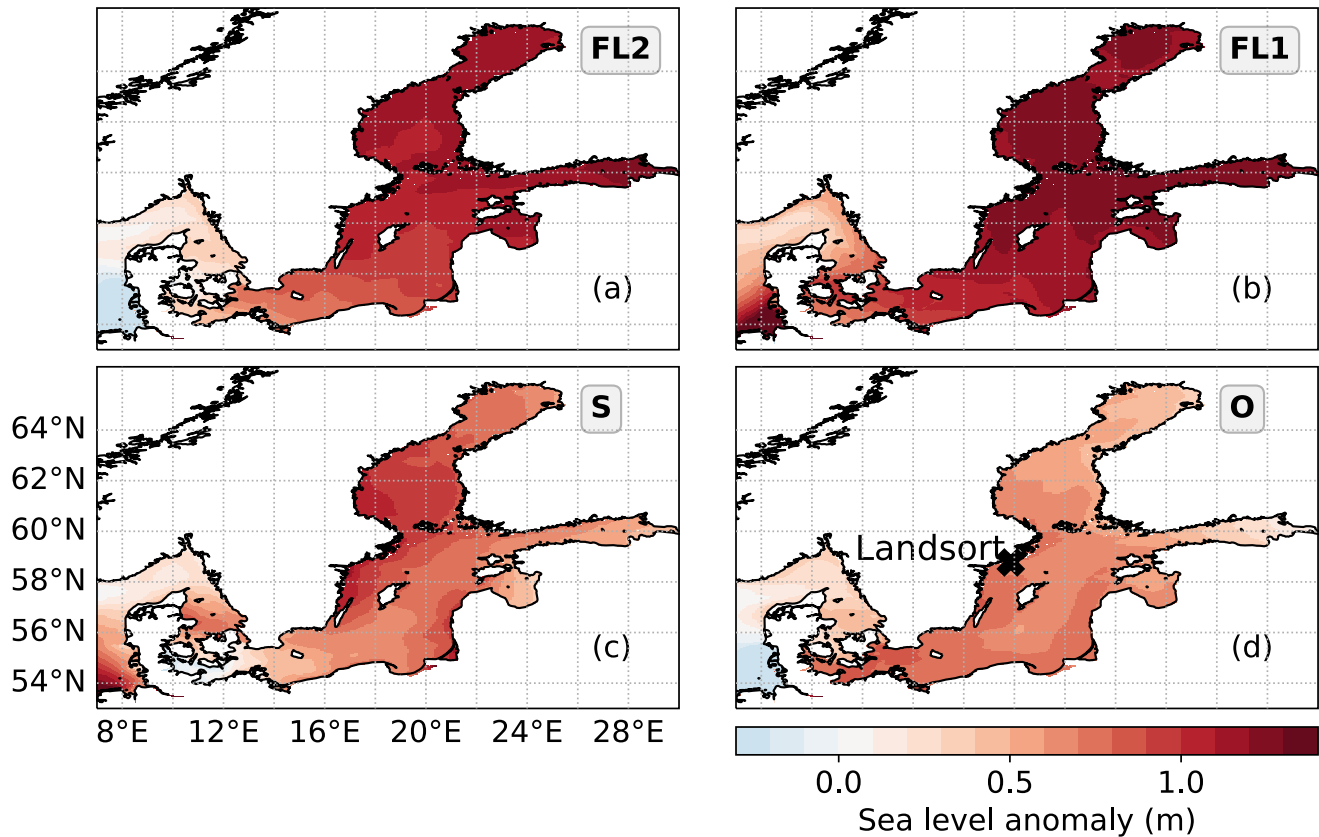
Figure 2. The sea level anomaly field that corresponds to the maximum water level at Landsort for each simulation (see Fig. 3 for time series). The magnitude of the sea level anomalies are indicated by the colorbar. Panel (d) shows the unperturbed case (O) from 14:00 11 November 1872. Preconditioning for the sea level anomalies in panels (a) and (b) were obtained from an ocean hindcast (Andrée et al., 2021). The time is adjusted to match case O. Therefore, the time steps shown correspond to 9 November at 19:00 (FL2) and midnight (FL1), respectively. Case S (panel (c) uses the same conditions as O, except that the atmospheric forcing between midnight on 9 November and up until 15:00 on 12 November 1872 are is replaced by the corresponding times from 1st to 4th January 2017. The panel represents 04:00 on 12 November. Panel (d) shows the location of station Landsort, which is used to estimate the filling level.
