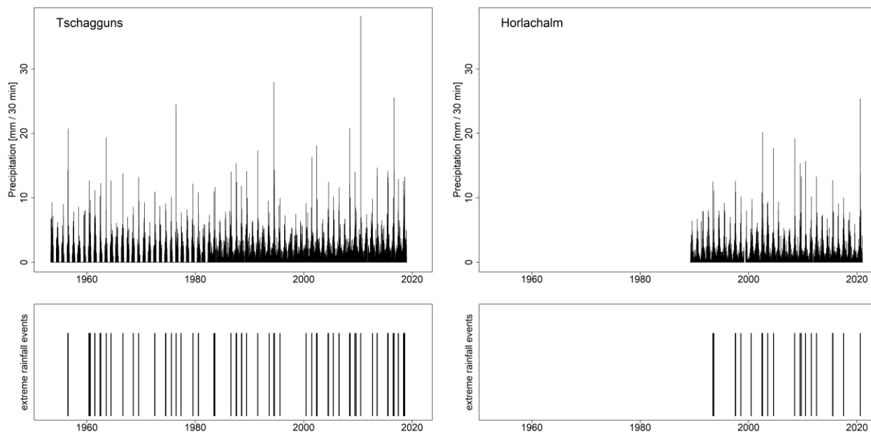
340 Figure 10: Recorded precipitation data of the meteorological stations Tschagguns (left) and Horlachalm (right). Days with intensities exceeding 10 mm per 30 minutes are marked in the respective bottom plots.
