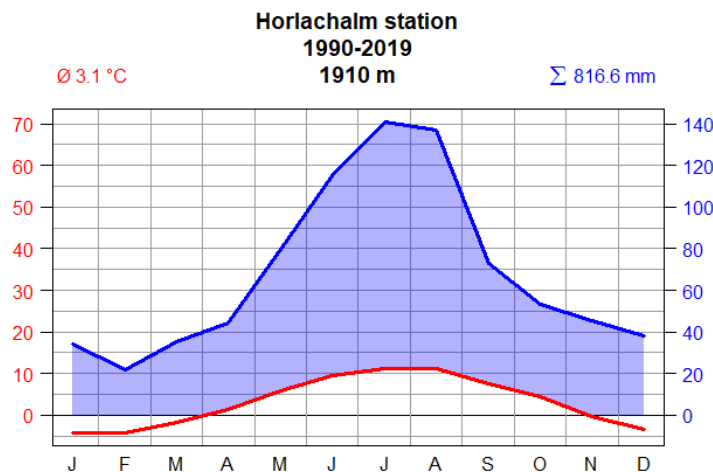
Figure 2: Climate diagram of the Horlachalm station (1910 m) using temperature and precipitation data between 1990 and 2019. Data source: TIWAG.
