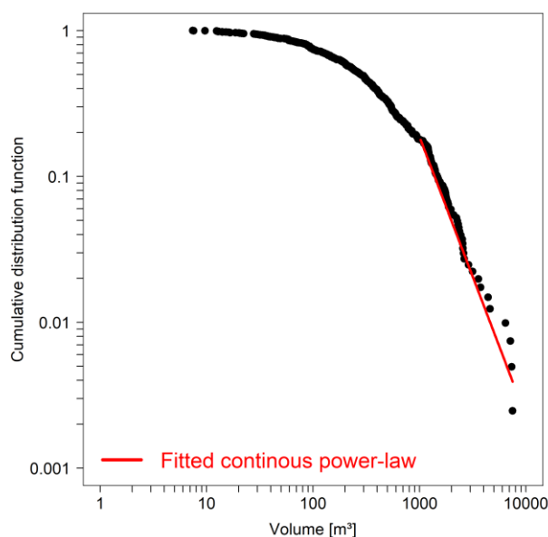
310 Figure 9: Magnitude–frequency relationship displayed with a cumulative distribution function for the debris flows in GT, LT and ZT. The fitted continuous power-law describes the relationship for debris flows with a volume greater than 1025 m 3 .
