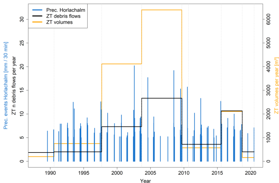
500 Figure 14: High intensity rainfall events exceeding 5 mm per 30 minutes at the Horlachalm station combined with the number of mapped debris flows per year in ZT (black) and the deposited debris flow volumes per year in ZT (orange). The sub-catchment ZT is located quite close to the Horlachalm meteorological station.
