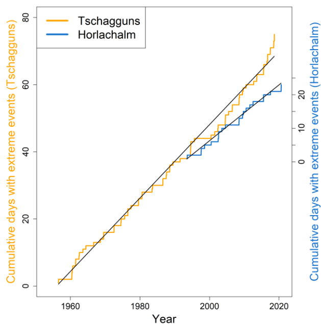
Figure 11: Cumulative sums of days with precipitation intensities exceeding 10 mm per 30 minutes for Tschagguns (orange) and Horlachalm (blue).
