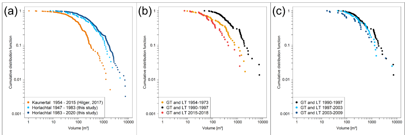
430 Figure 12: (a): Magnitude – frequency relationship for the early debris flows in Horlachtal (1947 – 1983, light blue) compared with recent debris flows (1983 – 2020, dark blue). The results of a similar investigation from Hilger (2017) in Kaunertal is shown in orange. (b): Comparison of the magnitude – frequency relationships of the three highly active debris flow periods in GT and LT. (c): Comparison of the magnitude – frequency relationships for the three consecutive periods 1990–1997, 1997–2003 and 2003–2009 in GT and LT.
