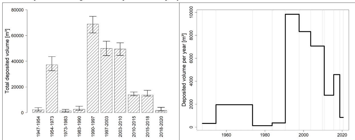
Figure 8: Temporal variability of the volumes deposited by slope-type debris flows in Horlachtal since 1947. Left: The total deposited volume of slope-type debris flows in all sub-catchments in each epoch covered by the orthophotos. Uncertainties of the calculations are added for each time span. Right: The deposited volume of slope type debris flows per year. The dashed vertical lines represent the acquisition dates of the orthophotos used.
