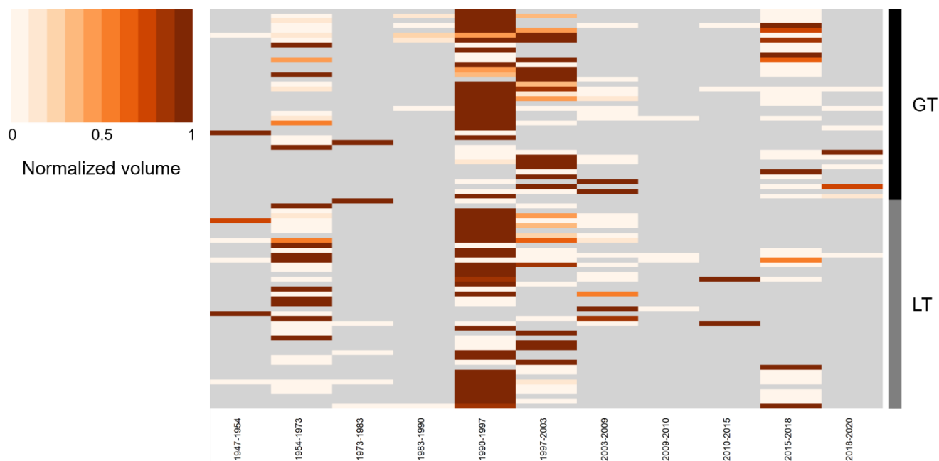
Figure 13: Heatmap of the 82 different starting zones in GT and LT which were triggered at least twice between 1947 and 2020. The normalized magnitudes of every starting zone is shown by the colouring scheme. For more details please refer to the text.
