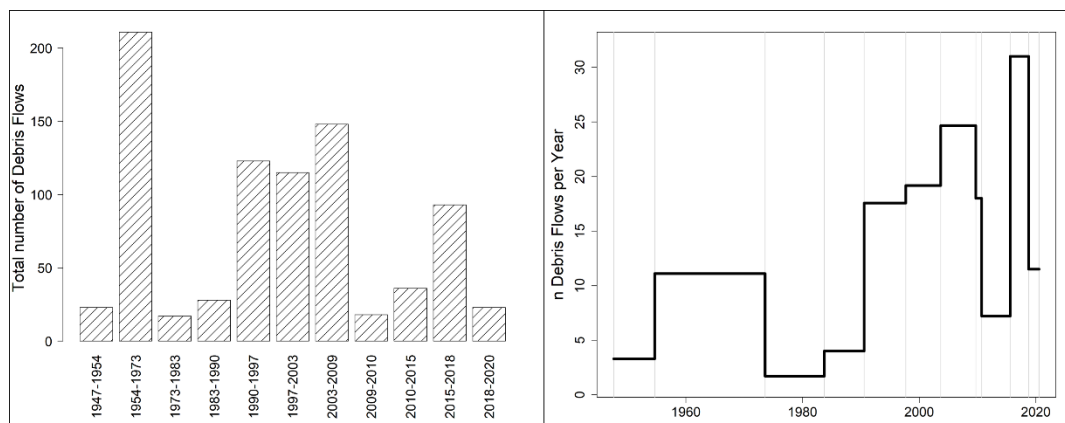
Figure 6: Temporal variations of slope-type debris flow activity in Horlachtal since 1947. Left: The total number of detected slope-type debris flows in all sub-catchments in each epoch covered by the orthophotos. Right: The number of mapped slope type debris flows per year. The dashed vertical lines represent the acquisition dates of the orthophotos used.
