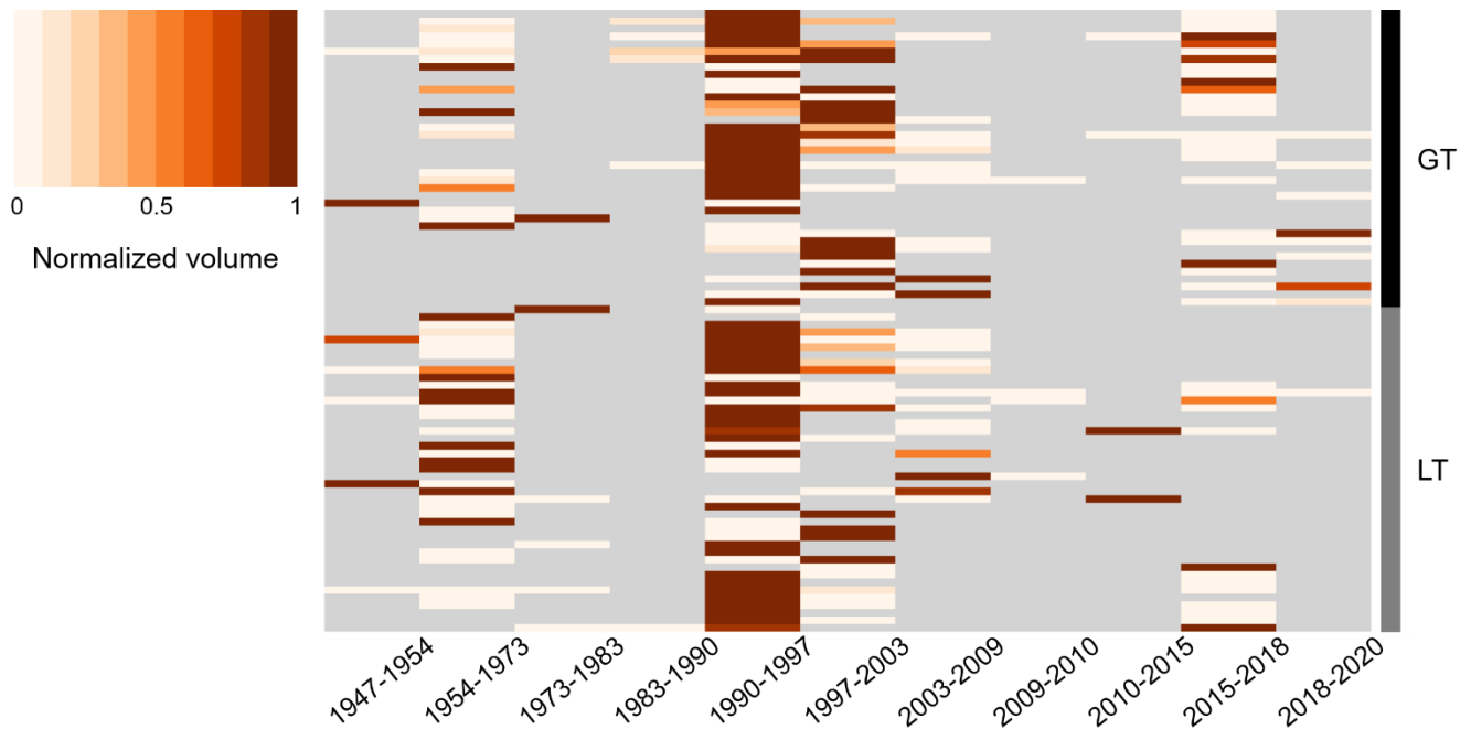
460 Figure 12: Heatmap of the 82 different starting zones in GT and LT which were triggered at least twice between 1947 and 2020. The normalized magnitudes of every starting zone is shown by the colouring scheme. For more details please refer to the text.
