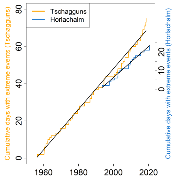
Figure 10: Cumulative sums of days with precipitation intensities exceeding 10 mm per 30 minutes for Tschagguns (orange) and Horlachalm (blue).
