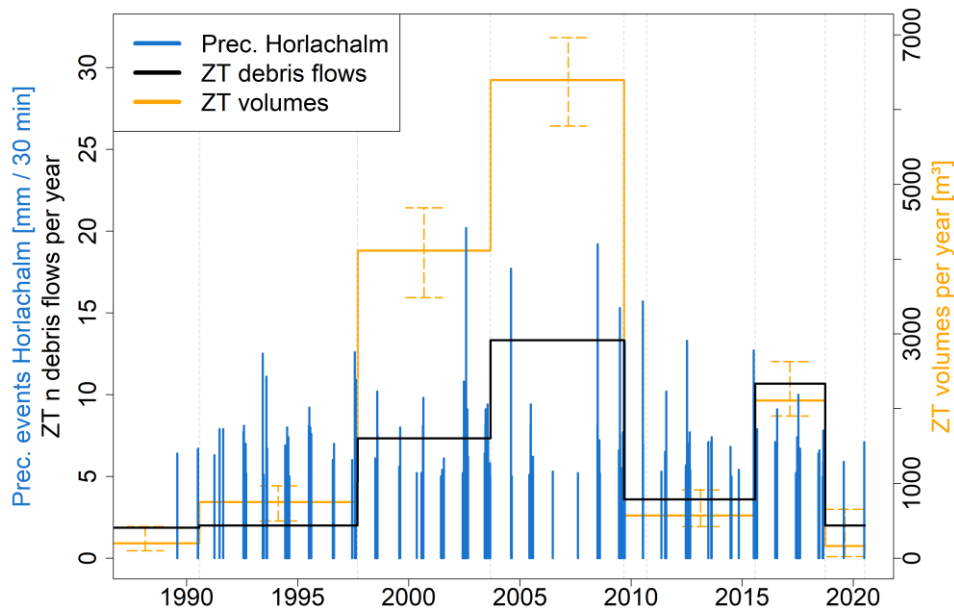
Figure 13: High intensity rainfall events exceeding 5 mm per 30 minutes at the Horlachalm station combined with the number of mapped debris flows per year in ZT (black) and the deposited debris flow volumes per year in ZT (orange). The sub-catchment ZT is located quite close to the Horlachalm meteorological station.
