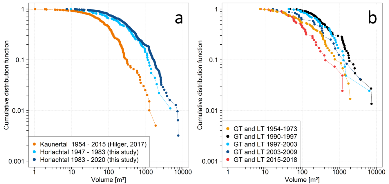
415 Figure 11: Panel a: Magnitude – frequency relationship for the early debris flows in Horlachtal (1947 – 1983, light blue) compared with recent debris flows (1983 – 2020, dark blue). The results of a similar investigation from Hilger (2017) in Kaunertal is shown in orange. Panel b: Comparison of the magnitude – frequency relationships of different periods in GT and LT.
