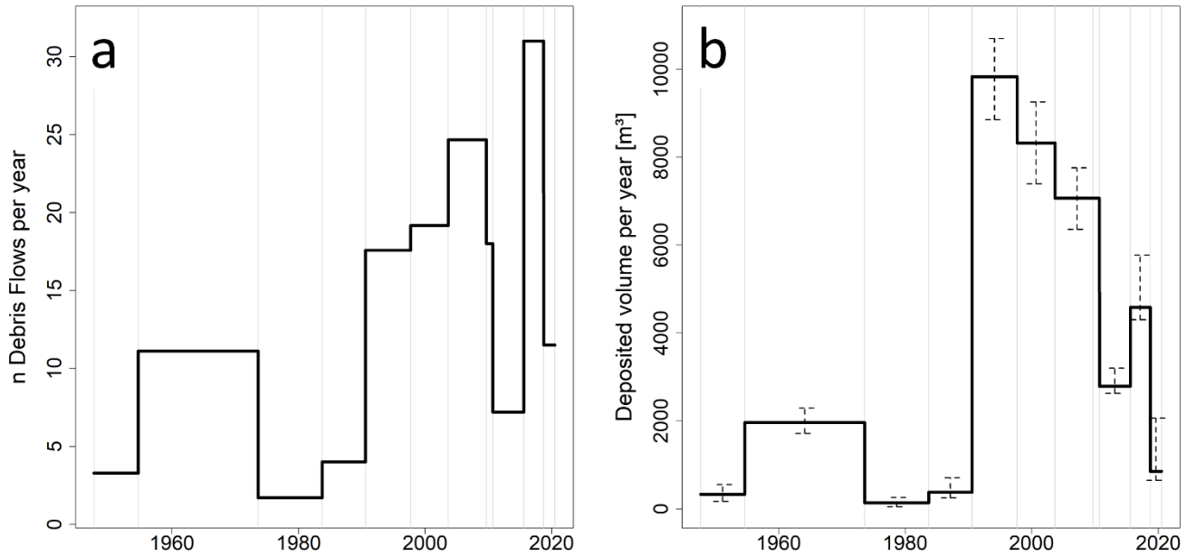
270 Figure 6: Temporal variations of slope-type debris flow activity in Horlachtal since 1947. Panel a: The number of mapped slope-type debris flows per year. Panel b: The deposited volume of slope-type debris flows per year. Uncertainties of the calculations are added for each time span. The light grey vertical lines in both panels represent the acquisition dates of the used orthophotos.
