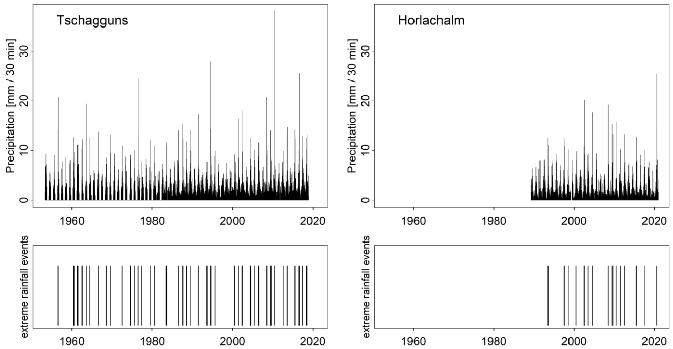
Figure 9: Recorded precipitation data of the meteorological stations Tschagguns and Horlachalm. Days with intensities exceeding 10 mm per 30 minutes are marked in the respective bottom plots.
