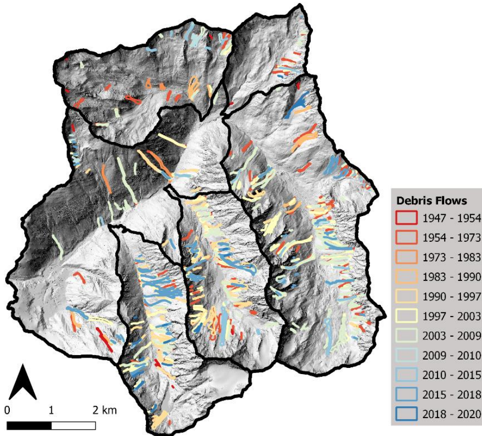
260 Figure 4: Results of the debris flow mapping in the entire study area. More recent debris flows overlay older ones in some places.
