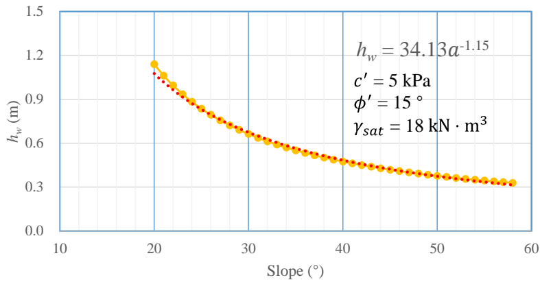
Figure 13. The relationship between the critical depth and the slope.
