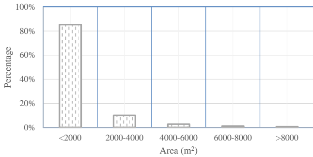
175 Figure 3. Proportion of “7.25” Tianshui sliding-flow landslides in different areas.
