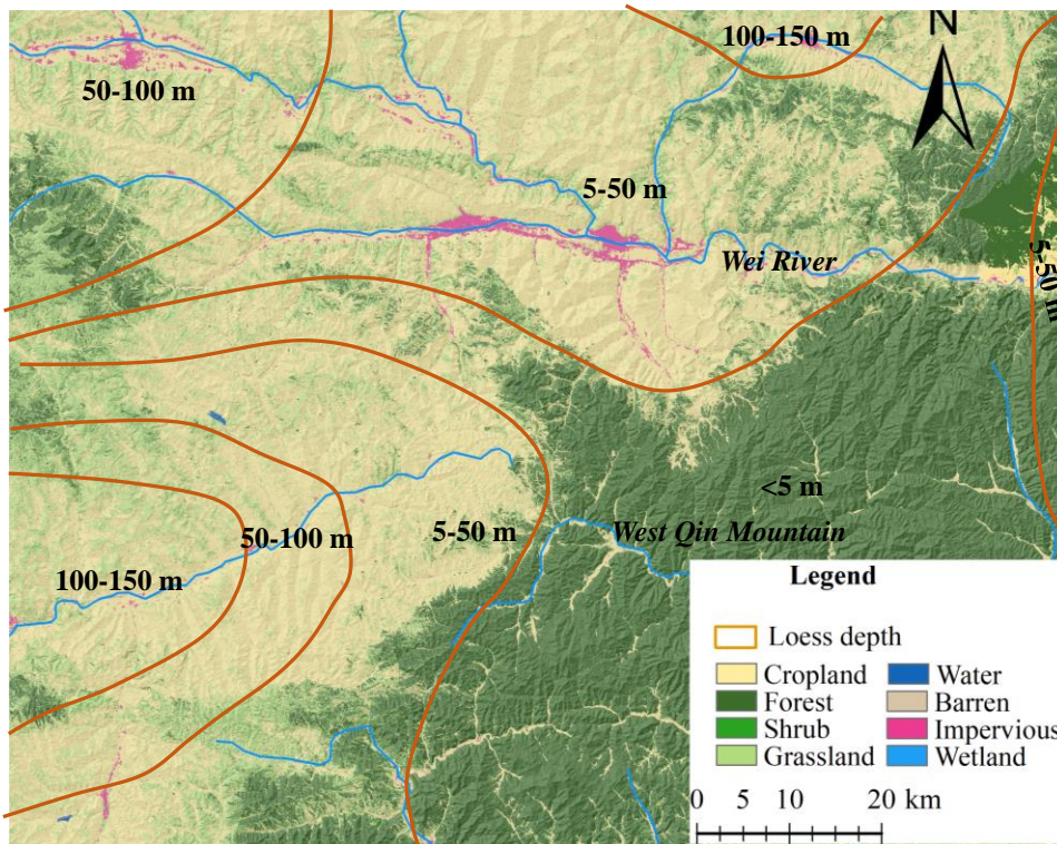
Figure 1. The geological and land use of the study area. Base DEM data from https://geocloud.cgs.gov.cn/#/home , land use data from http://www.geodata.cn .
