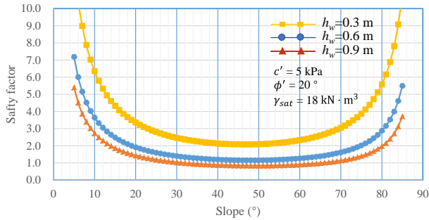
Figure 10. The stability safety factor according to the infinite slope model proposed by Taylor.
