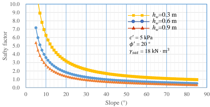
Figure 12. The stability safety factor according to the RISM.
