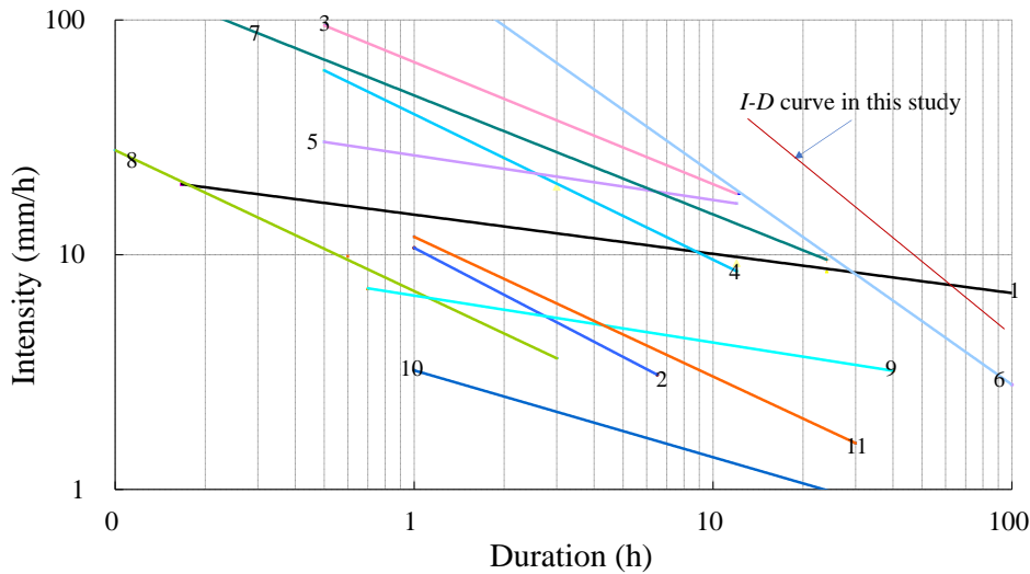
Figure 15. Comparison of I-D curves from the current and prior studies (No.1: Caine 1980; No. 2: Wiczorek 1987; No. 3, 4, 5: Jibson 1989; No. 6: Guadagno 1991; No. 7: Paronuzzi et al. 1998; No. 8: Crosta and Frattini 2001; No. 9: Shieh et al. 2009; No. 10: Guo et al. 2013; No. 11: Zhuang et al., 2015).
