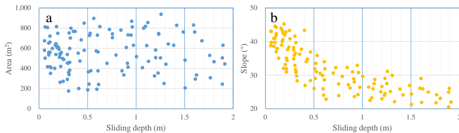
Figure 7. The distribution of sliding-flow landslide depths and area of the “7.25” Tianshui sliding-flow landslides. (a): landslide surface area vs sliding surface depth and; b): slope vs sliding surface depth).
