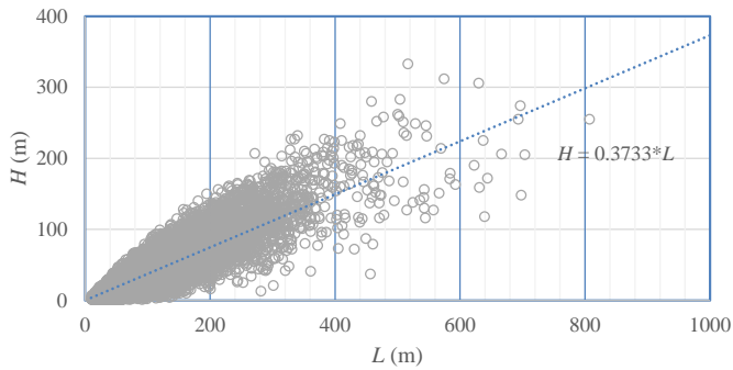
210 Figure 6. The relationship between height difference-differential and travel distance of the “7.25” Tianshui sliding-flow landslides.
