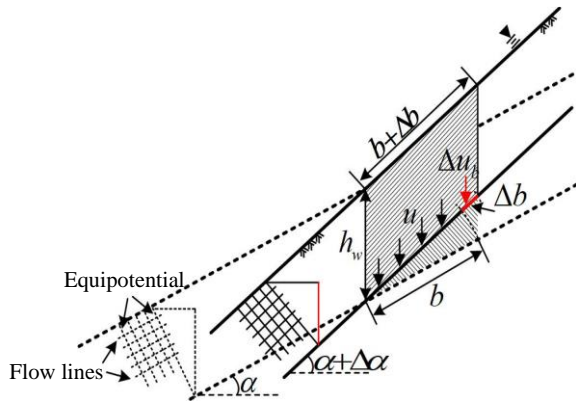
285 Figure 11. Figures demonstrating the infinite slope model with the slope variation in slope.
