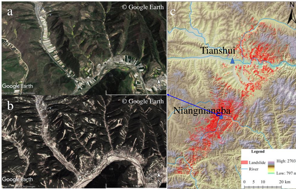
155 Figure 2 The landslides triggered by “7.25” Tianshui sliding-flow landslide events (a: before “7.25” Tianshui sliding-flow landslide events in October 2012; b: after “7.25” Tianshui sliding-flow landslide events in December 2013; c: the landslides distribution triggered by “7.25” Tianshui sliding-flow landslide events)
