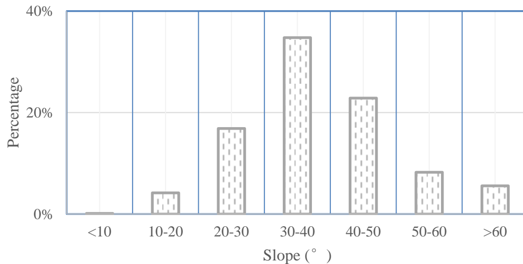
Fig. 1 The distribution of the “7.25” Tianshui sliding-flow landslides vs slope
