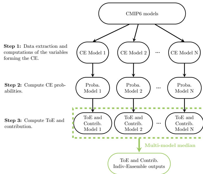
Figure 3. Flowchart for the computations of time of emergence and contributions for Indiv- and Full-Ensemble versions the Indiv-Ensemble version.
