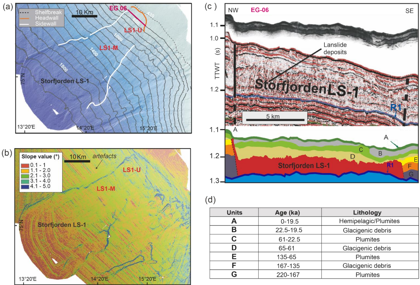
145 Figure 3. Storfjorden and Kveithola interfan TMs. (a) Shade relief colour map of the southwestern continental slope of the Storfjorden and Kveithola interfan TMs. The orange line marks the headwall and the white lines indicate its sidewalls. The pink line corresponds with multichannel seismic profile (EG-06) acquired during EGLACOM cruise. (b) Slope gradient values; artefacts are induced by slope parallel the ship tracks. (c) The top corresponds with the TOPAS subbottom profile (modified from Llopart et al., 2015) and multichannel seismic profile (EG-06, modified from Rebesco et al., 2014), acquired during 150 SVAIS cruise. Both profiles are displayed at the same horizontal and vertical scales to show matching of acoustic facies. At the bottom shows the line drawing of the multichannel seismic profile displaying the seismic stratigraphy, where R1 reflector (in blue) is the base of Storfjorden LS-1 and its top is the unit D (Pedrosa et al., 2011; Rebesco et al., 2014; Llopart et al., 2015). (d) Table with the seismic units and subunits, ages and their lithologies (modified from Llopart et al., 2015).
