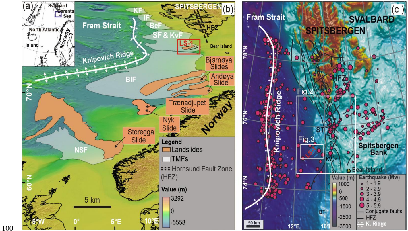
Figure 1. Geographic and geological settings of Storfjorden LS-1. (a) Location map of the study area (blue rectangle). (b) Shaded relief map taken from the International Bathymetric Chart of the Arctic Ocean (IBCAO) version 3.0 (Jakobsson et al., 2012) of North Atlantic Ocean (Norwegian and Barents Sea). The major Trough Mouth Fans (grey polygons), and the major submarine landslides (orange polygons) are located in the map. Compilation from : Haflidason et al. (2005); Laberg et al. (2000); Laberg and Vorren, (2000, 1993); Lindberg et al. (2004); Sejrup et al. (2005), and references therein. KF: Kongsfjorden Fan; IF: Isfjorden Fan; BeF: Bellsund Fan; SF & KvF Storfjorden and Kveithola Fans; BIF: Bear Island Fan; NSF: North Sea Fan. (c) Shaded relief map of northwestern Barents Sea (Ottessen et al., 2016) displaying the location of the Hornsund Fault Zone (HFZ) and the historical earthquakes recorded from 1960 to 2018 (source from IRIS catalogue). This map also shows the locations of figures 2 and 3.
