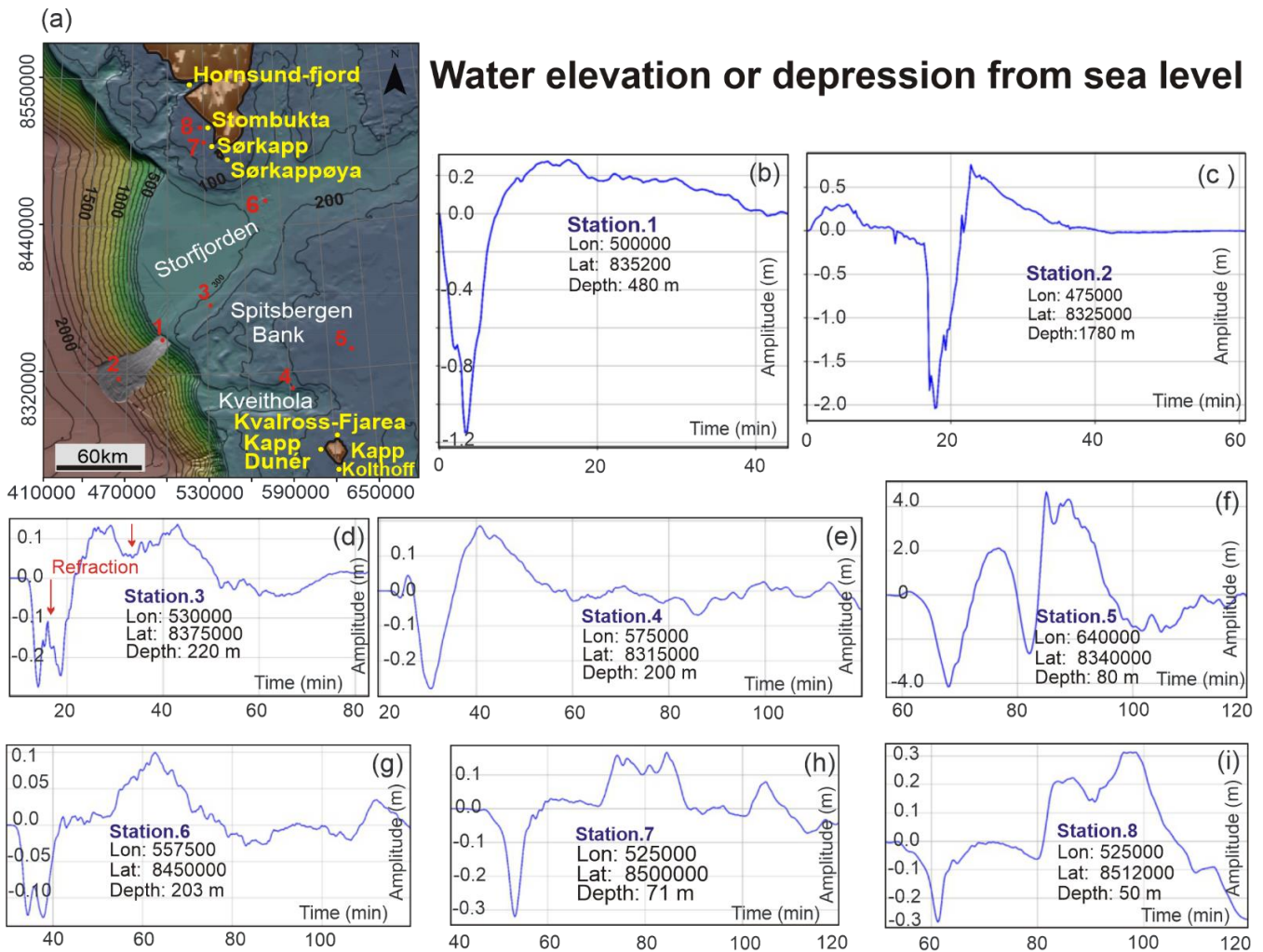
Figure 9. Synthetic marigrams. (a) The location map of the synthetic marigrams above the reference stations, numbered in figure (a) (station 1 to 8). Note the different arrival times, periods, wave heights, and polarities at the different stations (b) to (i).
