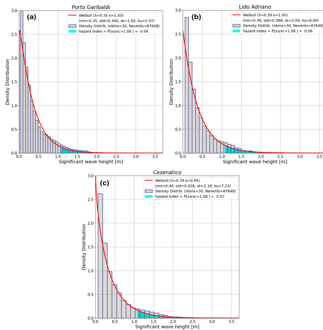
Figure 13. Comparison of the Weibull distribution fit (red line) to the histogram of the model data (2010-2019) for the control points: (a) Porto Garibaldi, (b) Lido Adriano, and (c) Cesenatico. The red line denotes the Weibull fit, the histograms represent the density distribution (seen in grey color), and the hazard index is indicated in cyan color [ mn : mean, std : standard deviation, sk : skewness, ku : kurtosis, nbins : number of bins, Nevents : number of events].
