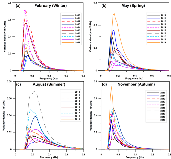
Figure 11. Simulated monthly mean wave spectra for the time slice 2010-19 for (a) February [winter], (b) May [spring], (c) August [summer], and (d) November (autumn) at station 6 (Cesenatico, see Fig. 1c for location).
