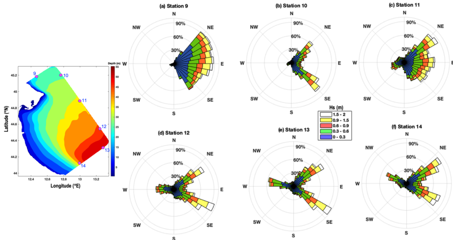
Figure 9. Offshore wave climate: Wave rose diagrams in the boundaries of the model domain for the control points (9 to 14) as indicated in the location bathymetric map shown adjacent (left) [N: North, NE: Northeast, E: East, SE: Southeast, S: South, SW: Southwest, W: West, NW: Northwest].
