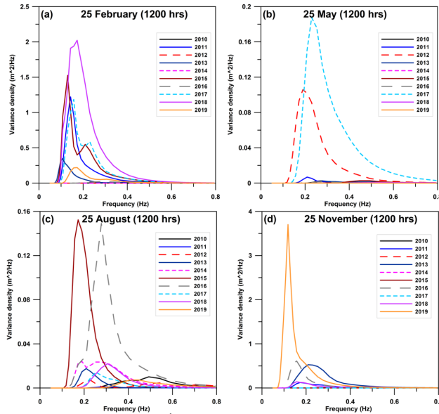
Figure 10. Simulated wave spectra for 2010-19 on the 25 th day (1200 hrs) of (a) February [winter], (b) May [spring], (c) August [summer], and (d) November (autumn) at station 6 (Cesenatico, see Fig. 1c for location).
