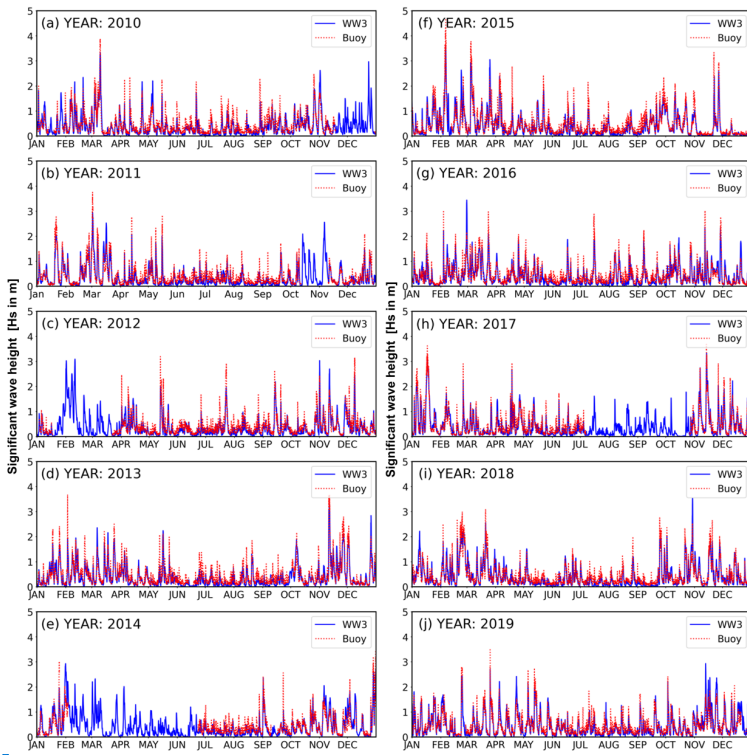
Figure 2. Time series plot of (a-j) significant wave height (in metres, indicated by blue solid lines) and observations (red dotted lines) for 2010-19 at station 6 (Cesenatico, see Fig. 1c for location).
