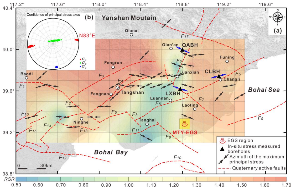
Figure 3. Crustal stress field in the Tangshan seismic region, as determined by inversion of 98 focal mechanisms shown in Fig.2 using STRESSINVERSE software package (Vavryčuk, 2014). (a) The results of the inversion in each bin ( 0.1^\circ \times 0.1^\circ ) include the predominant maximum principal compressive stress orientation ( \sigma_1 ) and the
