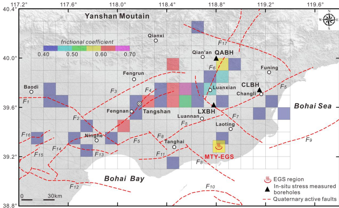
5 6 Figure 4. The critical coefficient of friction of the main seismic faults in the Tangshan seismic region, as 7 determined by inversion of 98 focal mechanisms (seen in Figure 2) using STRESSINVERSE software package 8 (Vavryčuk, 2014). 9
