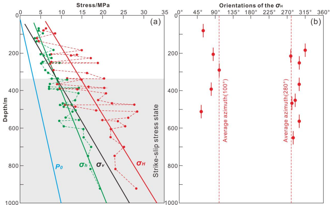
10 11 Figure 5. Hydraulic fracturing in situ stress results at shallow depths (< 1000 m) near the MTY EGS field in 12 Tangshan seismic region. (a) The magnitudes of three principal stresses with the depth. (b) The orientations of the 13 maximum horizontal principal stress ( \sigma_H ). 14
