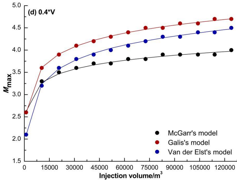
Figure 17. The maximum moment magnitude of injection-induced seismicity within ~10-15 km away from the injected wells in response to monthly time series of injection volume in MTY EGS field. In the calculation, the monthly injection volumes ( V ) are taken as 2.59 \times 10^3 \text{ m}^3 , 2.59 \times 10^4 \text{ m}^3 , 5.18 \times 10^4 \text{ m}^3 , 7.78 \times 10^4 \text{ m}^3 , 1.04 \times 10^5 \text{ m}^3 , 1.30 \times 10^5 \text{ m}^3 , 1.56 \times 10^5 \text{ m}^3 , 1.81 \times 10^5 \text{ m}^3 , 2.07 \times 10^5 \text{ m}^3 , 2.33 \times 10^5 \text{ m}^3 , 2.59 \times 10^5 \text{ m}^3 , 2.85 \times 10^5 \text{ m}^3 and 3.11 \times 10^5 \text{ m}^3 , respectively, corresponding to fluid injected rate of 1 L/s, 10 L/s, 20 L/s, 30 L/s, 40 L/s, 50 L/s, 60 L/s, 70 L/s, 80 L/s, 90 L/s, 100 L/s, 110 L/s and 120 L/s, respectively.
