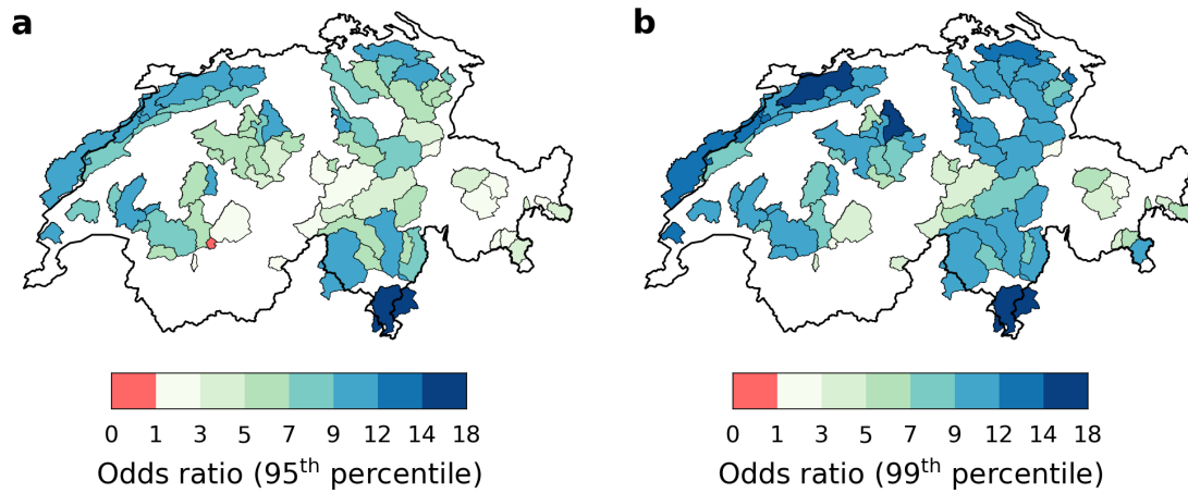
Figure 11. Odds ratio for extreme discharge occurrence (defined based on daily (a) 95 th and (b) 99 th discharge percentiles) during and up to 5 days after cluster events (see section 3.4 for methodological details).
