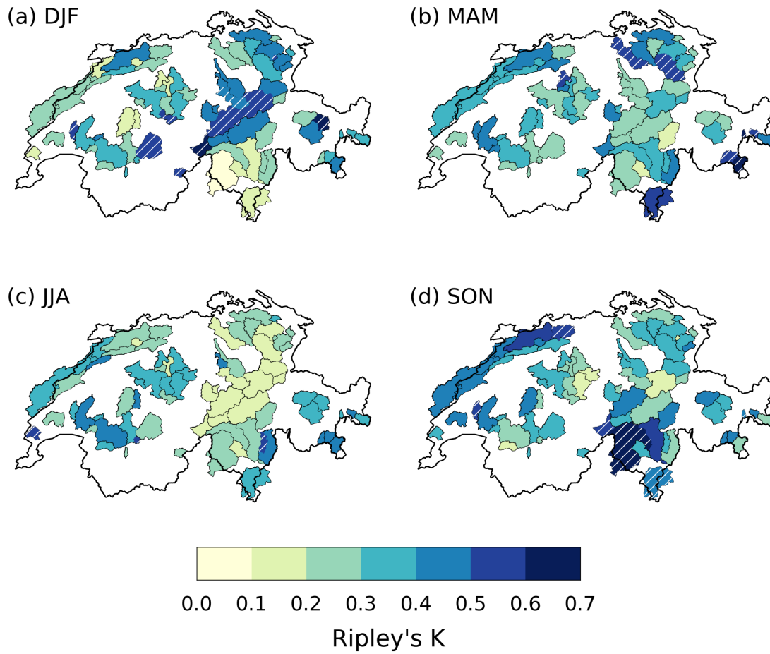
Figure A4. Value of Ripley's K in the RhiresD dataset for a 20-day window, in (a) DJF, (b) MAM, (c) JJA and (d) SON, for the 63-catchment partition. Compare with Figure 4.
