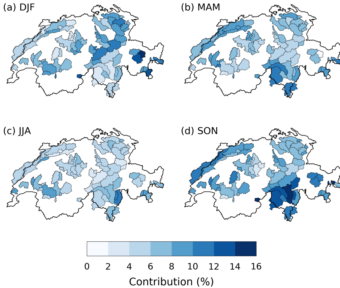
Figure A5. Contribution of 21-day extreme precipitation clusters to seasonal precipitation in RhiresD, in (a) DJF, (b) MAM, (c) JJA and (d) SON, for the 63-catchment partition. Compare with Figure 6.
