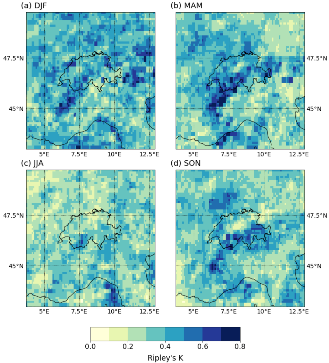
Figure A3. Average Ripley's K value for a 20-day window across ERA5, TRMM, CMORPH, CPC and EOBS in (a) DJF, (b) MAM, (c) JJA and (d) SON. For this comparison, all datasets were regridded to the smallest 0.1^\circ EOBS resolution.
