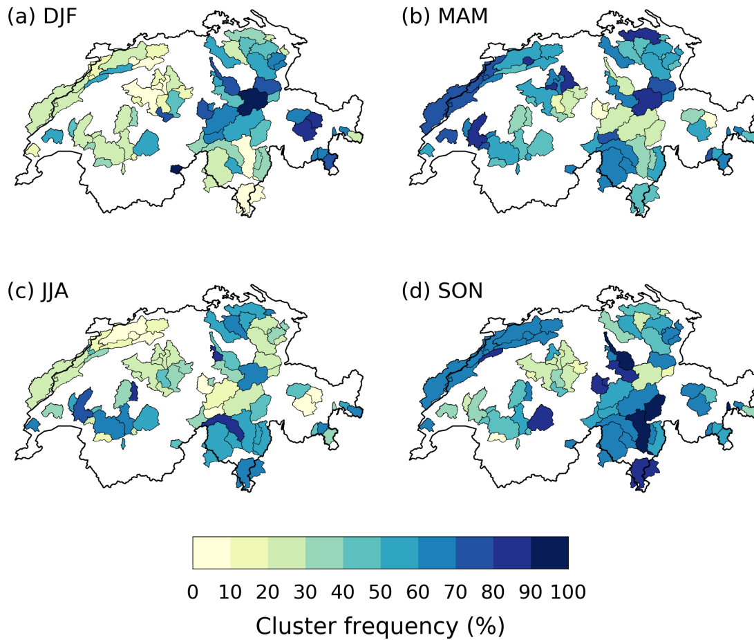
Figure A6. Frequency of extreme precipitation cluster occurrence during extreme 21-day cumulative precipitation events (> 99 th percentile) in RhiresD, in (a) DJF, (b) MAM, (c) JJA and (d) SON, for the 63-catchment partition. Compare with Figure 7.
