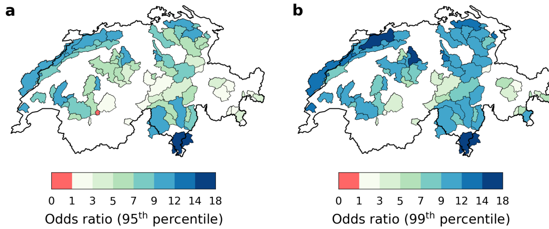
Figure 11. Odds ratio for extreme discharge occurrence (defined based on daily (a) 95 th and (b) 99 th discharge percentiles) during and up to 5 days after cluster events (see section 3.4 for methodological details ).
