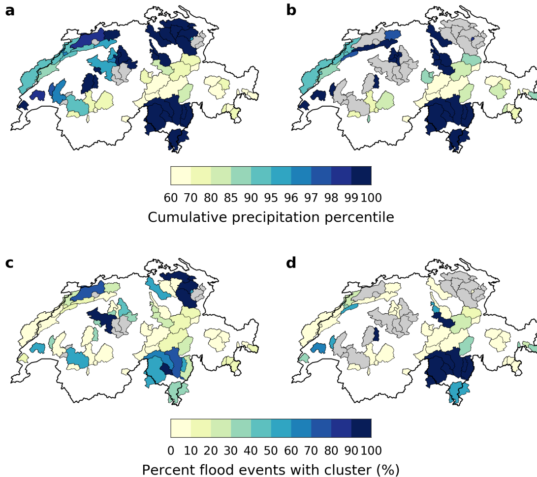
Figure 8. (a,b) Average cumulative precipitation percentile during and 10 days prior to persistent high-discharge periods , defined as: (a) at least 5 days within a 10-day window with discharge above its 99 th percentile, and (b) at least 8 days within a 20-day window with discharge above its 99 th percentile. Catchments for which such persistent high-discharge periods are not observed are shown in white. (c,d) Same as (a,b), but for the frequency of cluster occurrence during and 10 days prior to persistent high-discharge periods .
