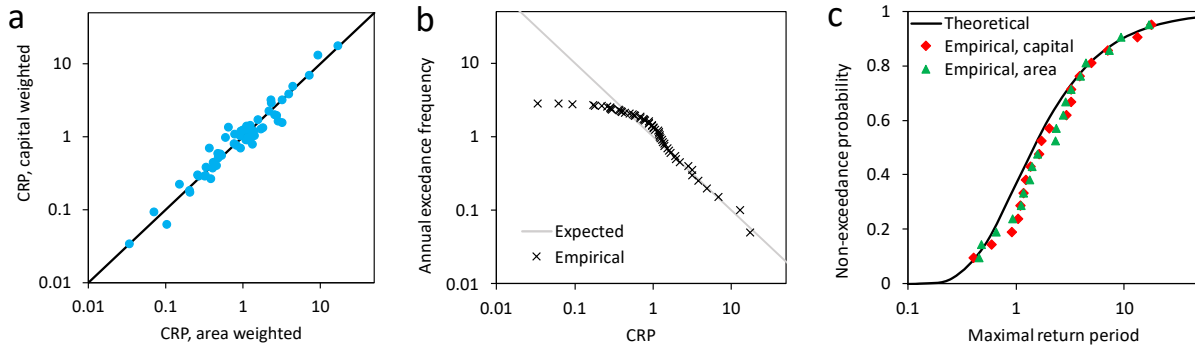
425 Figure 5: Results of the analysis: a) comparison of area and capital weighted CRPs, b) comparison of theoretical and observed exceedance frequency of capital weighted CRP, c) test of distribution of seasonal maxima of CRP.
