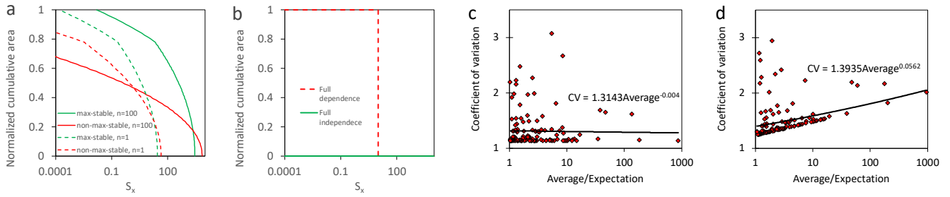
240 Figure 3: The area function and corresponding characteristics: a) area function of the biggest event of Figure 1, b) area functions for the limit cases (examples), c) relation CV to average for the max-stable case of Figure 1b, d) for the non-max-stable case of Figure 1d (events with average >1, the distance between the support points is 0.1 for the computation of the average in the region [-4,4]).
