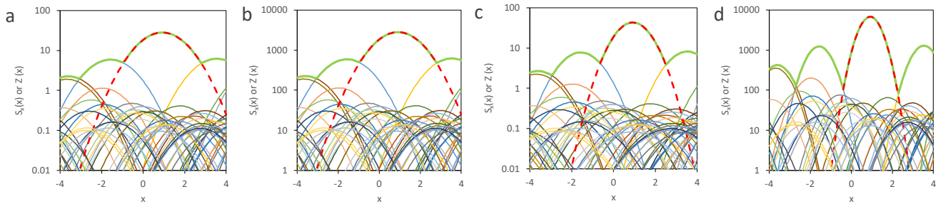
205 Figure 1: Examples of simulated fields of local event intensities and enveloping field of maxima (bold green line) generated with standard normal PDF as Y(x) in (6,7,9,10) and the same series of numbers from pseudo-random generator: a) max-stable and n=1 , b) max-stable and n=100 , c) non max-stable and n=1 , d) non max-stable and n=100 . The strongest event has a broken red line.
