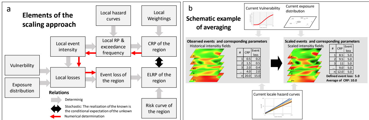
345 Figure 4: Schemes of the scaling approach: a) elements and relations, b) schematic example for estimation RP of event loss by averaging of CRP.
