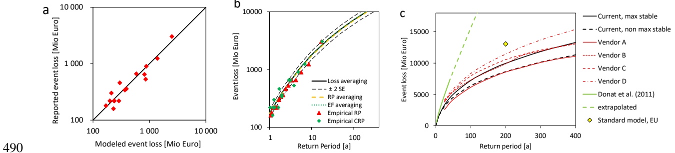
Figure 7: Estimates for insured losses from winter storms in Germany: a) reported versus modelled event losses, b) current risk curves and observations, c) influence max-stable and non-max-stable scaling and comparison to scaled, previous estimates (Donat et al., 2011; Waisman, 2015, European Commission, 2014).
