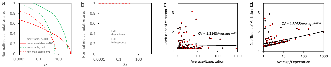
245 Figure 3: The area function and corresponding characteristics: a) area function of the biggest event of Figure 1, b) area functions for the limit cases (examples), c) relation CV to average for the max-stable case of Figure 1b, d) for the non-max-stable case of Figure 1d (events with average >1, the distance between the support points is 0.1 for the computation of the average in the region [-4,4]).
