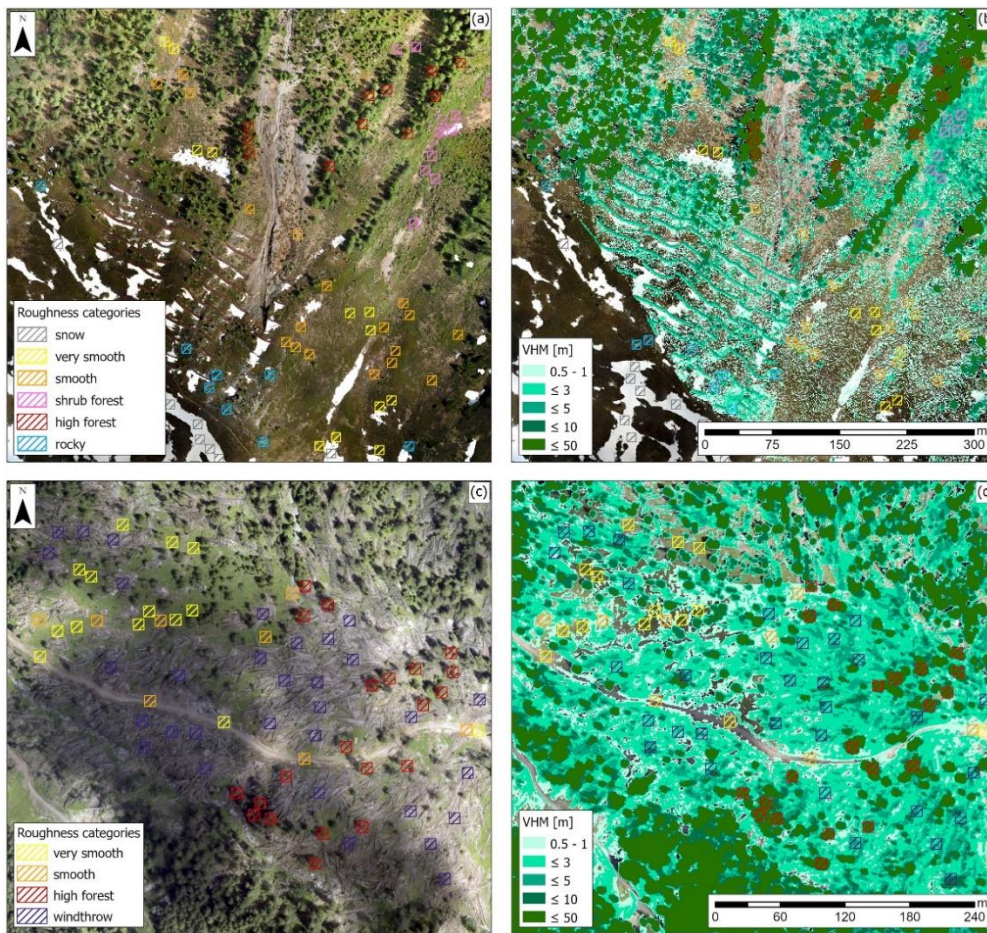
280 Figure 2: Roughness categories were selected based on the orthophoto alone (a) and (c) (drone flights, 2019) and with the vegetation height model (VHM, produced as the difference between the DSM and DTM provided by the Federal Office of Topography for Braema (©swisstopo, 2018) and Veneto region for Franza; (b) and (d)). The Braema study area (Grisons, Switzerland) is shown in (a) and (b), and the Franza study area (Veneto, Italy) is shown in (c) and (d).
