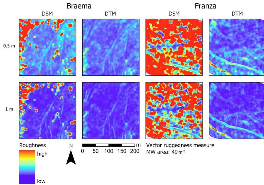
580 Figure A4: Calculated surface roughness in the two study areas Braema and Franza, using DSM and DTM (©swisstopo for Braema, region Veneto for Franza) and the vector ruggedness measure algorithm.
