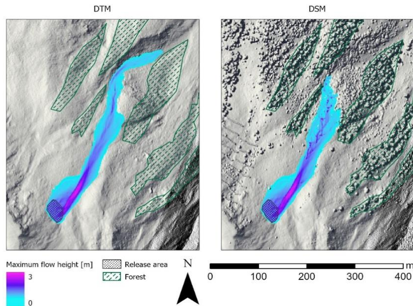
405 Figure 8: Avalanche simulation output (maximum flow height) in the Braema study area. The avalanche runout distance was 112 m greater when the DTM was used as the input model for the simulation than when the DSM was used (visualized are the hillshades calculated from the terrain and surface model swissALTI3D; ©swisstopo, 2018). The maximum flow height was 0.4 m greater when the DSM was used, as a result of the interaction with the roughness features.
