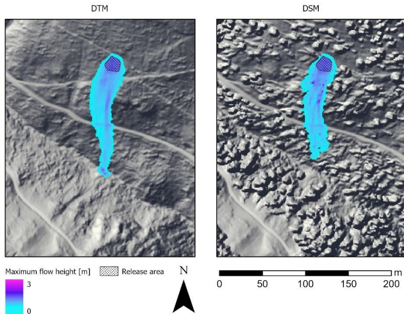
585 Figure A5: Avalanche simulation output (maximum flow height) in the Franza study area. The avalanche runout distance was 20 m longer when the DTM was used as the input model for the simulation than when the DSM was used (LiDAR data provided by the region Veneto). The maximum flow height was 0.2 m greater when the DSM was used, as a result of the interaction with the roughness features.
