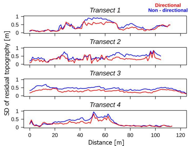
385 Figure 7: Analysis of the four transects from the Braema study area using the SD of residual topography algorithm (red) or without (blue) direction in the calculation.
