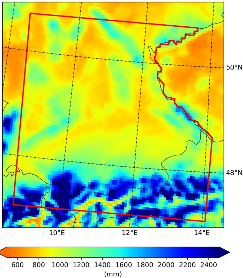
Figure 2: Annual mean precipitation for the period 1980–2009 from the RCM setup of Warscher et al. (2019).
