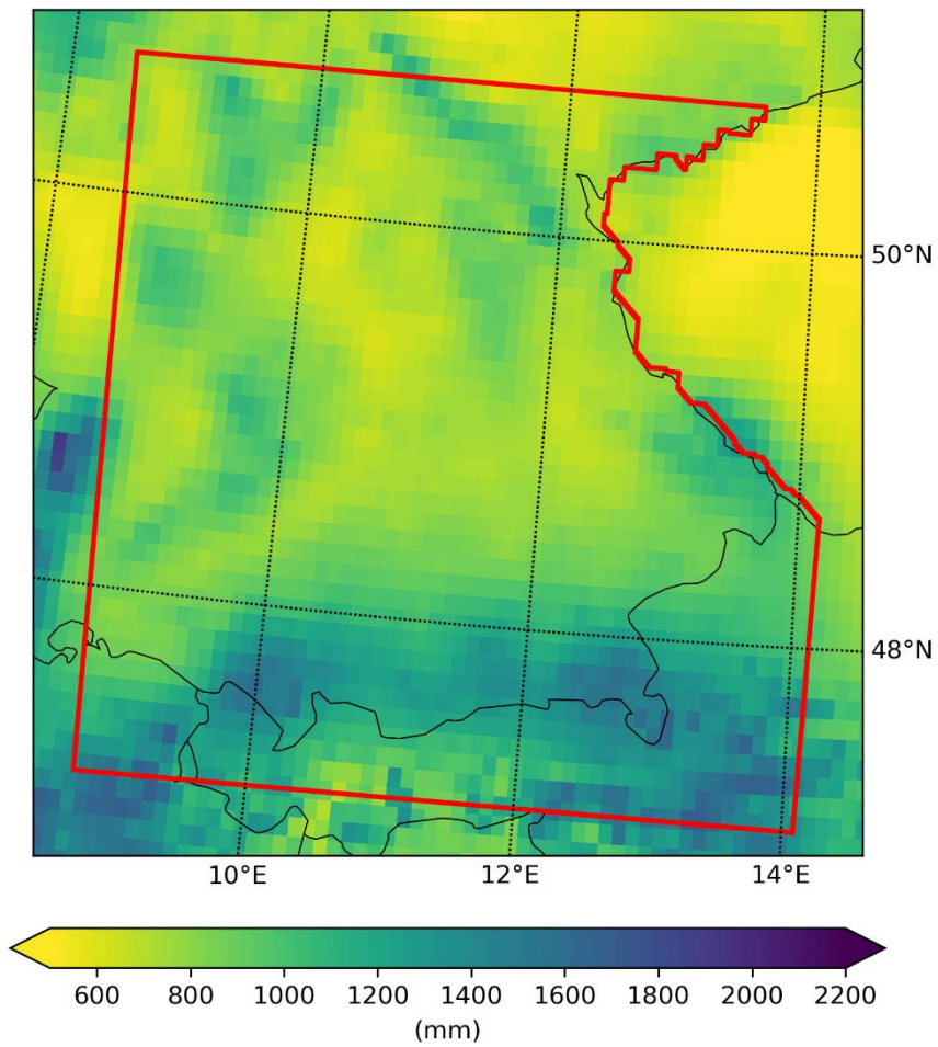
Figure 2: Annual mean precipitation for the period 1980 – 2009 from the RCM setup of Warscher et al. (2019) based on E-OBS (Haylock et al., 2008).
