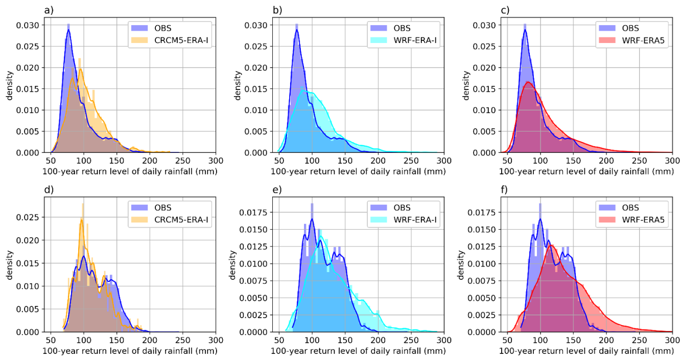
540 Figure 8: Histograms of the resulting 100-year return levels in the whole study area (a-c) and the alpine area south of 48° N (d-f). Gaussian kernel density estimates are plotted to enhance the readability.
