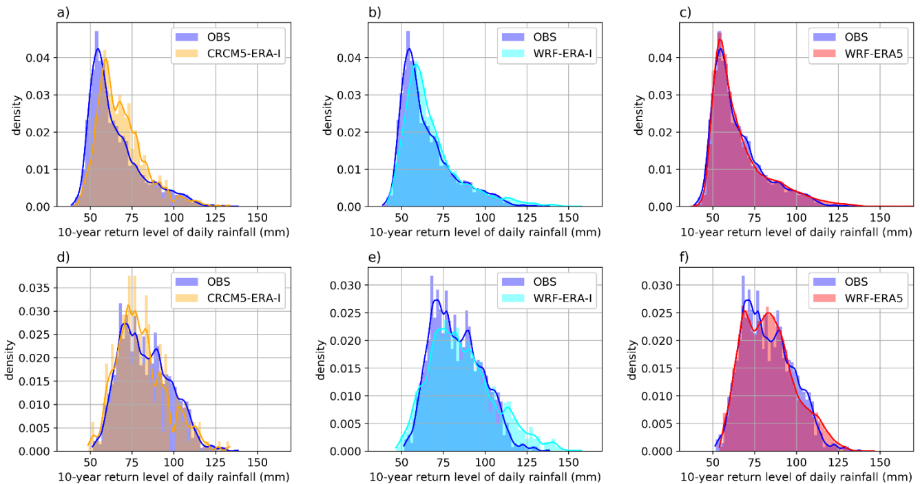
465 Figure 5: Histograms of the resulting 10-year return levels in the whole study area (a-c) and the alpine area south of 48^\circ\text{ N} (d-f). Gaussian kernel density estimates are plotted to enhance the readability.
