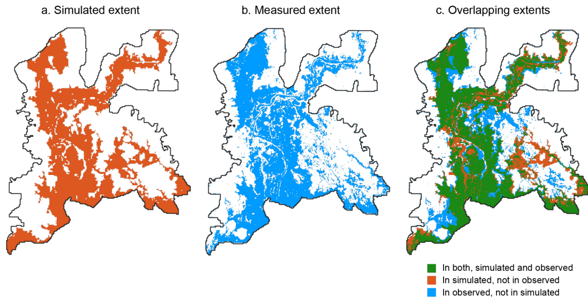
Fig. 3. Comparison of maximum flood extent resulting from the model and measured from satellite images.
