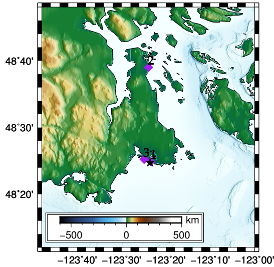
Figure 4. The location that drives the design algorithm is indicated with a black star (lon:-123.3934, lat:48.4127). The locations of three emulators (1- lon:-123.3904, lat:48.4149; 2- lon:-123.3989; lat: 48.6657; 3- lon:-123.415478, lat:48.420584) at the cell centres of the grid are displayed with purple diamonds.
