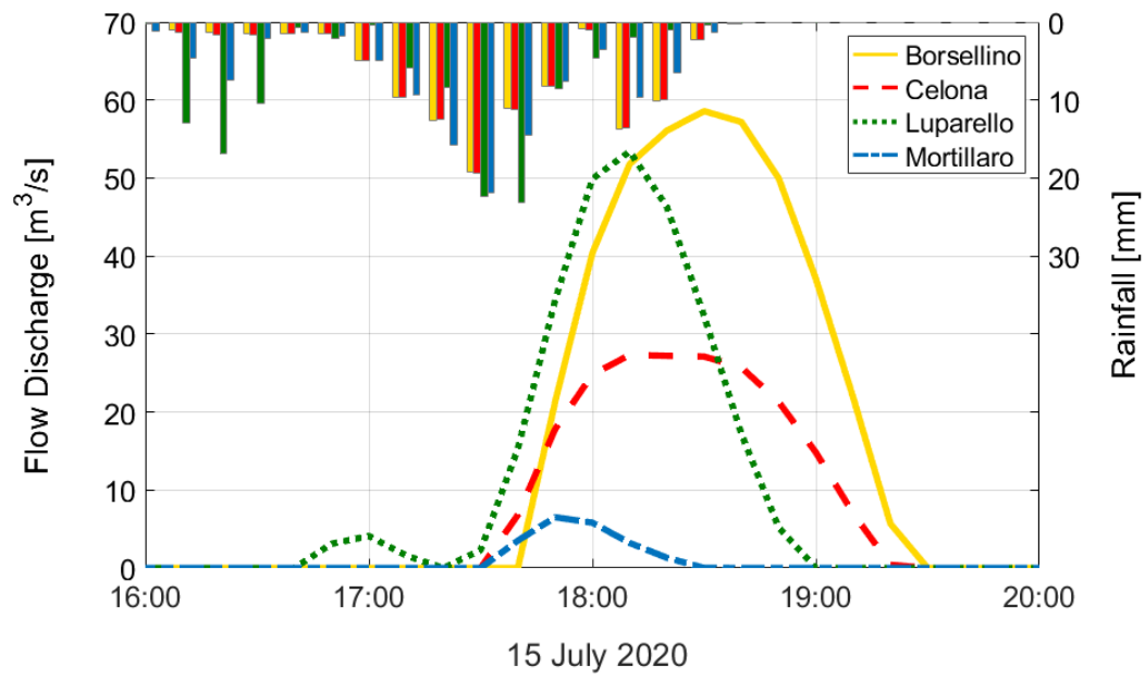
Figure 9. Rainfall Discharge obtained from the hydrological simulations in TOPDM. The bars in the upper part of the figure indicate the IDW interpolated precipitation over the four basins.
