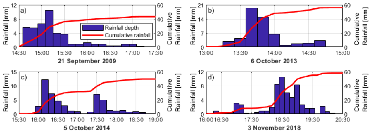
685 Figure 5. Rainfall collected at the rain gauge Uditore for the events occurred on a) 21 September 2009, b) 6 October 2013, c) 5 October 2014, and d) 3 November 2018.
