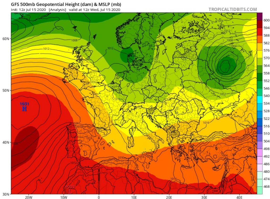
690 Figure 6. Geopotential heights at the 500mb level (12Z GFS) and mean sea level pressure (MSLP). Coloured scale bar indicates the geopotential height values in dam (i.e., decametre), while contour black lines indicate MSLP in mb (i.e., millibar). Source image: NCEP of the NOAA.
