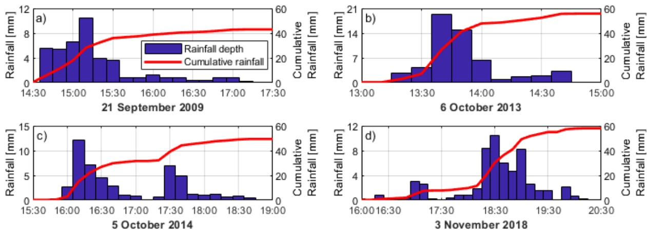
685 Figure 5. Rainfall collected at the rain gauge Uditors for the events occurred on a) 21 September 2009, b) 6 October 2013, c) 5 October 2014, and d) 3 November 2018.
