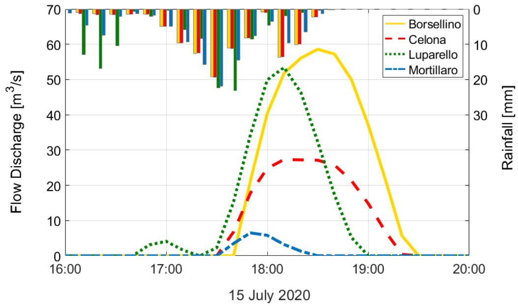
705 Figure 9. Rainfall Discharge obtained from the hydrological simulations in TOPDM. The bars in the upper part of the figure indicate the IDW interpolated precipitation over the four basins.
