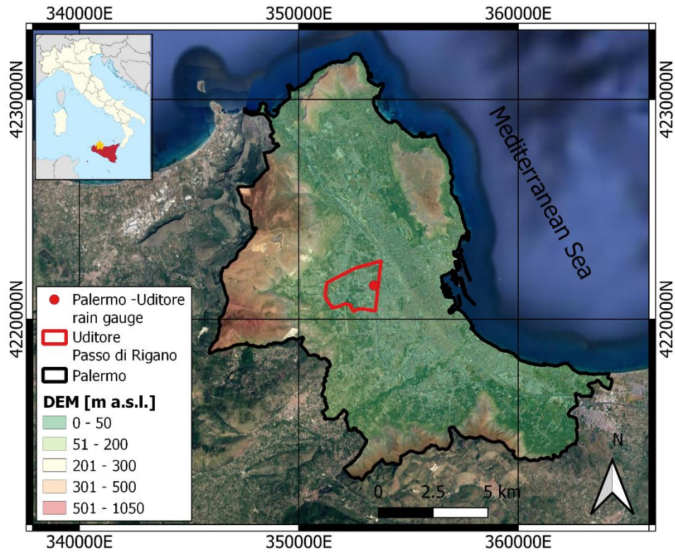
655 Figure 1. 20 meters resolution Digital Elevation Model of Palermo (Sicily, Italy) with location of the Uditore - Passo di Rigano district (red line) and the Uditore rain gauge station (red point) of the SIAS rain gauges' network. The yellow star in the inset indicates the location of Palermo. Source aerial: © Google Maps Satellite basemap available within the QuickMapServices plugin of Quantum GIS.
