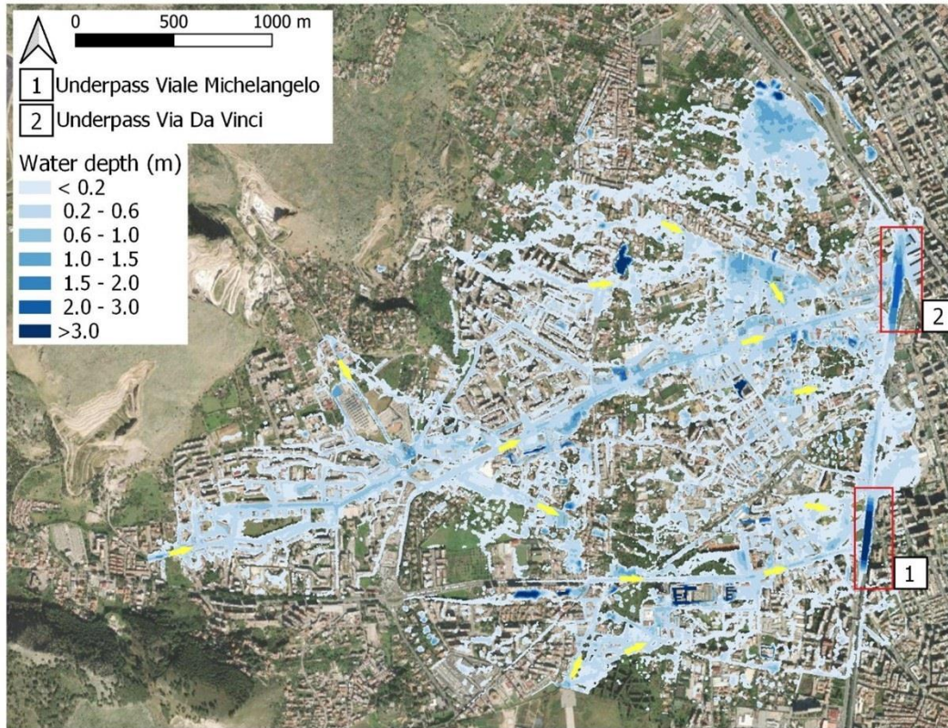
715 Figure 11. Map of the maximum flood depths reached on 15 July 2020 for the district Uditore - Passo di Rigano as simulated in WEC-FLOOD. The yellow arrows indicate the flow directions of the flood. Source aerial: © Google Maps Satellite basemap available within the QuickMapServices plugin of Quantum GIS.
