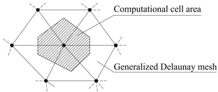
700 Figure 8. Computational mesh of WEC-FLOOD model. The vertices of each cell (black dots) are the computational centers of the cells (i.e., the point where the water surface is computed for the cell) and are obtained as the circumcenters of the generalized Delaunay triangulation.
