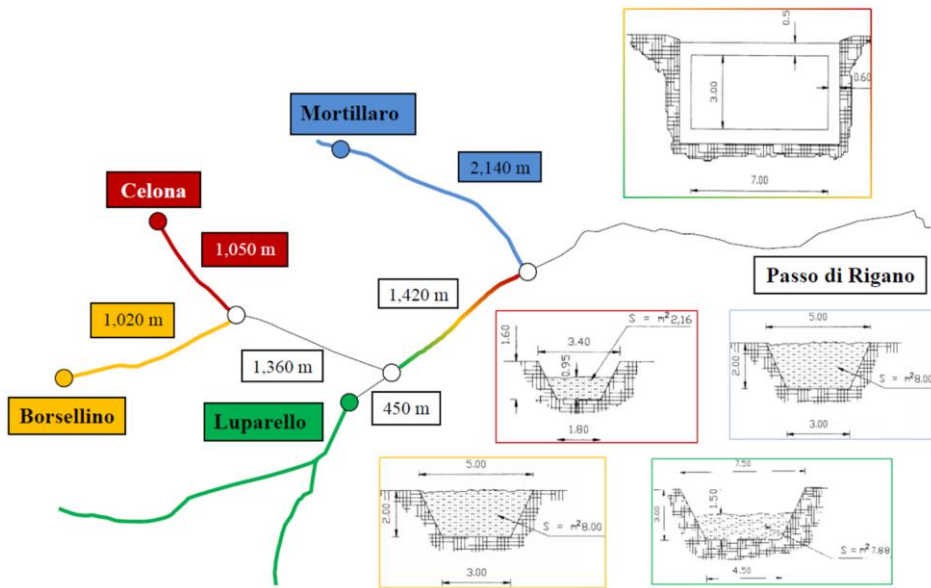
Figure 2. Passo di Rigano drainage system for the conveying and regulation of rainwater in the study area. Yellow color is associated with Borsellino, the red with Celona, the green with Luparello, and the blue with Mortillaro channels; the box within mixed colors (red, yellow, and green) refers to the section of the Luparello channel downstream the confluence with the Borsellino and Celona channels.
