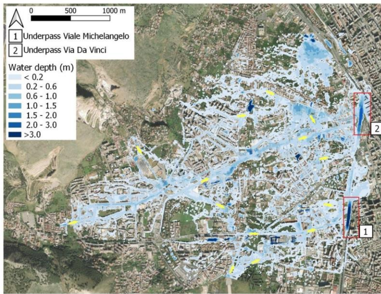
Figure 11. Map of the maximum flood depths reached on 15 July 15 , 2020 for the district Uditore - Passo di Rigano as simulated in WEC-FLOOD. The yellow arrows indicate the flow directions of the flood. Source aerial: © Google Maps Satellite basemap available within the QuickMapServices plugin of Quantum GIS.
