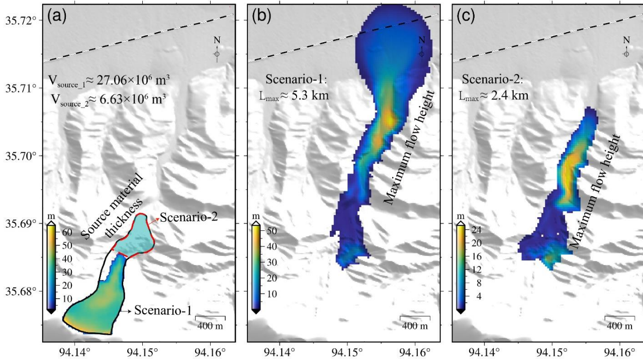
Figure 10: Runout estimates for the detachments of the whole glacier (scenario-1) and glacier tongue (scenario-2). (a) Ice (i.e., source material) thickness distribution of the avalanche scenarios-1 (black polygon) and scenario-2 (red polygon) derived from the global glacier ice thickness products of Farinotti et al. (2019). (b) The simulated maximum flow height of the avalanche for scenario-1 when choosing moderate friction values of 0.15 for Coulomb friction ( \mu ) and 2500 m·s -2 for turbulent friction ( \xi ) in the Voellmy-Salm model. (c) The simulated results for scenario-2.
