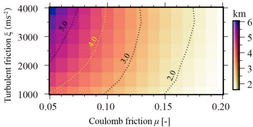
Figure 12: Variations of runout distance for varying friction parameters ( \mu and \xi ) of the Voellmy-Salm model. The dotted lines represent the contour lines with the yellow one representing the runout distance (4 km) that will threaten the Qinghai-Tibet railway.
