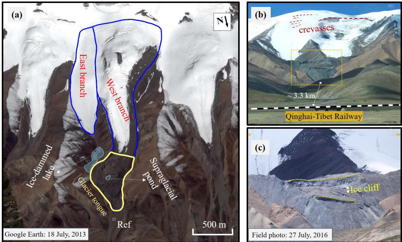
120 Figure 2: (a) The outlines of the KLP-37 glacier (blue line) and tongue (yellow line) overlaid on a Google Earth image of 18 July 2013 (© Google Earth™). The ice-dammed glacier lake and a supraglacial pond are also shown. (b) and (c) are the field photos acquired by the author on 27 July 2016, which exhibit the crevasses and ice cliffs on the glacier surface. The rectangle annotated with “Ref” in (a) indicates the area for estimating image cross-correlation error (see Section 3.3).
