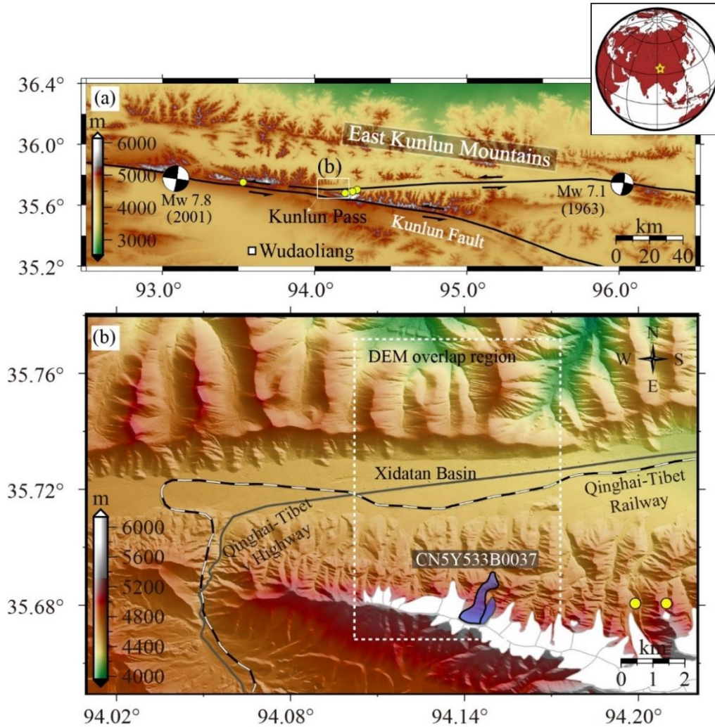
Figure 1: (a) The tectonic overview of the study area. The black lines depict the Kunlun fault traces. The yellow dots mark the ice avalanche locations induced by the 2001 Mw 7.8 earthquake (Jerome et al., 2004). The white square indicates the Wudaoliang Meteorological station. (b) The topography of the Kunlun Pass region. The white rectangle shows the overlap region of the DEMs used in this study. The polygons are the glaciers from the GAMDAM glacier inventory (Sakai et al., 2019), while the one filled with purple color is the KLP-37 glacier, whose west branch is outlined in thick black.
