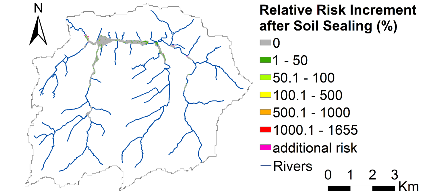
Figure 11: Relative flood risk increment (%) in the flooded areas in the Maarkebeek catchment after sealing the 750 highest ranked pixels in this land use change scenario. New areas being flooded after soil sealing are depicted as 'additional risk'.
