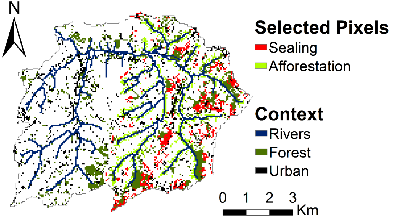
255 Figure 5: Locations of the pixels selected for land use change implementation, i.e. the 750 priority pixels (187.5 ha), for both the afforestation and soil sealing scenarios.
