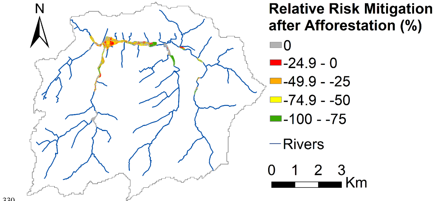
Figure 10: Relative flood risk mitigation (%) in the Maarkebeek catchment after afforesting the 750 highest ranked pixels in this land use change scenario.
