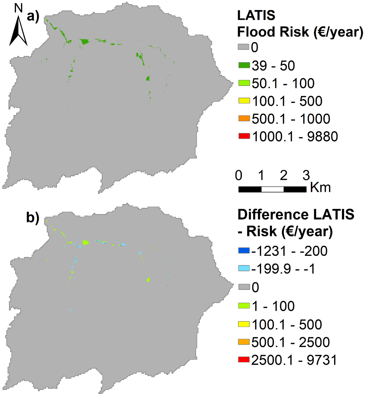
Figure 12: (a) Flood risk (€/year per pixel of 25 m 2 ) in the Maarkebeek catchment as calculated by the LATIS tool based on the flood damages determined for flood events with a return period of 10, 100 and 1000 years (adapted from (VMM, 2015)). (source: VMM et al., 2020); (b) Difference in flood risk (€/year per pixel of 25 m 2 ) between the flood risk determined by the LATIS tool and as calculated based on the four observed flood events in the Maarkebeek catchment.
