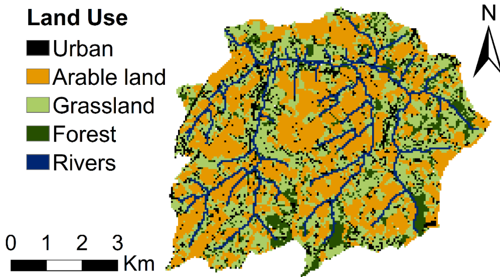
190 Figure 3: General land use in the Maarkebeek catchment, based on the land use dataset of 2012 (AGIV, 2016).
