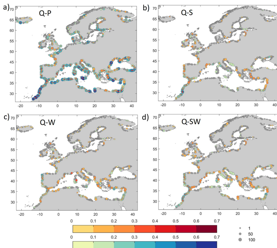
440 Figure 7: Kendall's correlation coefficients ( p < 0.05 ) between multivariate extremes selected using the POT3 approach and the joint occurrences between (a) Q-P, (b) Q-S, (c) Q-W and (d) Q-SW. Correlations between compound events selected when variable 1 is the dominant driver is represented on the red scale while the blue scale denotes the correlations obtained when variable 2 is the dominant driver. The size of the circles on blue scale represents the joint occurrences (maximum=100). If correlation is insignificant when variable 2 is the conditioning variable, the size of the circle on red scale represents the joint occurrences. When both correlation coefficients are insignificant, the size of the grey circle represents the joint occurrences.
