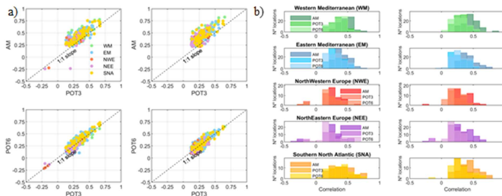
315 Figure 2: a) Scatter plots of the Kendall's correlation ( p < 0.05 ) between Q and P using POT3 vs AM (upper panels) and POT3 vs POT6 (lower panels), using either Q (left panels), or P (right panels) as the dominant variable. b) Histograms of the correlation coefficients using the three approaches (AM, POT3 and POT6) for each region when either Q (left panels) or P (right panels) as the dominant drivers.
