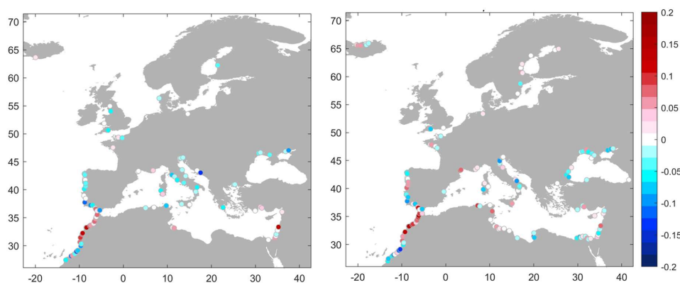
390 Figure 6: Differences in the Kendall's correlation coefficient ( p < 0.05 ) obtained when using Q and SW and Q and WL (left panel) and P and SW and P and WL (right panel) when SW or WL are the dominant variables.
