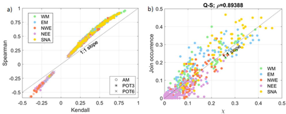
Figure 5: a) Scatter plot of the Kendall's correlation coefficient ( p < 0.05 ) vs Spearman's correlation coefficient ( p < 0.05 ) between all pairs of variables. b) Scatter plot of the statistic \chi (threshold = 0.95) against the joint occurrence divided by 3 events per year for the pair of variables Q-S.
