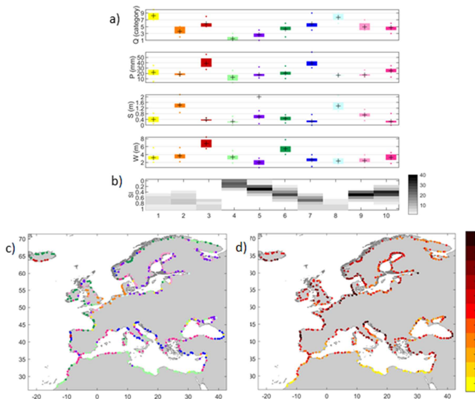
475 Figure 8: a) Ten clusters defined by the combination of the thresholds of four drivers (Q, P, S, W) used in the conditional sampling (the same colour is used to represent the four thresholds by the mean, 25th, 75th, 5th and 95th within each cluster). b) Probability of occurrence of each cluster for each severity index (SI) score (grey scale shows the number of locations represented by each cluster). c) Spatial distribution of the clusters represented in the same colour as used in panel a. d) Spatial distribution of SI based on the sum of the normalized thresholds of the four drivers.
