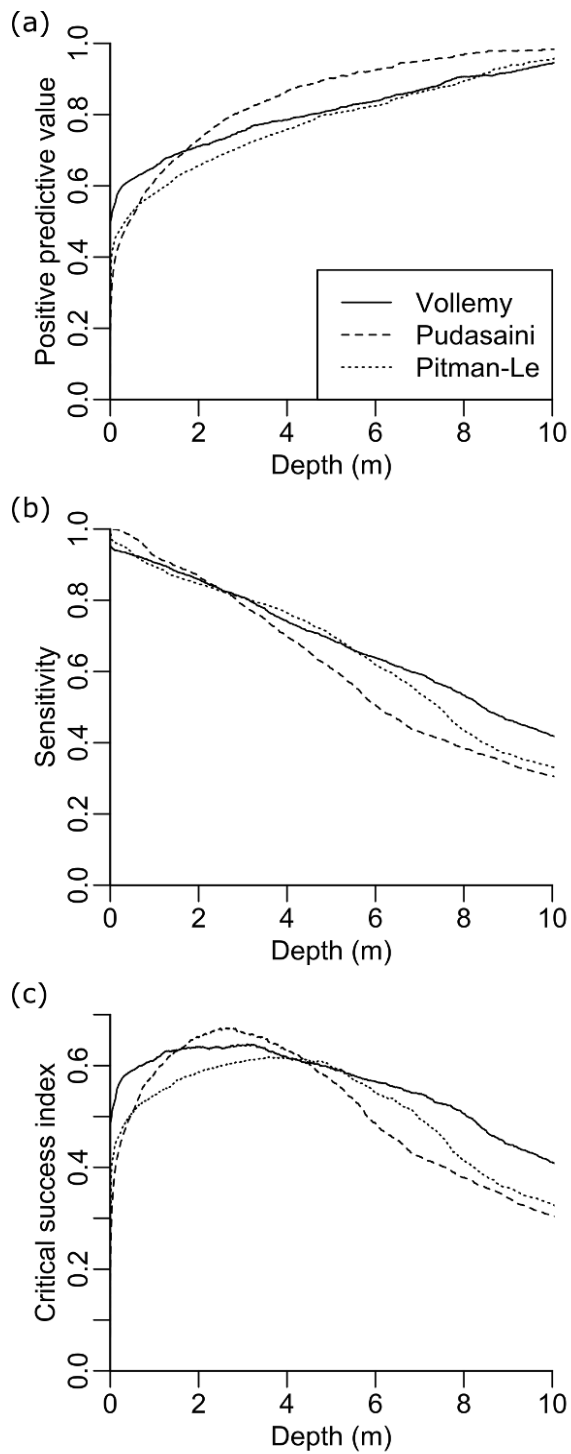
580 Figure 5. Flow outline performance with depth for Voellmy-Salm (solid line), Pudasaini (2012) (dashed line) and Pitman and Le (2005) (dotted line) flow models. Performance metrics are: (a) positive predictive value (PPV), (b) Sensitivity, and (c) Critical success index (CSI).
