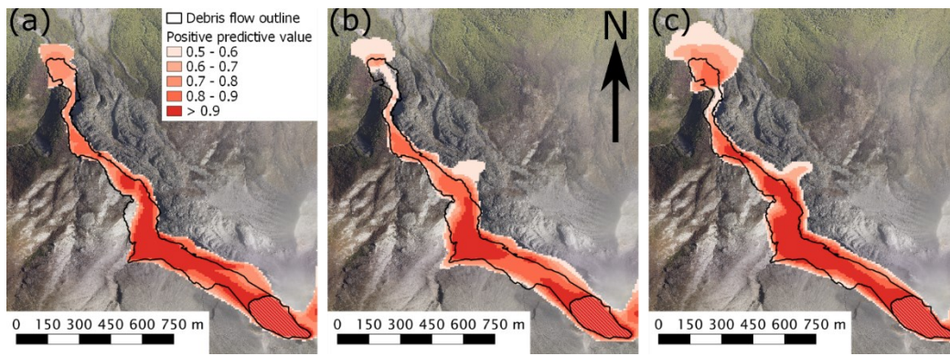
585 Figure 6. Positive predictive values for (a) Voellmy-Salm, (b) Pitman and Le (2005), and (c) Pudasaini (2012) simulations. The observed flow and source are outlined in black. Aerial basemap sourced from LINZ Waikato Aerial Photos (2012-2013).
