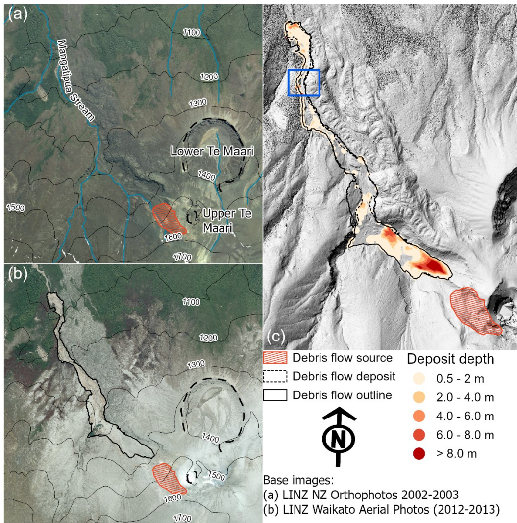
565 Figure 1. Te Maari debris avalanche case study region (a) pre-eruption, (b) post-eruption, and (c) debris avalanche deposit depth and outline. Blue rectangle in (c) shows area of spurious elevations from source Digital Terrain Model.
