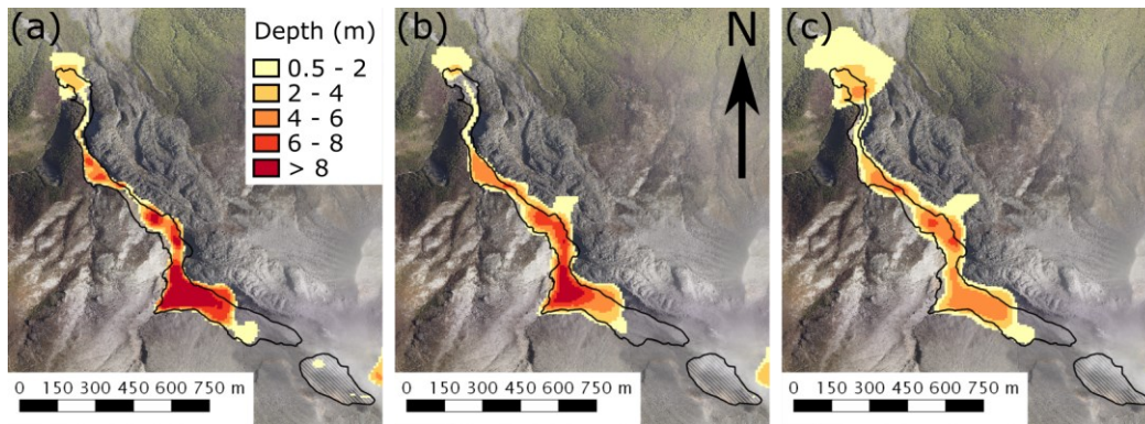
570 Figure 3. Simulated deposit depth for (a) Voellmy-Salm, (b) Pitman and Le (2005), and (c) Pudasaini (2012) models compared with the observed deposit and source outline (black). Aerial basemap sourced from LINZ Waikato Aerial Photos (2012-2013).
