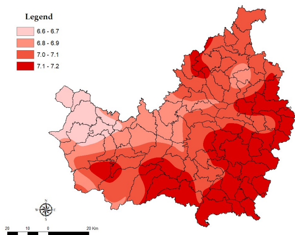
Fig. SM_7. Mean duration of a heat wave event (days)
