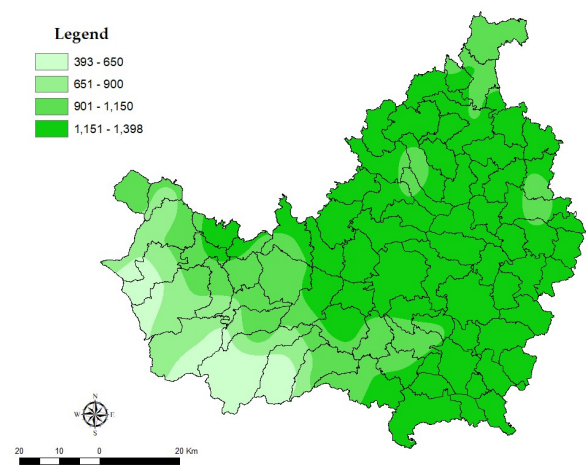
Fig. SM_12. Growing degree days ( ^{\circ}\text{C} )
