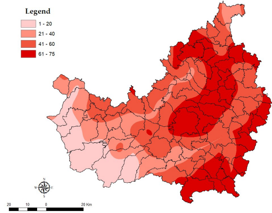
Fig. SM_2. Mean annual number of summer days
