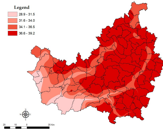
Fig. SM_1. Historical maximum temperature (°C)
