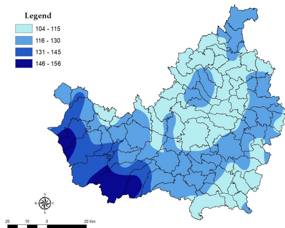
Fig. SM_9. Mean annual number of frost days
