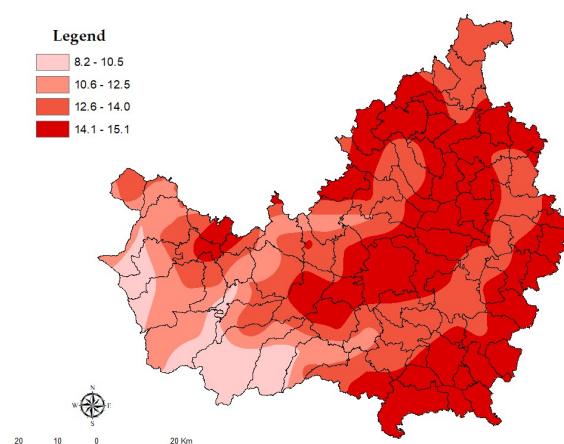
Fig. SM_6. Mean value of daily maximum temperature (°C)
