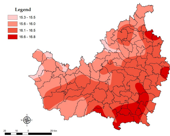
Fig. SM_8. Mean annual frequency (cumulative duration) of heat waves (days)
