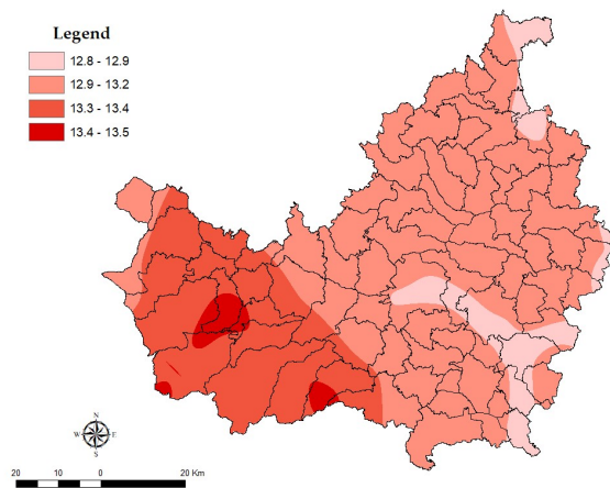
Fig. SM_5. Percentage of very hot days
