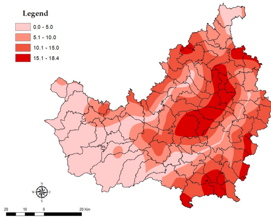
Fig. SM_3. Mean annual number of tropical days
