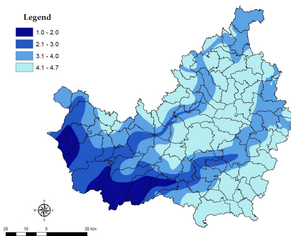
Fig. SM_11. Mean annual value of daily minimum temperature ( ^{\circ}\text{C} )
