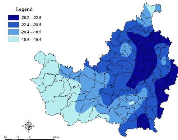
Fig. SM_10. Intensity of a cold wave event
