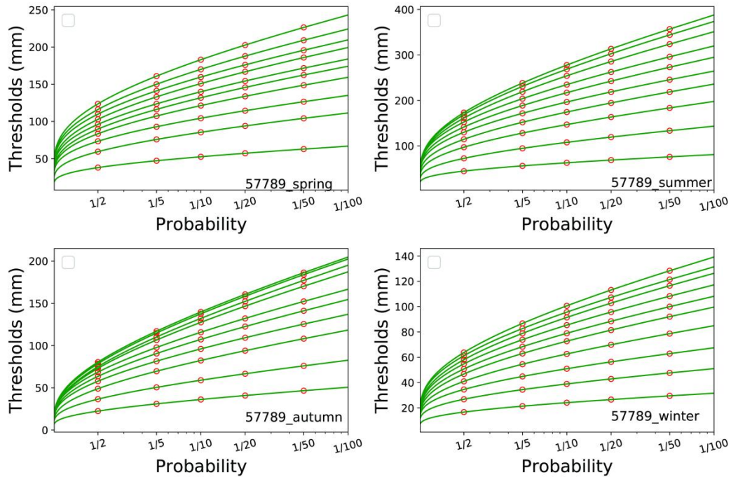
Figure 4 An example of extreme precipitation threshold distribution from the gamma fits of 1-10 run 12-H data in seasons. The green lines from bottom to up show the gamma fits of 1-10 runs respectively. The orange hollow points are thresholds calculated with a probability of 0.5 (1/2), 0.2 (1/5), 0.1 (1/10), 0.05 (1/20) and 0.02 (1/50).
