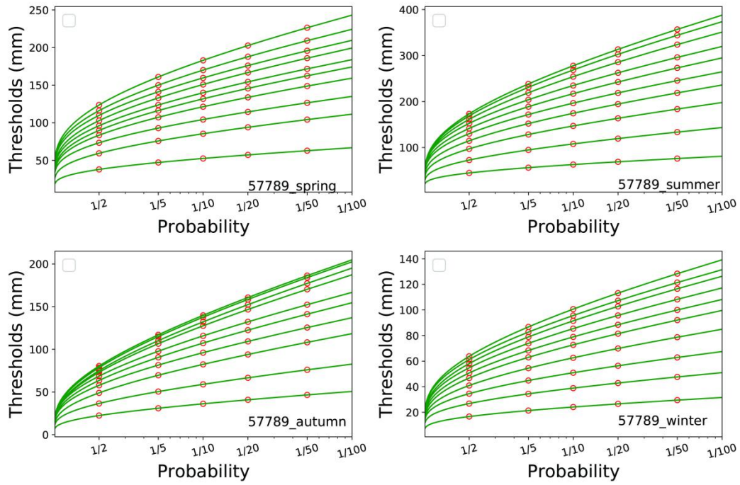
610 Figure 4 An example of extreme precipitation threshold distribution from the gamma fits of 1-10 run 12-H data in seasons. The green lines from bottom to up show the gamma fits of 1-10 runs respectively. The orange hollow points are thresholds calculated with a probability of 0.5 (1/2), 0.2 (1/5), 0.1 (1/10), 0.05 (1/20) and 0.02 (1/50).
